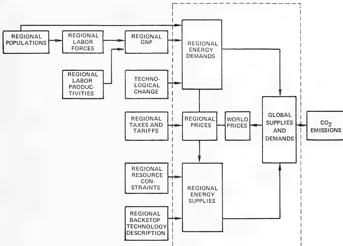
FIGURE B-3 SUMMARY OF INFORMATION FLOWS AND PROCEDURES IN THE IEA MODEL TO BALANCE ENERGY SUPPLIES AND DEMANDS
