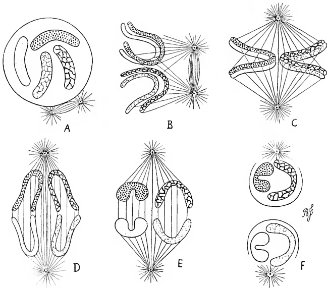
FIG. 4.—DIAGRAM OF MEIOSIS OR REDUCING DIVISION OF A NUCLEUS WITH FOUR CHROMOSOMES. (ORIGINAL.)
