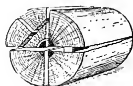
Shows manner of splitting section for timber of large diameter into stave bolts. In making staves, as well as heading bolts, for oil and other tight work, it is ever and always necessary to keep with the grain of wood.
