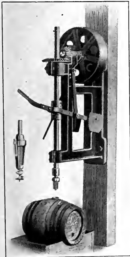
A BUNG BORING MACHINE
