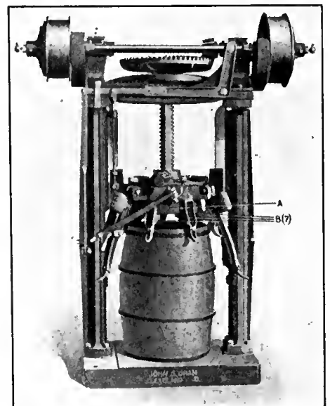
A BARREL TRUSSER AT WORK
