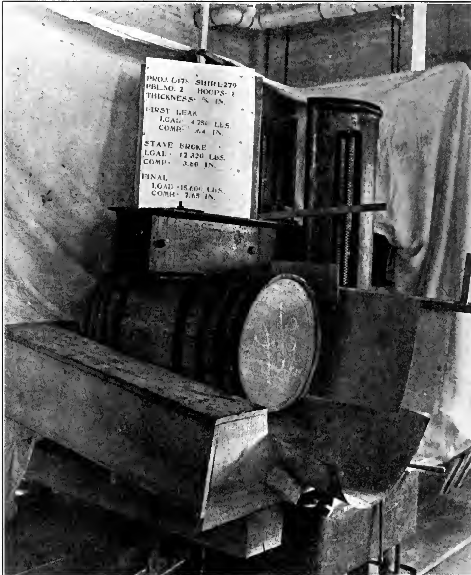
GAUGING PRESSURE ON THE BARREL'S SIDE
