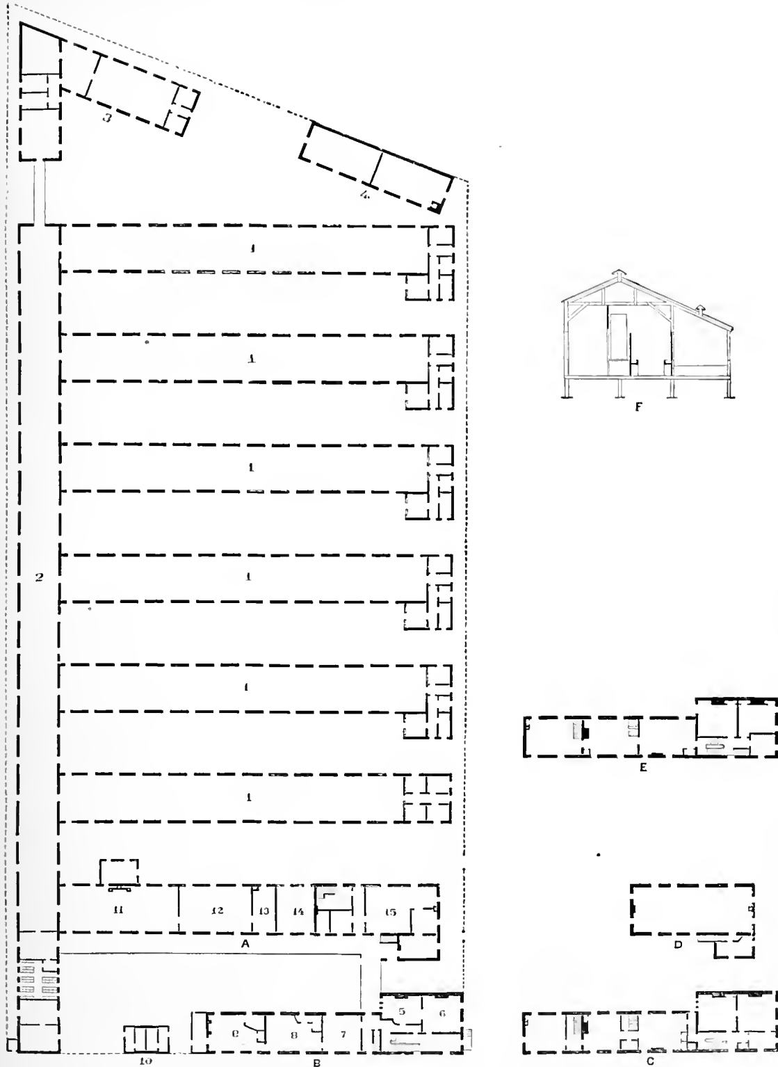
TILDEN HOSPITAL, WILMINGTON, DEL.—1, Wards; 2, Corridor; 3, Barracks, containing officers' rooms, guard-room, prison, smoking-room, water-closet and bath-room; 4, Tank-house; 5, General office; 6, Surgeon in charge; 7, officer of the day; 8, Officers' mess; 9, Kitchen and coal-house; 10, Water-closets; 11, Kitchen and coal-house; 12, Wash- and ironing-room; 13, Drying-room; 14, Store-room; 15, Steward's store-room, sleeping, office and bath-room. A, B, Ground floor of administration building. C, Second story of A, containing rooms of surgeon in charge, ladies' contributing-room, bath and water-closet. D, Ward in second story of B. E, Third story of B, containing dormitories of officers, etc. F, Transverse section through wardmaster's room, wash-room and water-closets. Picket-fence marked -----.
