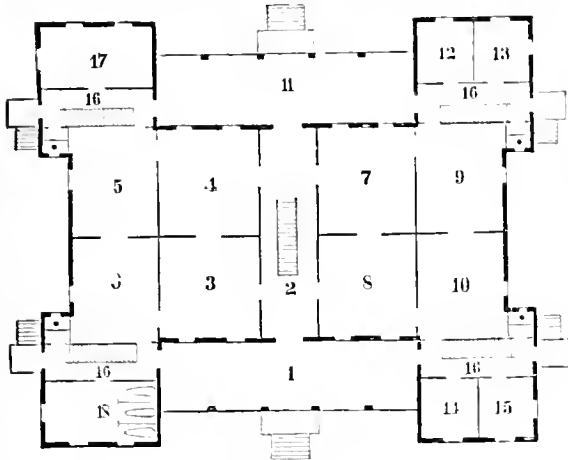
PLAN OF FLOOR— \frac{1}{8} "
