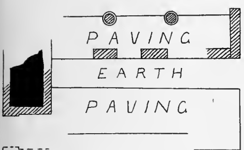
BUILDING OF SHABAKA IN S-W OF PTAH TEMENOS 1:200
