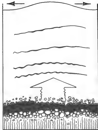
LONG-PERIOD EARTHQUAKE WAVES
