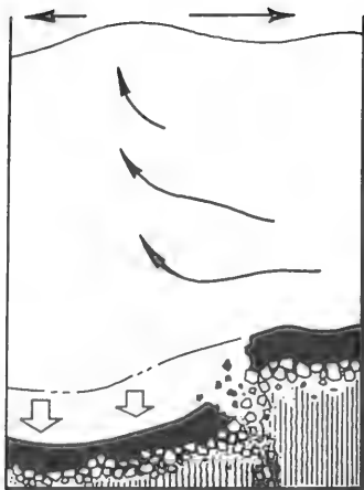
VERTICAL DISPLACEMENT OF SUBMARINE FLOOR
