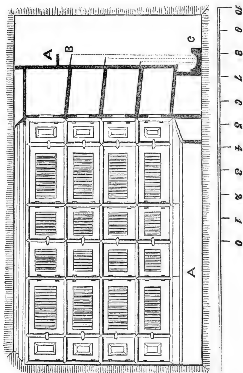
Nos. V. AND VI.—FRONT AND FLOOR SECTIONS.
