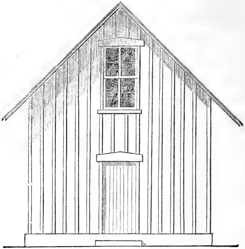
No. I.—GABLE END ELEVATION.
