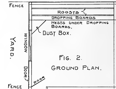
DESIGN FOR AN INEXPENSIVE CITY POULTRY HOUSE
