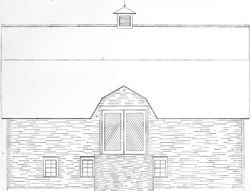
SIDE ELEVATION OF BARN BARN
