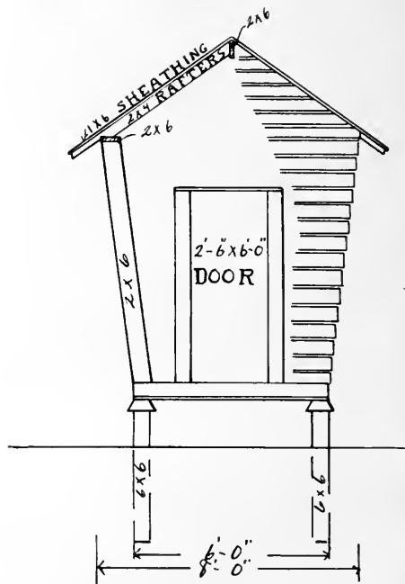
CROSS SECTION OF CORN CRIB
