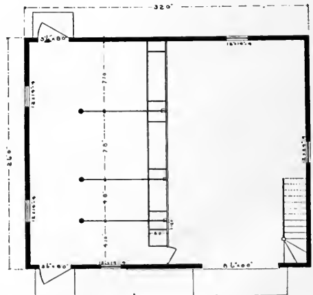
FLOOR PLAN
