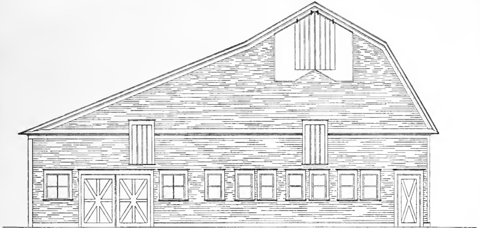
SIDE ELEVATION OF BARN AND YARD
