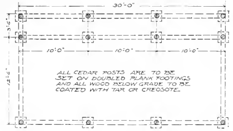
FOUNDATION PLAN
