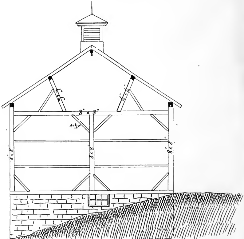
FRAMING AT END
