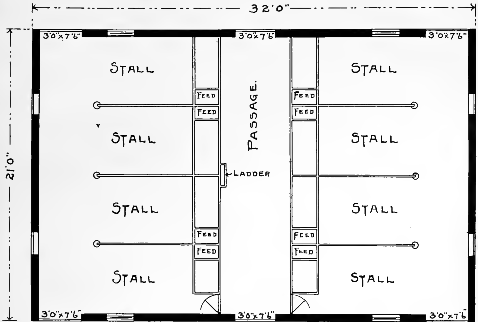
FLOOR PLAN.
