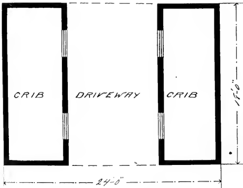
PLAN OF CORN CRIB.
