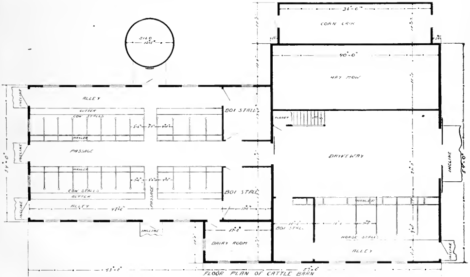
FLOOR PLAN OF CATTLE BARN
