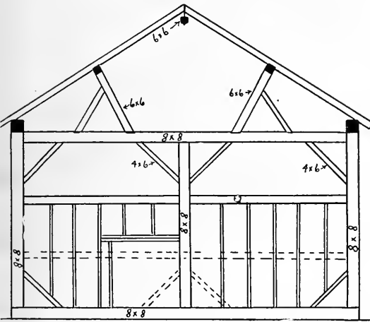
TRANSVERSE SECTION
