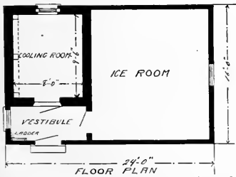
PLANS OF ICE HOUSE
