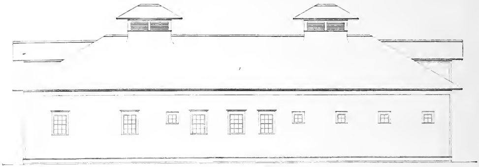
FIGURE 1. ELEVATION OF HORSE BARN
