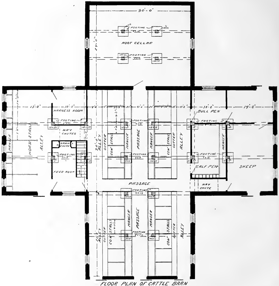
FLOOR PLAN OF CATTLE BARN
