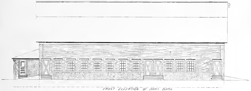
FRONT ELEVATION OF DAIRY BARN
