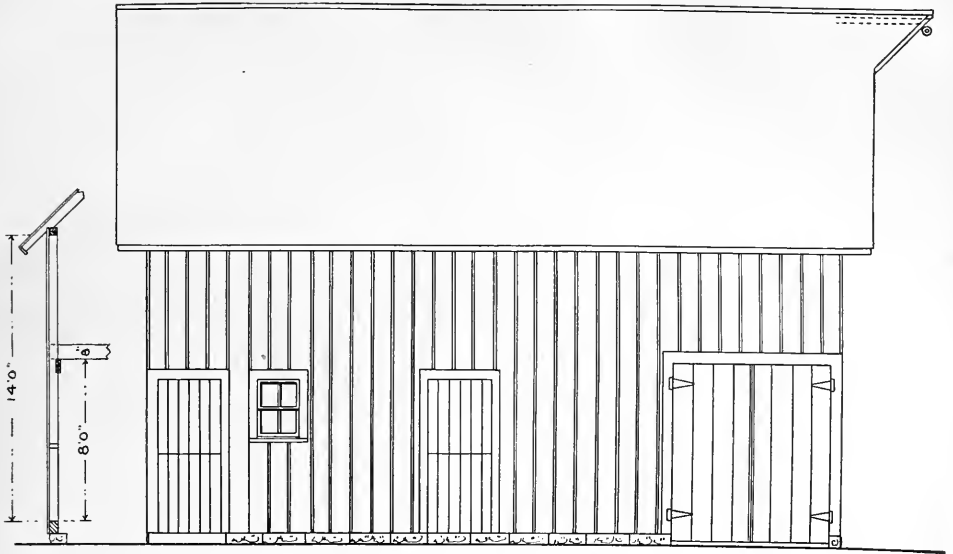
FRONT ELEVATION.
