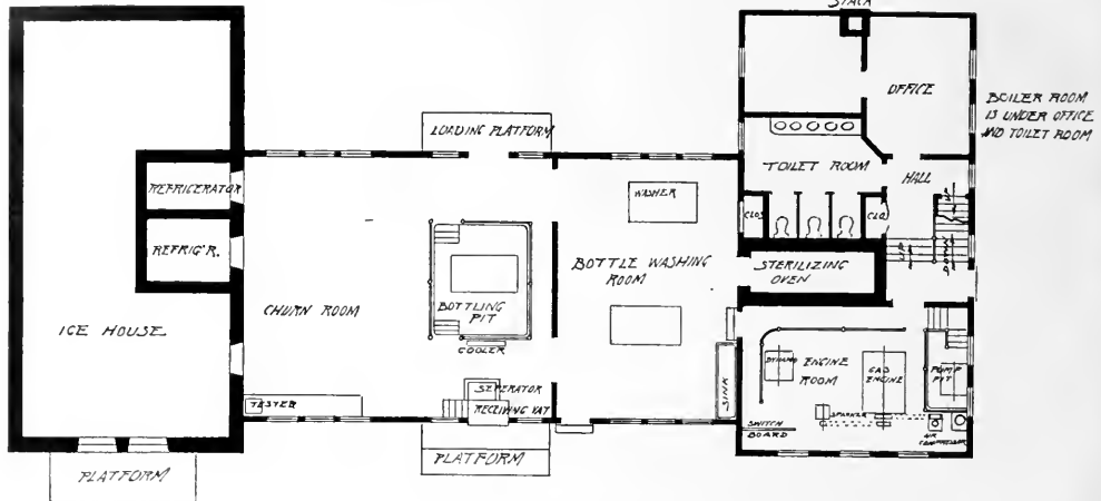
GROUND FLOOR PLAN OF DAIRY
