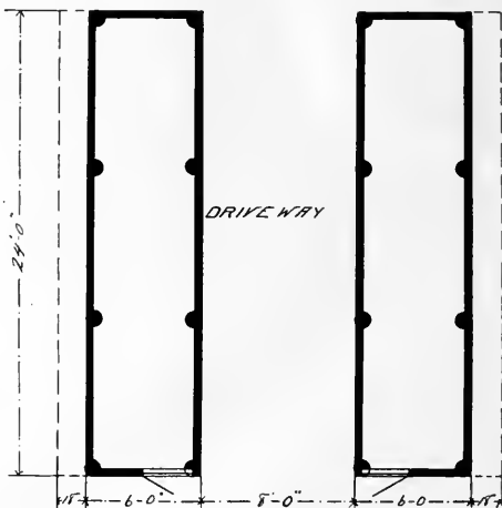
FLOOR PLAN OF DOUBLE CORN CRIB
