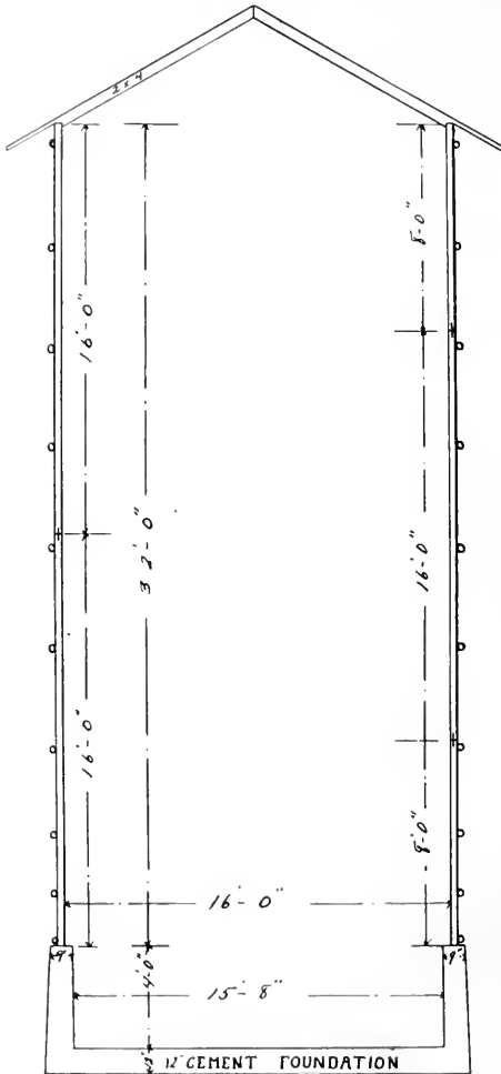
CROSS SECTION OF SILO
