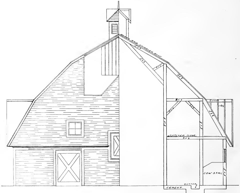
SECTION
