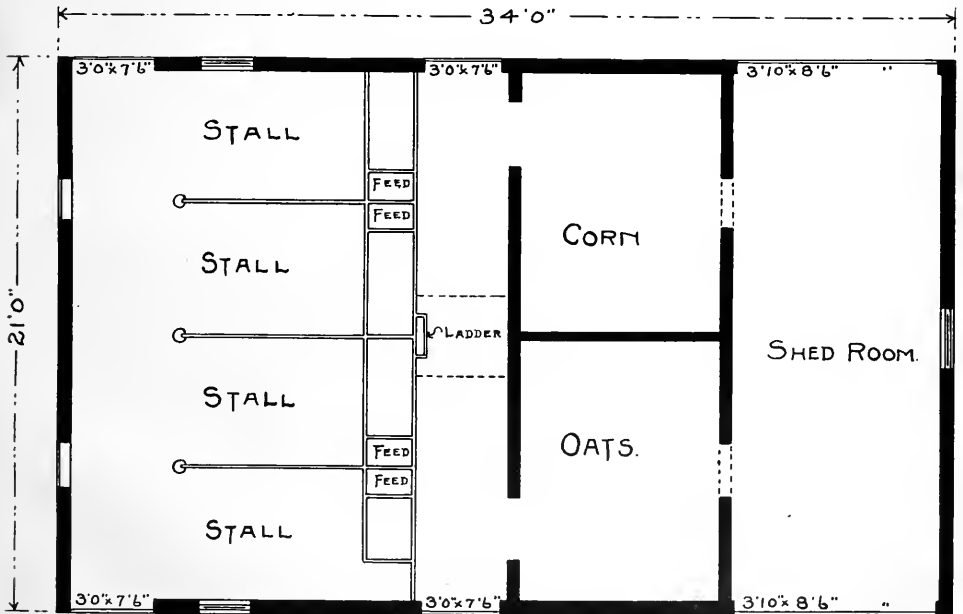
FLOOR PLAN.
