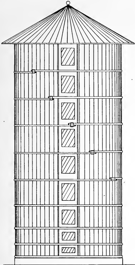
ELEVATION OF SILO
