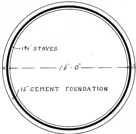
PLAN OF SILO
