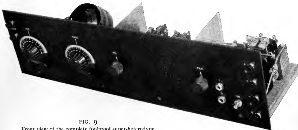
Front view of the complete foolproof super-heterodyne
