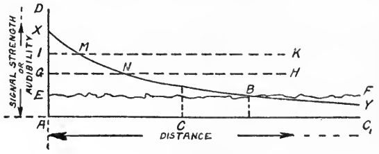
FIG. 4 A crystal set can receive San Francisco's signal at IM distance from the transmitting station, a regenerative set at GN distance, and a super-heterodyne at any distance up to point B
