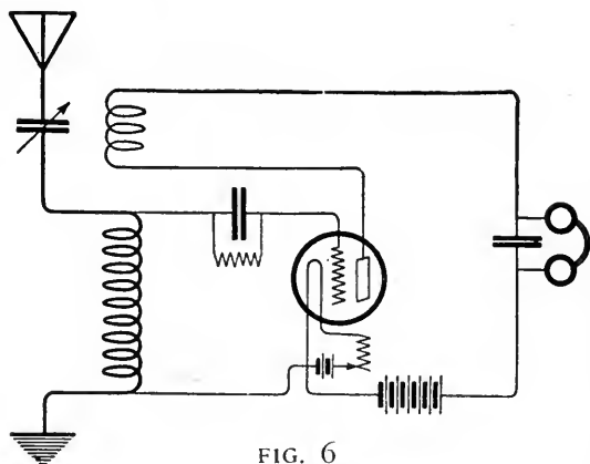
A so-called single circuit receiver employing a tickler or feed-back coil for regeneration. Note that in Fig. 5 S has been moved over to its rightful place as secondary. This circuit can easily be changed, then, to operate with a Sodian tube
