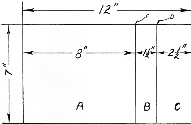
PANEL LAYOUT
