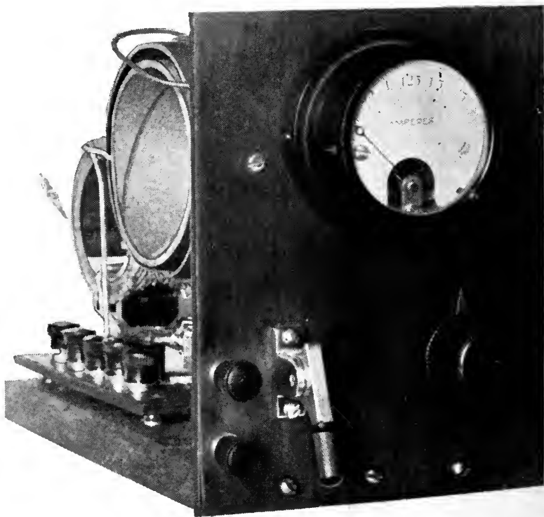
FIG. 2 The ideal beginner's C. W. transmitter which has a daylight range of about five miles and can be built for less than $20
