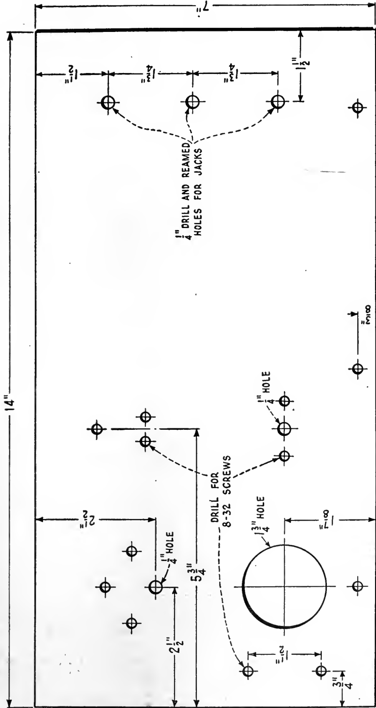
FIG. 5 Working drawing of panel, half actual size
