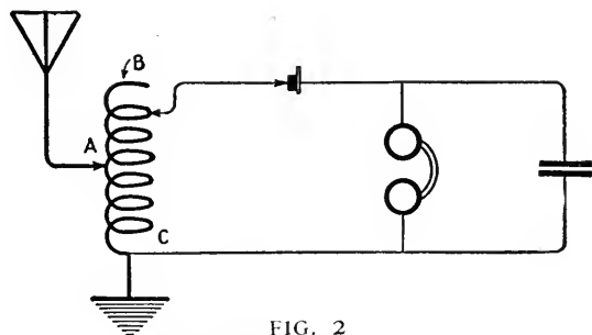
FIG. 2 A typical single-circuit receiver
