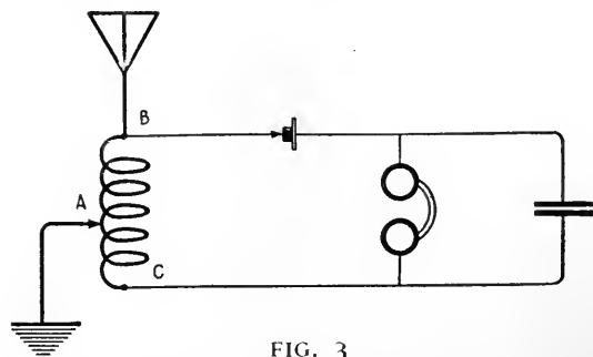
FIG. 3 An improvement over the arrangement shown in Fig. 2
