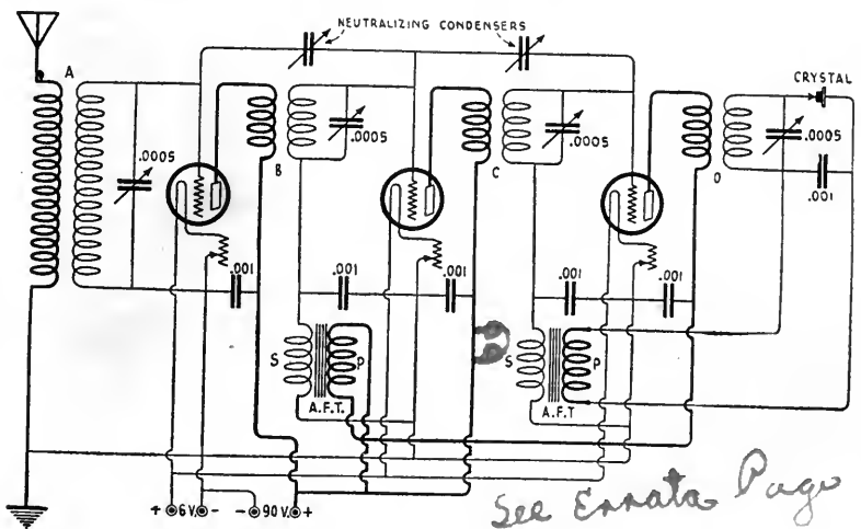
FIG. 5 The best Inverse Duplex circuit we have yet seen. The neutrodyne condenser helps smother self-oscillations
