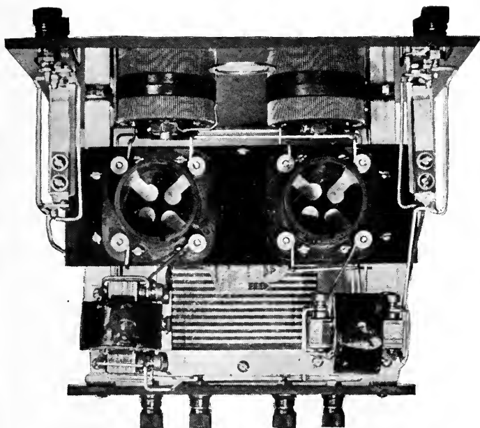
THE COMPLETED UNIT Looking from above
