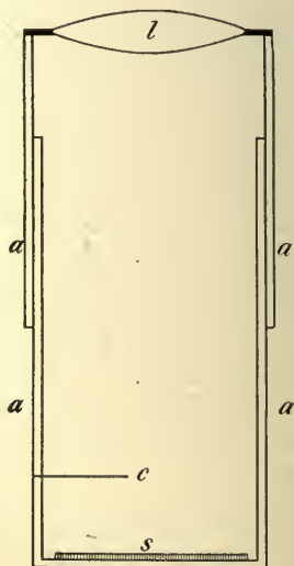
Diagram of spintariscope. An infinitesimal amount of radium is held by a needle ( c ) over a screen of zinc sulphide ( s ). The lens ( l ) is mounted so as to focus upon the screen; inside of box should be black.
