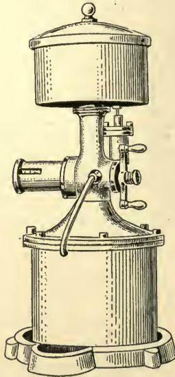
Emanator for charging drinking-water. The handle on the side prevents the withdrawal of an excess amount.
