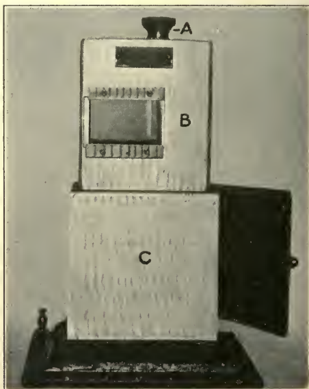
An electroscope used at the Oncologic Hospital: C , the ionizing chamber; B , electroscope proper; A , cap covering the insulated rod holding the leaf.
