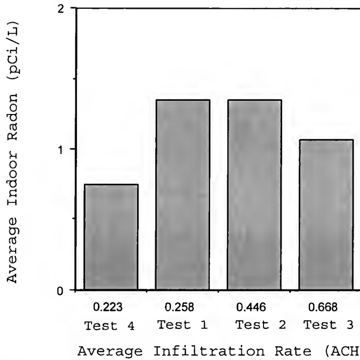
Figure 4.8 Indoor Radon Levels vs. Infiltration Rates
