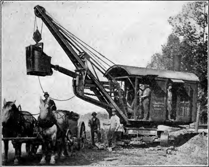
FIG. 10.—Thew Shovel.
