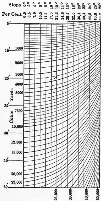
FIG. 81.—Cubic Yards per Station, with Transverse Slope.
