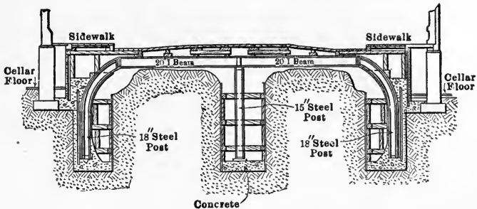
FIG. 29.—The Cut and Cover Method.
