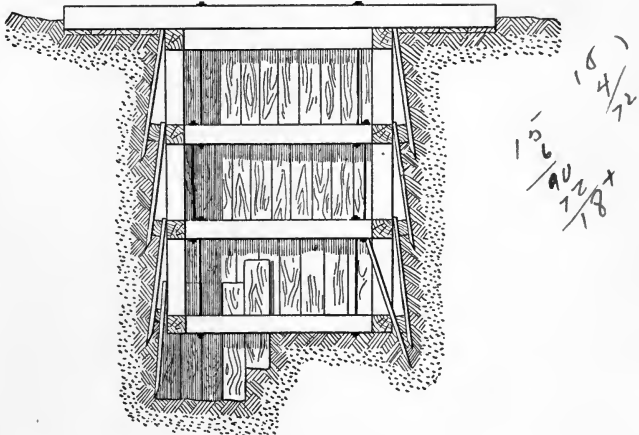
FIG. 17.—Shaft Timbering.
