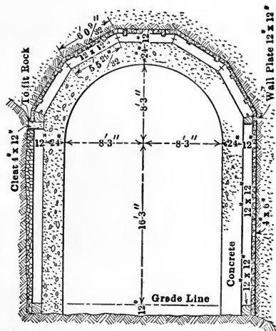
FIG. 21.—Concrete Lining.
