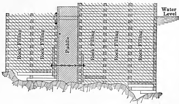
FIG. 36.—Crib Cofferdam.
