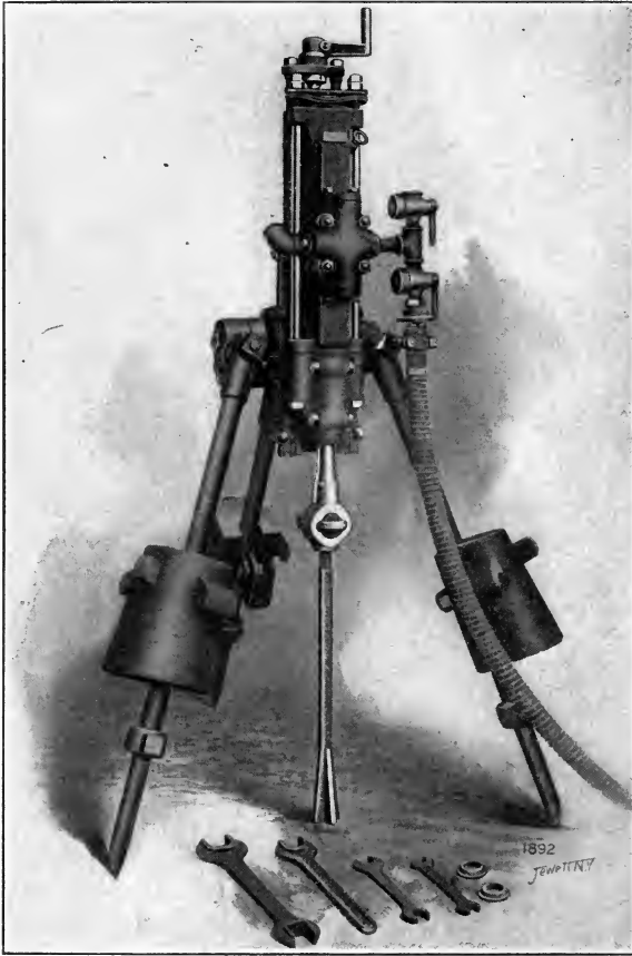
FIG. 15.—Sergeant Rock Drill.
