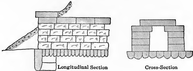
FIG. 44.—West Shore Railroad Single Box Culvert.
