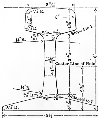
FIG. 71.—Dudley 100-lb. Rail.
