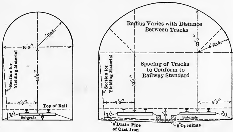
FIG. 18.—Inside Dimensions.
