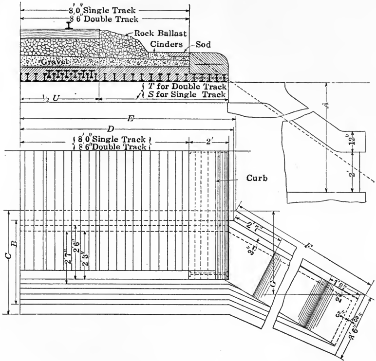
FIG. 49.—New York Central Railroad Rail Floor Culverts.
