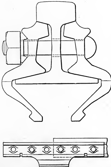
FIG. 74.—100 Per Cent. Type of Joint
