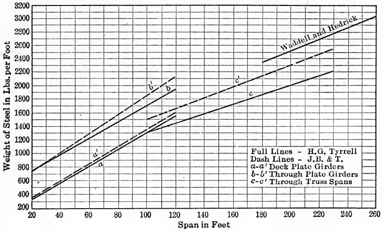
FIG. 67.—Weights per Foot of Steel Bridges.
