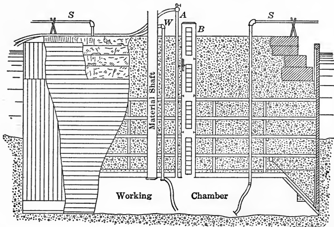
FIG. 37—Pneumatic Caisson.
