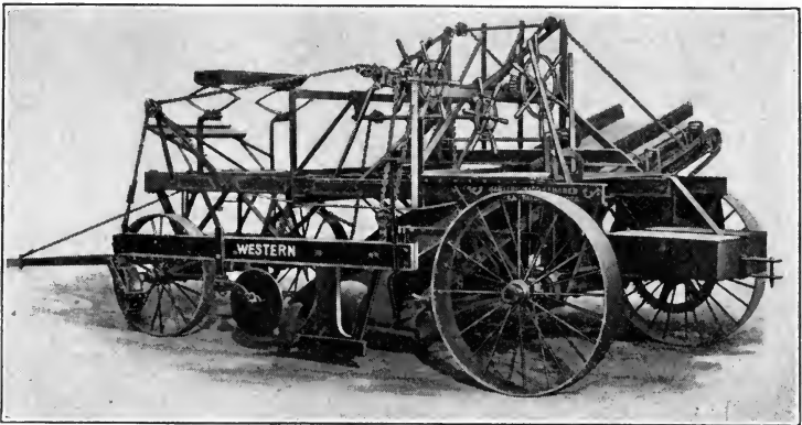
FIG. 8.—Elevating Grader.
