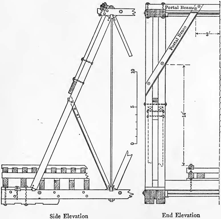
FIG. 65.—Portal Bracing, Oregon Pacific Howe Truss.
