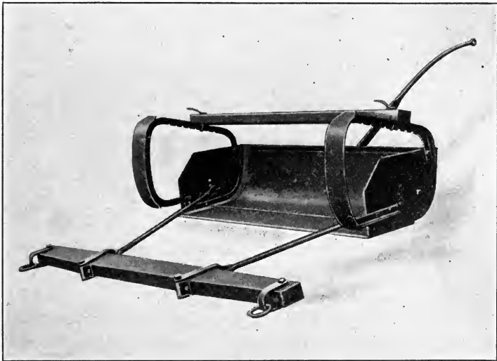
FIG. 5.—Fresno Scraper.
