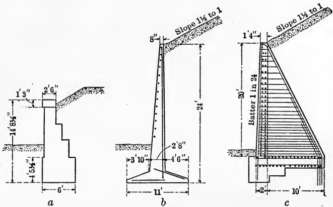
FIG. 50.—Retaining Wall Sections.
