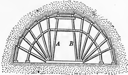
FIG. 23.—Arch Timbering.
