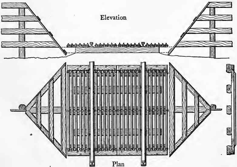
FIG. 79.—Wooden Surface Cattle Guard.
