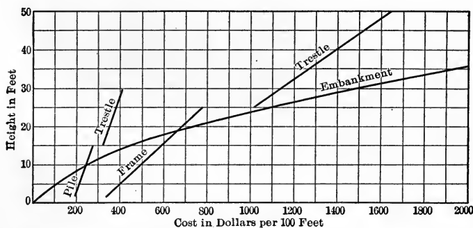
FIG. 62.—Comparison of Wooden Trestle and Embankment.
