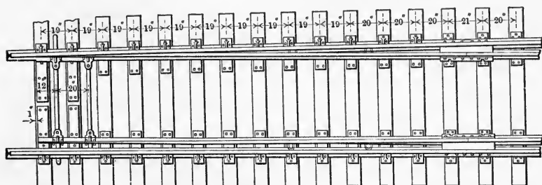
Fig. 76.—Point Switch.
