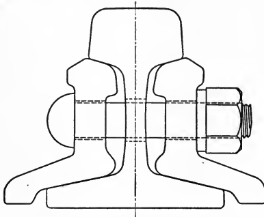
FIG. 73.—Angle Bar Splice
