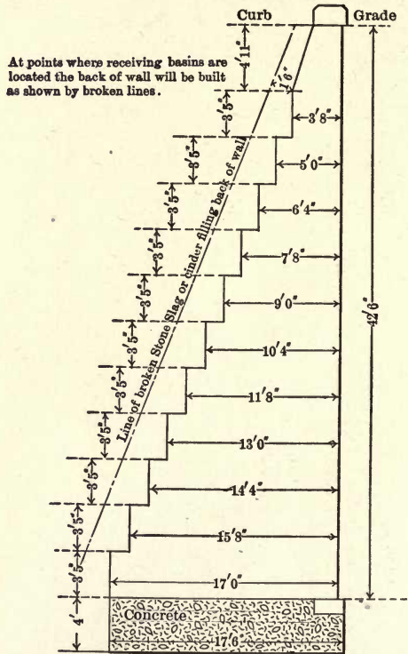
Fig. 37. Retaining Wall, Harlem River Speedway.
