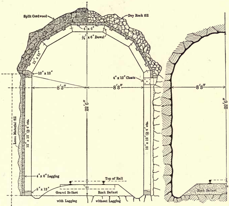
Figs. 41 and 42. Tunnels.
