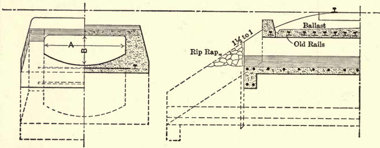
Fig. 21. Rail Concrete Culvert.
