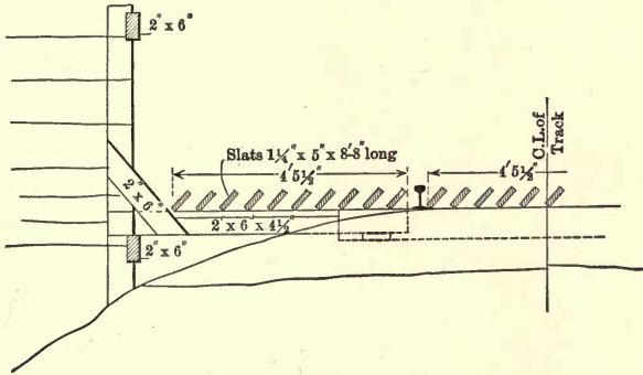
Fig. 18. Wood Cattle Guard.
