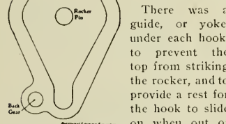
FIG. 22. ROGERS'S CONNECTED DOUBLE HOOK.
