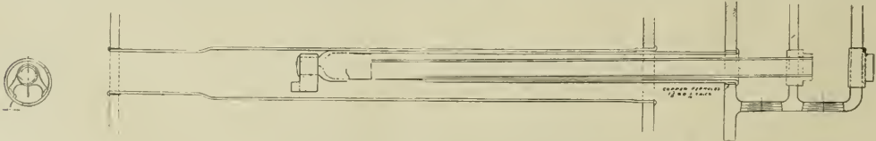
ARRANGEMENT OF PIPES IN THE SCHENECTADY SUPERHEATER, D., I. & W. ENGINE.
