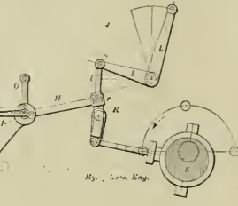
FIG. 33. A. J. STEVENS' VALVE MOTION.
