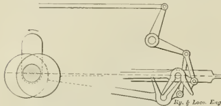
FIG. 10. PACWELS' VALVE GEAR.
