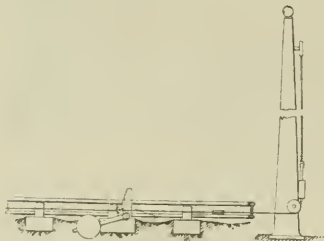
SIDE VIEW OF STOP SIGNAL WITH TRIP BESIDE RAILS.
