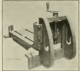
LATHE ATTACHMENT FOR BORING.
