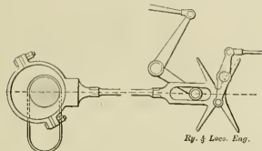
FIG. 5. CARMICHAEL'S VALVE GEAR.
