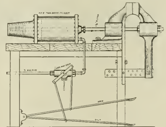
AIR OPERATED BENCH VISE.
