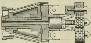
TUBE CLEANER.
