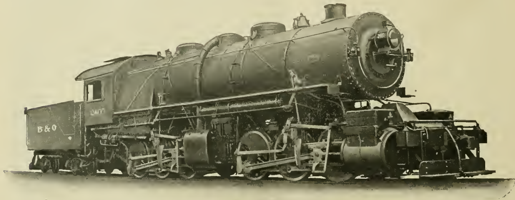
MALLET ARTICULATED COMPOUND ON THE BALTIMORE & OHIO.
