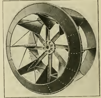
CONSTRUCTION OF THE FAN.
