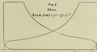
INDICATOR DIAGRAMS FROM ENGINE EQUIPPED WITH CLARK'S VALVE MOTION.
