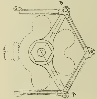
FIG. 2—PLAN OF GUARD SUPPORT.
