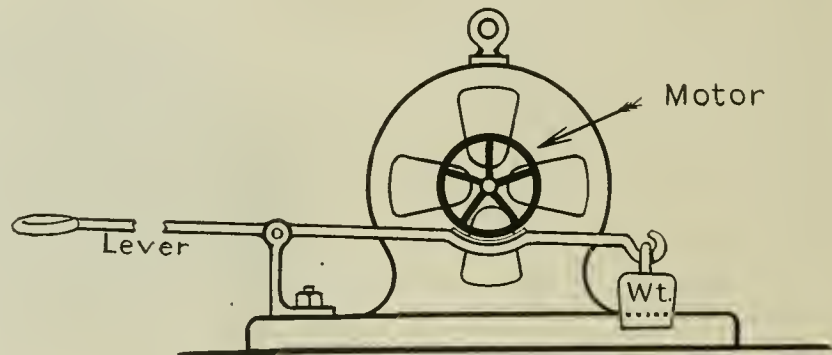
IMPROVISED HAND BRAKE ON ELECTRIC MOTOR.
