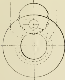
FIG. 1—STAYBOLT WRENCH.
