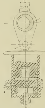
CYLINDER OF BELL RINGER
