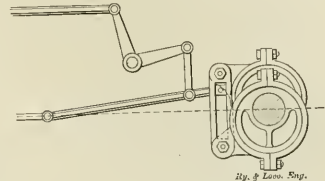
FIG. 16. PRETENDED WILLIAMS' LINK MOTION.
