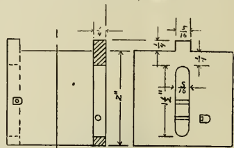
CASE SHOWING CROSS PINS FOR KEYS
