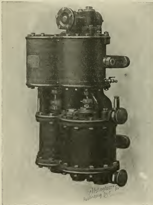
FIG. 1. 8½-INCH CROSS COMPOUND PUMP.
