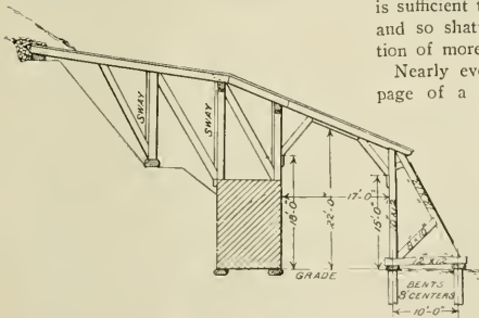
SNOW SHED ON COMPARATIVELY FLAT INCLINE.
