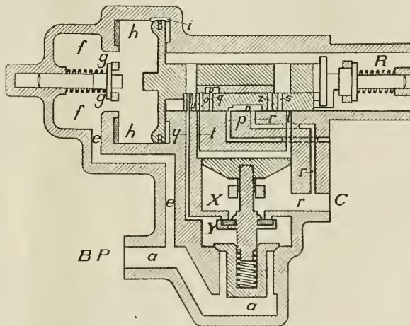
FIG. 2. FULL RELEASE AND CHARGING POSITION.
