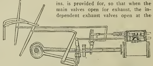
ROGERS' LINK MOTION AND INDEPENDENT CUT-OFF.
