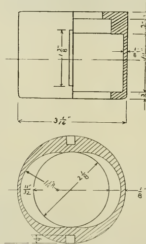
CASE WITH CRESCENT SHAPED CAVITIES FOR KEYS
