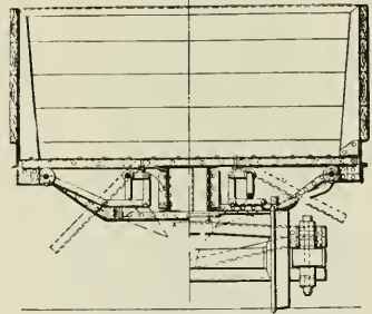
CAMPBELL DROP-BOTTOM GONDOLA.
