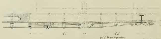
DOOR DETAILS ON PENNSYLVANIA BOX CAR.
