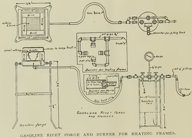
GASOLINE RIVET FORGE AND BURNER FOR HEATING FRAMES.
