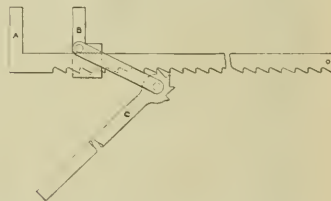
DEVICE FOR PULLING CROSSHEADS
