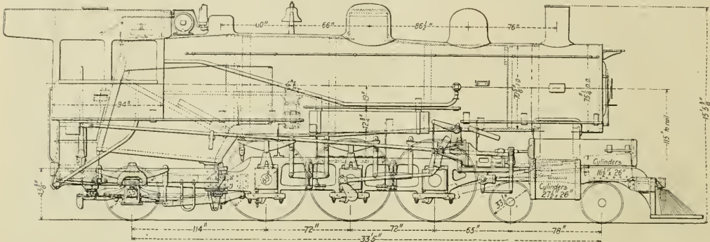
GENERAL PLAN OF NORTHERN PACIFIC BALANCED COMPOUND
