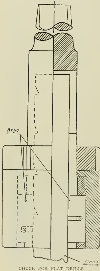
CHUCK FOR FLAT DRILLS
