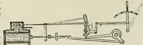
FIG. 23. BALDWIN'S VARIABLE CUT-OFF MOTION.
