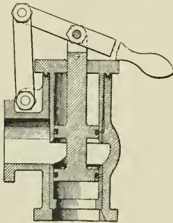
BLOW-OFF VALVE
