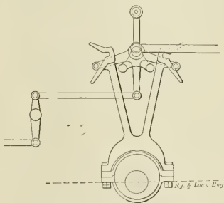
FIG. 7. FORRESTER'S VALVE GEAR.
