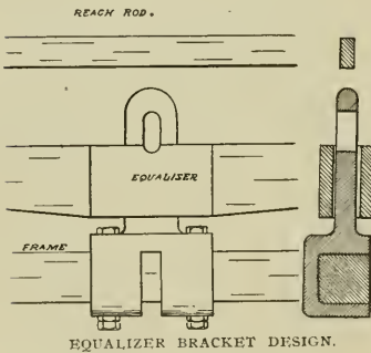
EQUALIZER BRACKET DESIGN.
