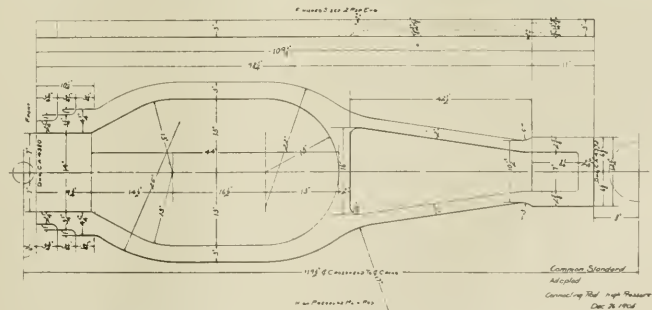
HIGH PRESSURE CONNECTING ROD, SURROUNDING LEADING AXLE.
