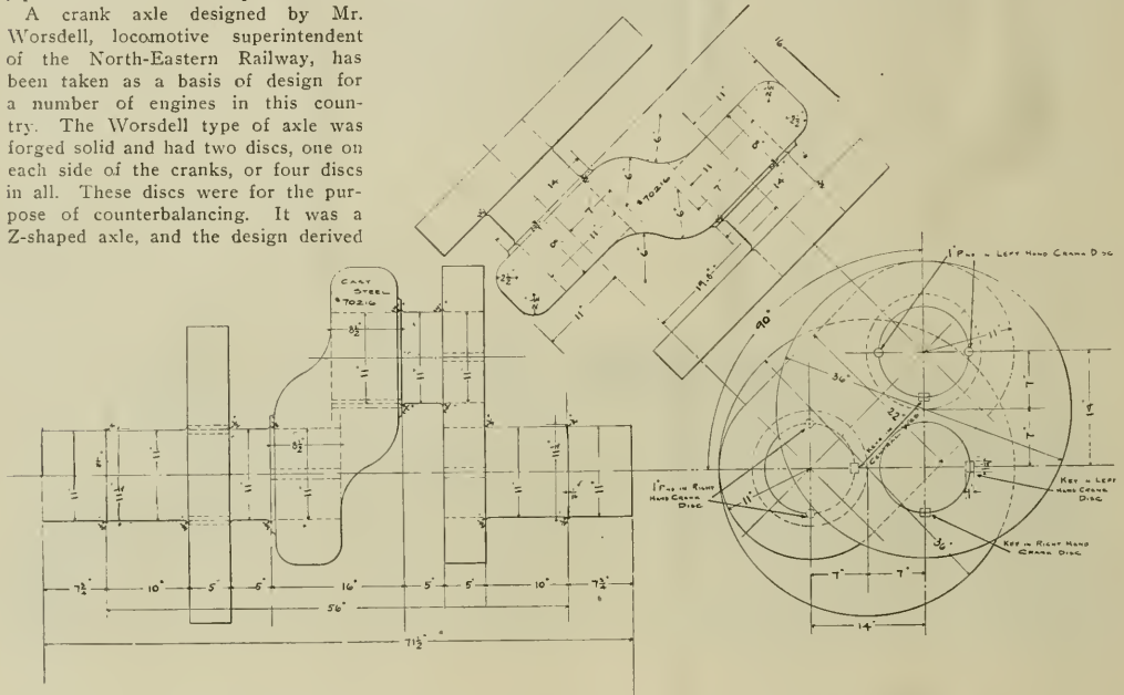
CRANK AXLE OF UNION PACIFIC 4-4-2 ENGINE. IT IS MADE IN SEVEN PIECES.
