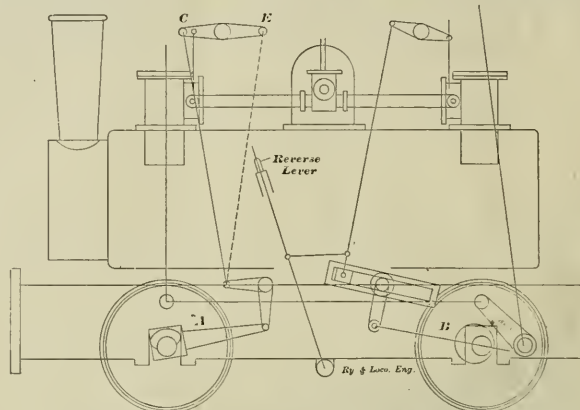
FIG. 1. ORIGINAL AND ALTERED FORM OF VALVE MOTION.
