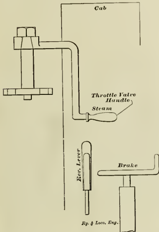
FIG. 3. TRANSVERSE SECTION THROUGH CAB LOOKING FROM FRONT OF OLD ENGINE.
