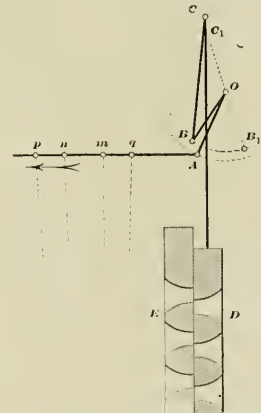
FIG. 36. STRONG VALVE GEAR.
