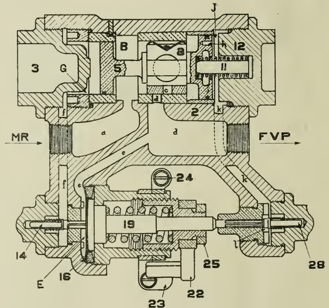
WESTINGHOUSE "K" FEED VALVE, CLOSED POSITION.
