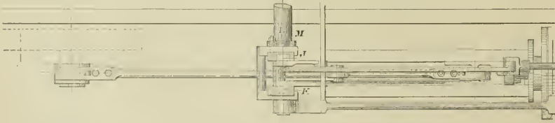
FIG. 2. PLAN OF JOY'S VALVE GEAR.
