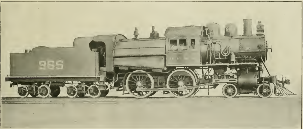
SIMPLE 4-4-0 ENGINE WITH SUPERHEATER FOR THE D., L. & W.
