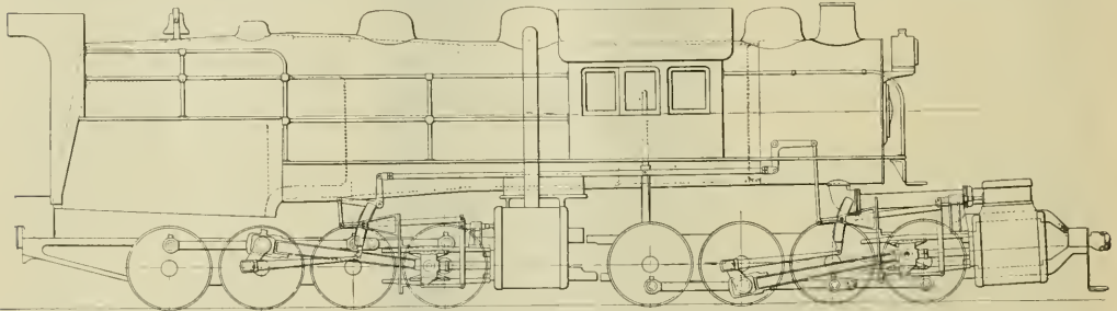
OUTLINE OF MALLET COMPOUND FOR THE ERIE RAILROAD
