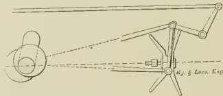
[FIG. 11. STEPHENSON'S VALVE GEAR.
