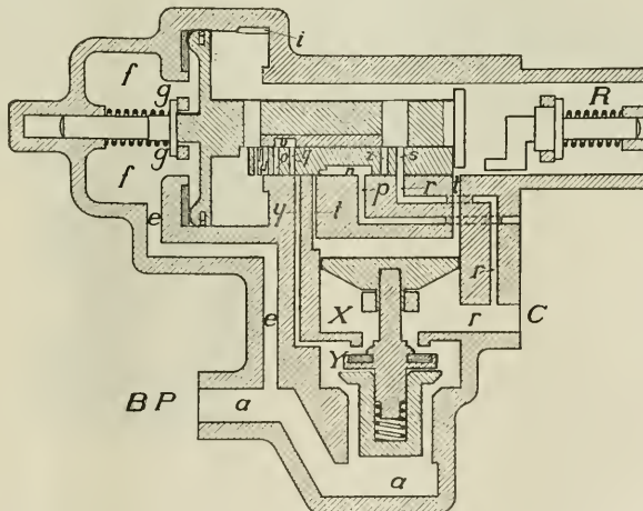
FIG. 6. EMERGENCY POSITION.
