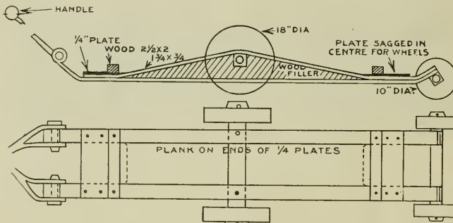
CAR OR COACH-WHEEL CARRIAGE FOR THE SHOP.
