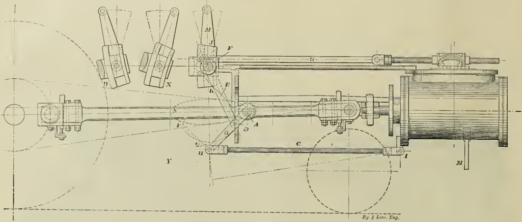
FIG. 1. ELEVATION JOY'S VALVE GEAR.
