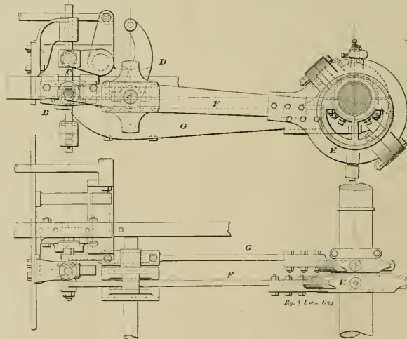
FIG. 35. WILLIAM WILSON'S VALVE MOTION.
