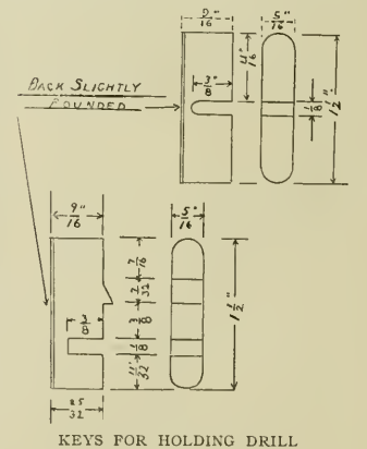
KEYS FOR HOLDING DRILL
