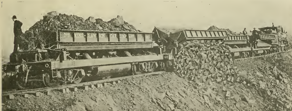
"CAUGHT WITH THE GOODS." INSTANTANEOUS PHOTOGRAPH OF THE KING-LAWSON CAR IN ACTION.
