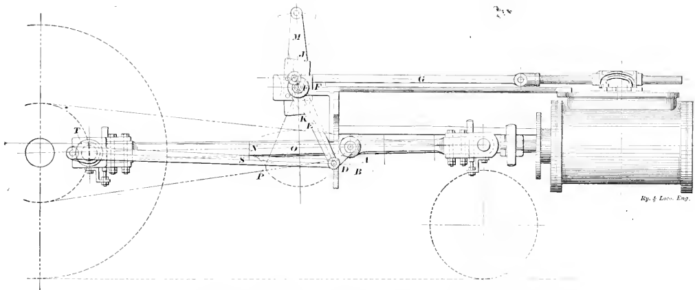
FIG. 4. JOY'S VALVE GEAR MODIFIED TO RAISE PARTS FROM TRACK.
