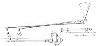
FIG. 6. BURY'S DROP HOOK GEAR.
