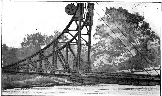
ERIE LIFT BRIDGE, WITH COMPENSATING WEIGHT.
