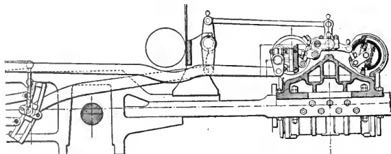
FIG. 38. SECTION OF YOUNG'S ADAPTATION OF THE CORLISS PRINCIPLE.
