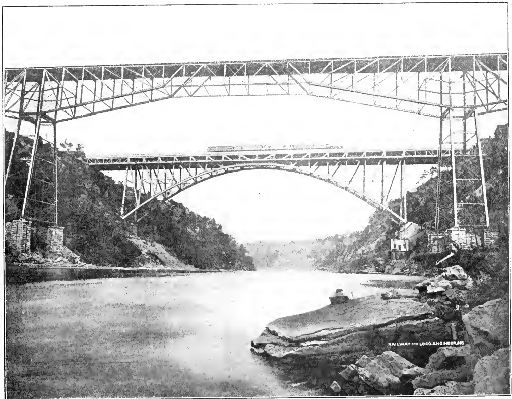
RAILROAD BRIDGES OVER THE NIAGARA GORGE. THE CANTILEVER AND THE STEEL ARCH
