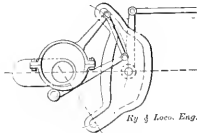
FIG. 13. CRAMPTON'S EXPANSION GEAR.
