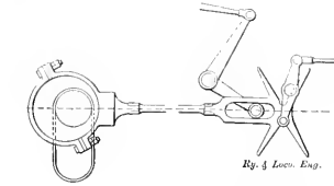
FIG. 5. CARMICHAEL'S VALVE GEAR.
