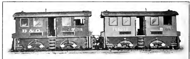
TWO SECTION ELECTRIC FREIGHT LOCOMOTIVE, B. & O.
