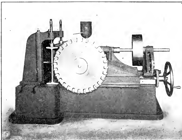
MODERN COLD METAL CUTTING OFF MACHINE.
