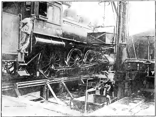
FIG. 1. LOADED ASH BUCKET HOISTED READY TO SWING OVER ASH CAR
