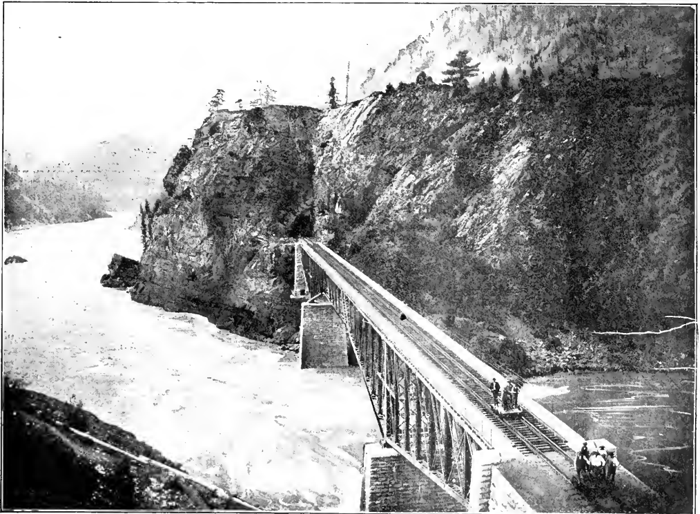
CANTILEVER BRIDGE OVER THE FRASER RIVER, C. P. R., BRITISH COLUMBIA.
