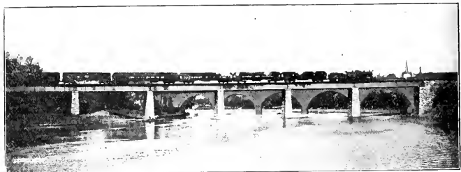
STEEL GIRDER AND BRICK ARCH RAILWAY BRIDGES
