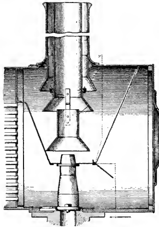
EXHAUST MECHANISM
