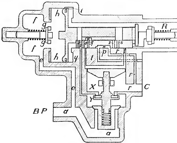
FIG. 5. RETARDED RELEASE POSITION.
