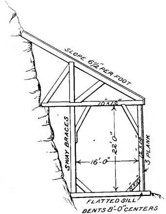
SNOW SHED ON A STEEP INCLINE.
