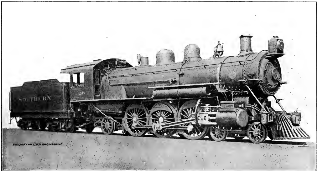
PASSENGER 4-6-2 ENGINE FOR THE SOUTHERN.
