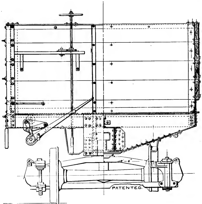
END ELEVATION AND SECTION, RALSTON CAR.
