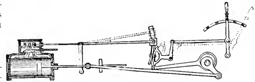
FIG. 23. BALDWIN'S VARIABLE CUT-OFF MOTION.
