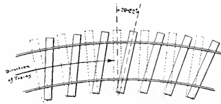
FIG. 2. TIES SHIFTED ON CURVE.
