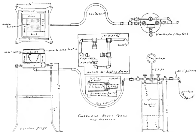
GASOLINE RIVET FORGE AND BURNER FOR HEATING FRAMES.
