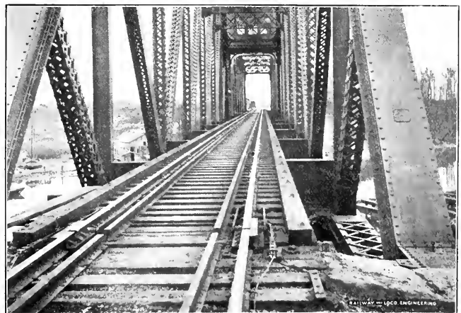
INTERIOR OF SWING SPAN, SHOWING CONTACT FOR ELECTRIC SIGNAL CIRCUIT.
