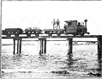
BUILDING THE JETTY AT BANDON, ORE. TIDE COMING IN.
