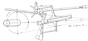
FIG. 9. HAWTHORN'S RADIAL GEAR.
