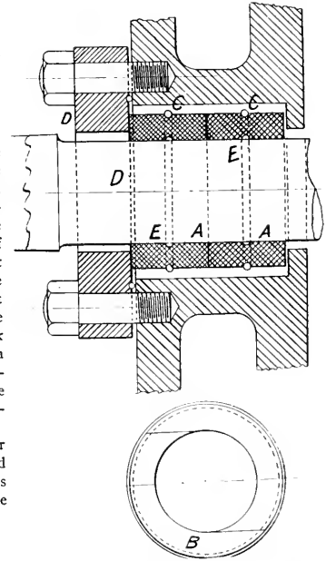
PISTON ROD AND VALVE STEAM PACKING.
