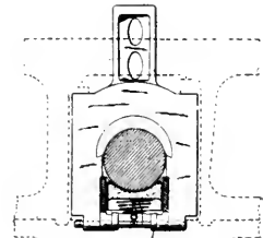
AXLE BOX LUBRICATOR.
