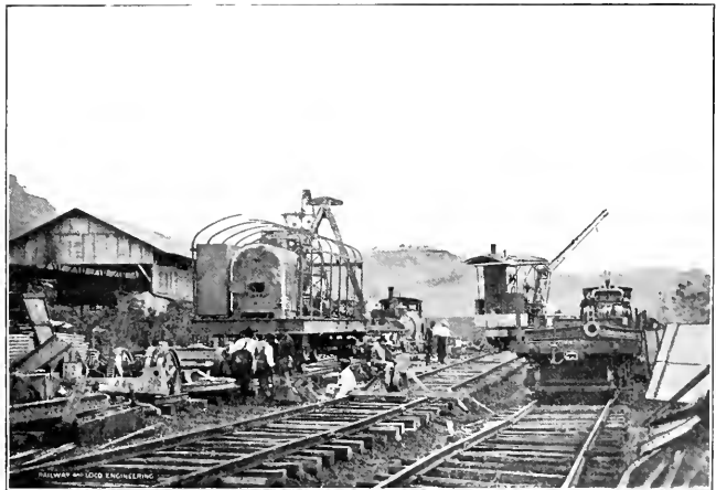
ERECTING A STEAM SHOVEL ON THE GROUND
