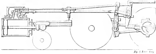
FIG. 34. DAVID CLARK'S VALVE MOTION.
