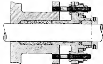
METHOD OF TIGHTENING GLAND.
