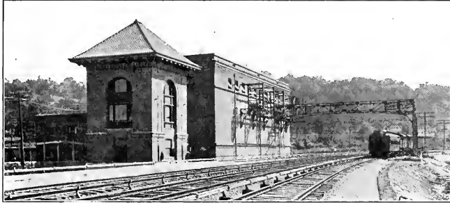
SUB-STATION, TRAIN, TRACK AND THIRD RAIL ON THE N. Y. C. (Courtesy of Street Railway Journal.)
