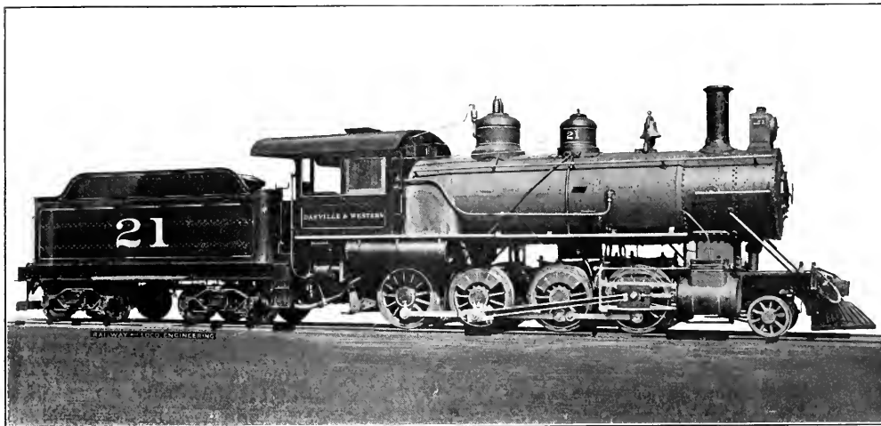
CONSOLIDATION ENGINE FOR THE DANVILLE & WESTERN.
