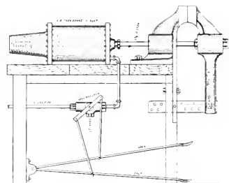
AIR OPERATED BENCH VISE.
