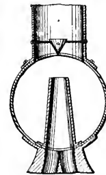
EXHAUST SPLITTER
