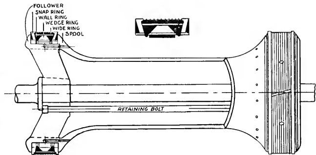
SECTION OF THE SEMI-PLUG VALVE.
