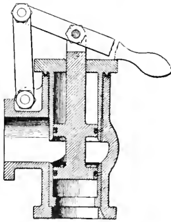
BLOW-OFF VALVE
