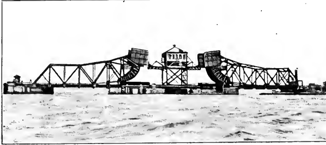
DOWN STREAM VIEW OF ROLLER LIFT BRIDGE OVER NEWARK BAY, N. J.
