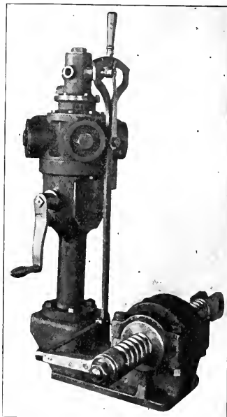
AIR OPERATED REVERSING MECHANISM, MALLETT COMPOUND.
