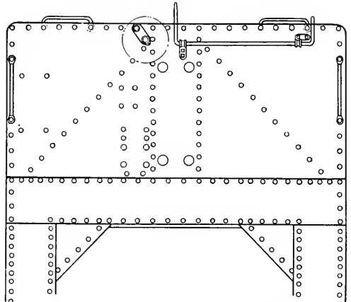
PLAN OF END OF PENNSYLVANIA FLAT CAR SHOWING ENDS OF BOX GIRDERS, DIAGONAL BRACES AND SHORT END PLATFORM.
