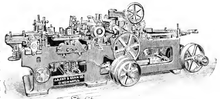
INSIDE MOLDER CUTS FOUR SIDES.
