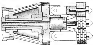
TUBE CLEANER.
