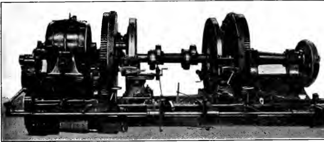
59-INCH MOTOR DRIVEN NILES BEMENT-POND WHEEL LATHE, C. R. I. & P. SHOPS.
