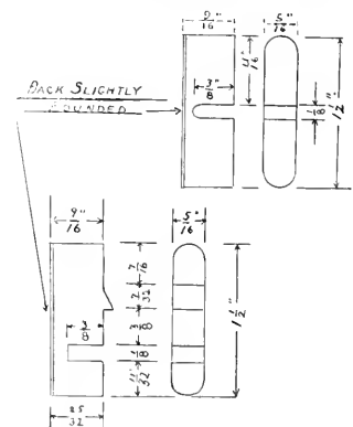
KEYS FOR HOLDING DRILL
