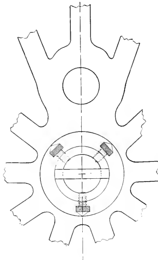
ADJUSTABLE CENTERING DEVICE.
