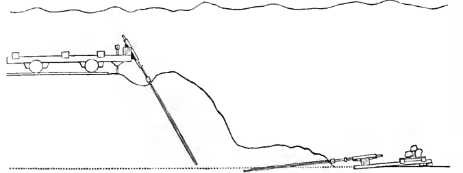
TAKING OUT BOTTOM BY HOLES DRILLED FROM HEADING AND ALONG FLOOR. (Reproduced from "Drinker's Tunneling.")
