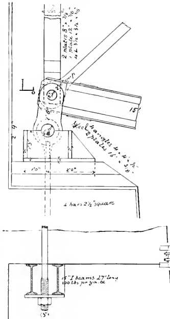
FIG. 2. ANCHORAGE SYSTEM, FRASER RIVER BRIDGE.
