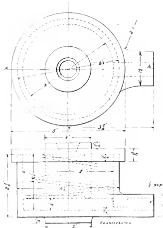
PNEUMATIC HOLDING ON DEVICE FOR FIRE BOX SEAMS.
