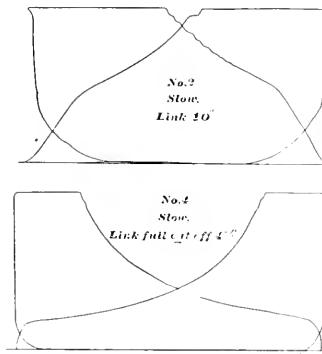
INDICATOR. DIAGRAMS FROM ENGINE EQUIPPED WITH CLARK'S VALVE MOTION.
