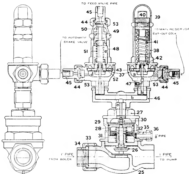
S-D-4 PUMP GOVERNOR.
