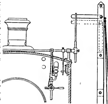
STOP SIGNAL DEVICE.
