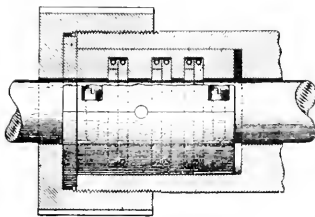
PISTON ROD PACKING.
