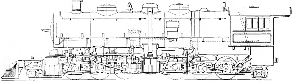
SIDE ELEVATION OF BALDWIN MALLET ARTICULATED COMPOUND ENGINE.
