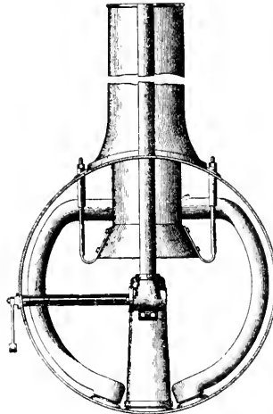
EXHAUST MECHANISM.
