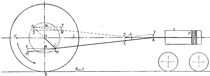
DIAGRAM SHOWING FORCES ACTING A DRIVING WHEEL.
