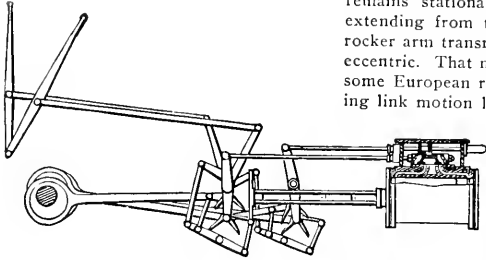
FIG. 25. ROGERS VALVE MOTION. =
