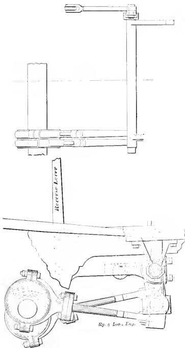
LINK MOTION USED BY BALDWIN IN 1840. (Referred to on page 135 of R.V. AND L. E.)
