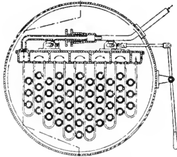
NEW SUPERHEATER.
