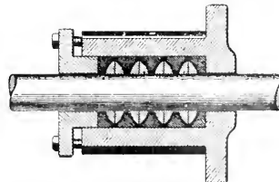
METALLIC PACKING.
