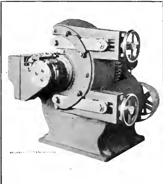
ACME THREAD ROLLING MACHINE. Back View.
