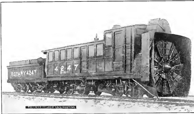
SIDE VIEW OF ROTARY SNOW PLOW.
