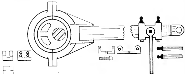
ECCENTRIC ROD BENDER OR TWISTER.
