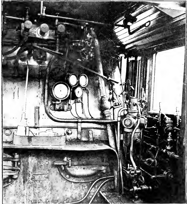
INTERIOR OF CAB OF BALDWIN MALLETT ARTICULATED LOCOMOTIVE SHOWING REVERSING MECHANISM.
