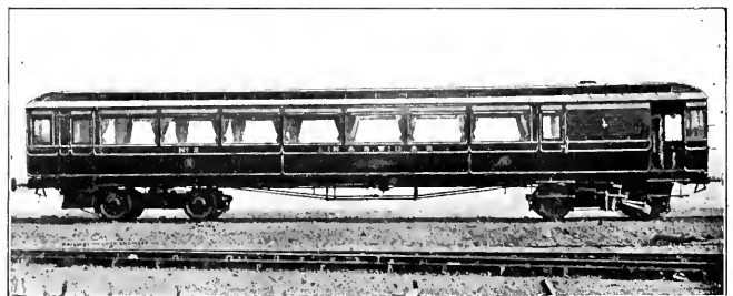
STEAM MOTOR CAR USED IN GLASGOW
