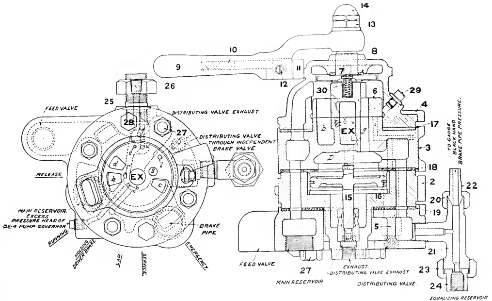
FIG. 1. H. BRAKE VALVE, AUTOMATIC BRAKE.
