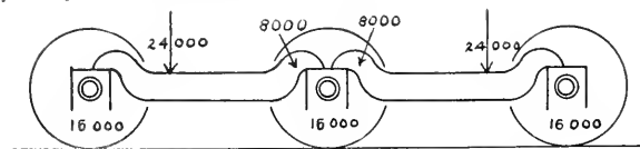
FIG. 4. LOAD AS IT IS IN PRACTICE ON RAILWAYS.
