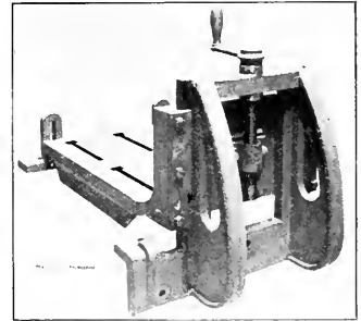
LATHE ATTACHMENT FOR BORING.
