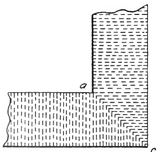
FIG. 1. CASTING WITHOUT FILLET
