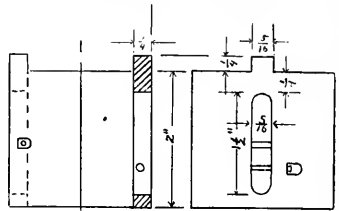
CASE SHOWING CROSS PINS FOR KEYS
