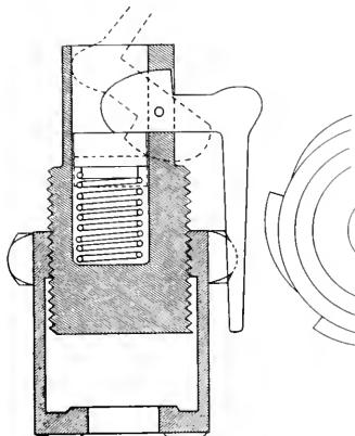
FINCH'S LEVER LOCK GREASE CUP.
