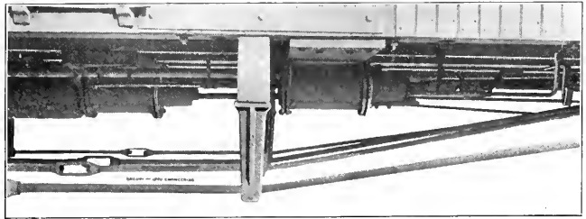
SAUVAGE BRAKE IN FULL RELEASE.
