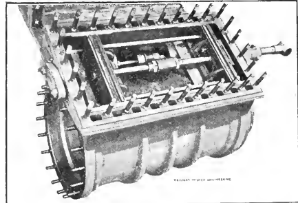
FIG. 33. ARRANGEMENT OF ALL-FREE-HUBBELL VALVES.
