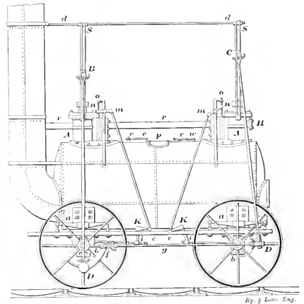
FIG. 4 FIRST USE OF AN ECCENTRIC ON LOCOMOTIVES.
