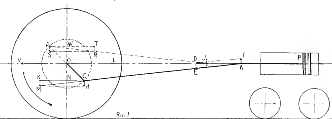
DIAGRAM SHOWING FORCES ACTING A DRIVING WHEEL.
