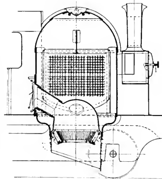
BOILER OF COCHRAN'S MOTOR.
