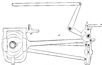
UHRY & LUTTGENS' CAM-LINK MOTION, 1806.
