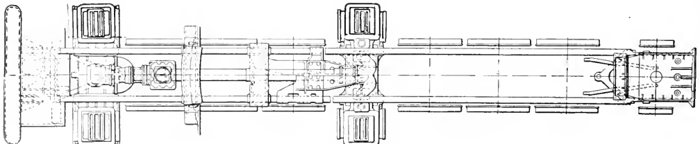
PLAN OF BALDWIN MALLET COMPOUND ENGINE FOR THE GREAT NORTHERN.
