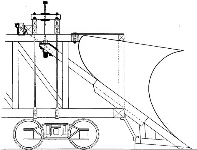
SNOW FLOW ATTACHED TO ORE CAR, C. & N. W.
