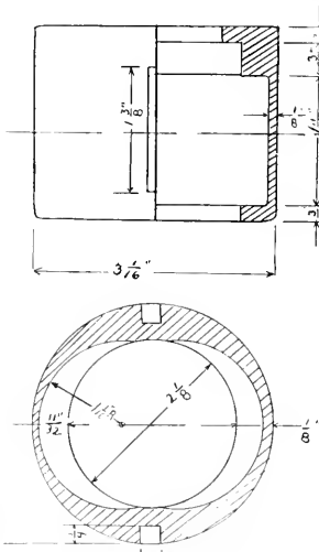
CASE WITH CRESCENT SHAPED CAVITIES FOR KEYS
