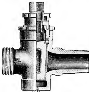
Fig. 9. All Brass, extra heavy, with Cased Plug For 250 lbs. pressure. Made with Draining Plug to prevent freezing.
