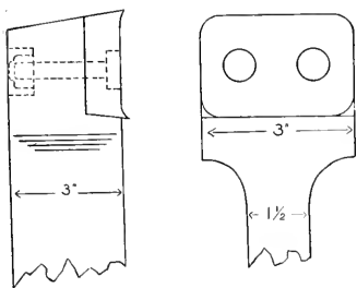
FIG. 1. TREAD FINISHING TOOL.
