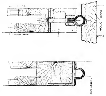
DETAILS OF EDGE OF DOOR AND DOOR STOP.
