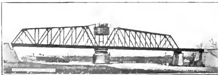
BLACK RIVER SWING, ON THE NICKEL PLATE. CANTILEVER FOR THE DEAD LOAD, CONTINUOUS GIRDER FOR THE LIVE LOAD.
