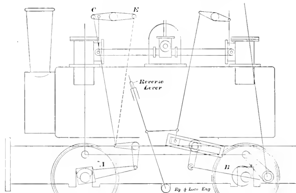
FIG. 1. ORIGINAL AND ALTERED FORM OF VALVE MOTION.
