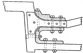
TEMPORARY FRAME PATCH
