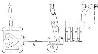
FIG. 18. ROSS WINANS' VALVE GEAR.
