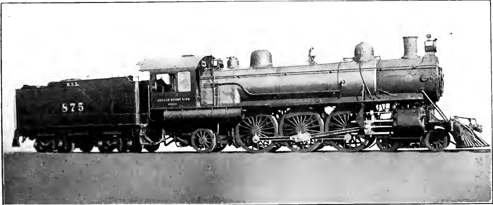
PRAIRIE TYPE ENGINE FOR THE OREGON SHORT LINE.
