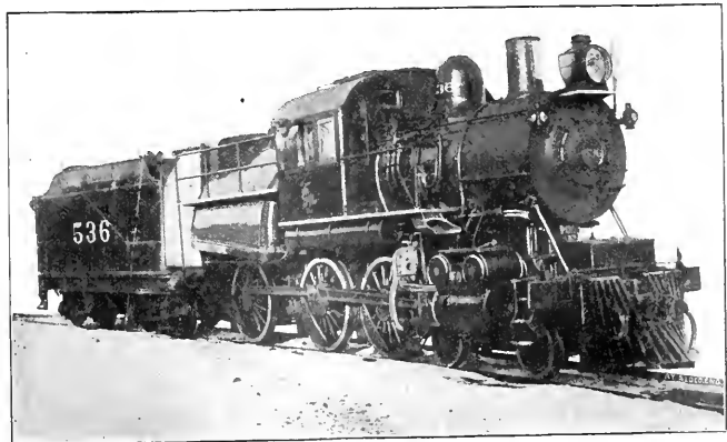
D. & H. ENGINE WITH YOUNG'S ROCKING VALVES.
