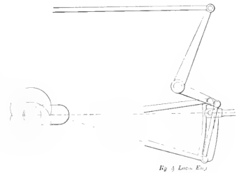
FIG. 17. ORIGINAL LINK MOTION.
