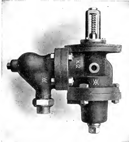
FIG. 1. WESTINGHOUSE "K" TRIPLE VALVE
