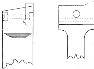
FIG. 2. TREAD FINISHING AND CHAMFERING TOOL.
