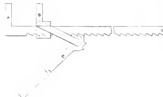
DEVICE FOR PULLING CROSSHEADS
