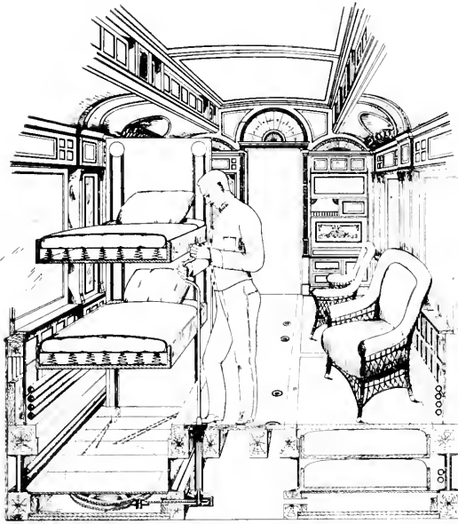
SECTION OF COACH SHOWING METHOD OF LIFTING BEDS AND STEEL BERTH POCKET BELOW CAR FLOOR.
