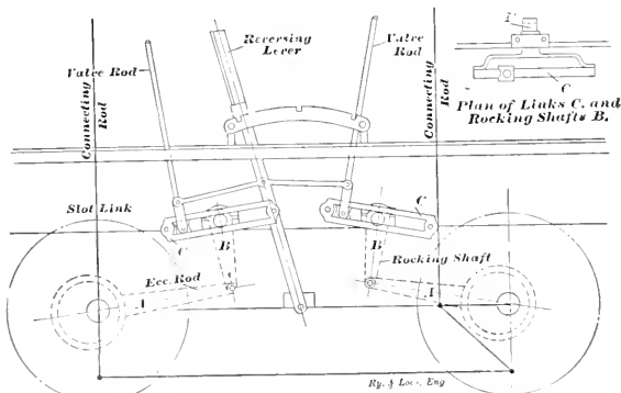
FIG. 2. PRESENT DAY VALVE GEAR OF OLD ENGINE.
