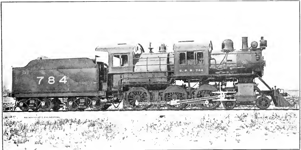
CANADIAN PACIFIC TEN WHEELER FREIGHT AND PASSENGER ENGINE.
