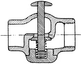
EXHAUST VALVE WITH PUSH BUTTON.
