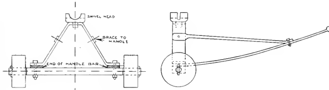
SHOP SULKY OR GENERAL UTILITY PONY TRUCK.
