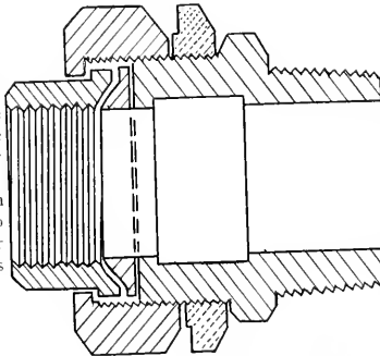
LOCK NUT ON PUMP CONNECTION
