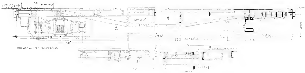
STRUCTURAL STEEL PLAT CAR FOR THE PANAMA RAIL ROAD. BUILT BY THE STANDARD STEEL CAR CO OF PITTSBURGH.
