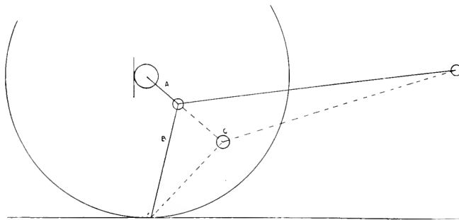
WHEEL DIAGRAM LONG AND SHORT STROKE ENGINES.
