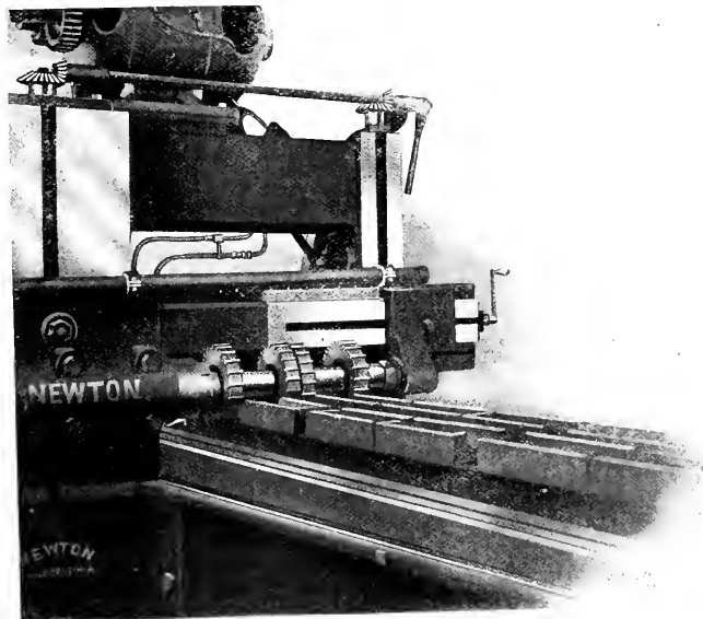
NEWTON MILLING MACHINE FINISHING LOCOMOTIVE DRIVING SHOES.
