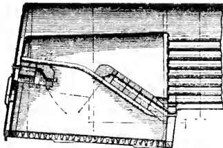
LOCOMOTIVE FURNACE.
