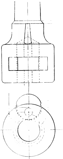
FIG. 1 STAYBOLT WRENCH.
