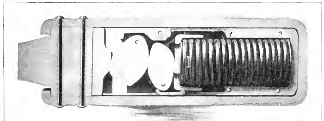
NEW CAM LEVER DRAW GEAR.
