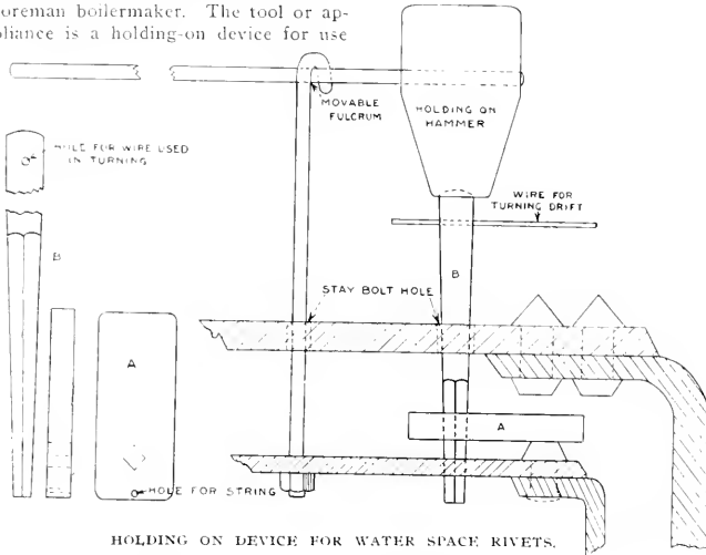
HOLDING ON DEVICE FOR WATER SPACE RIVETS.
