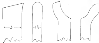
FIG. 3. ROUGHING AND FLANGE FINISHING TOOLS.
