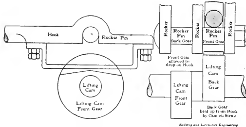
FIG. 19. COMMON FORM OF DROP HOOK MOTION.
