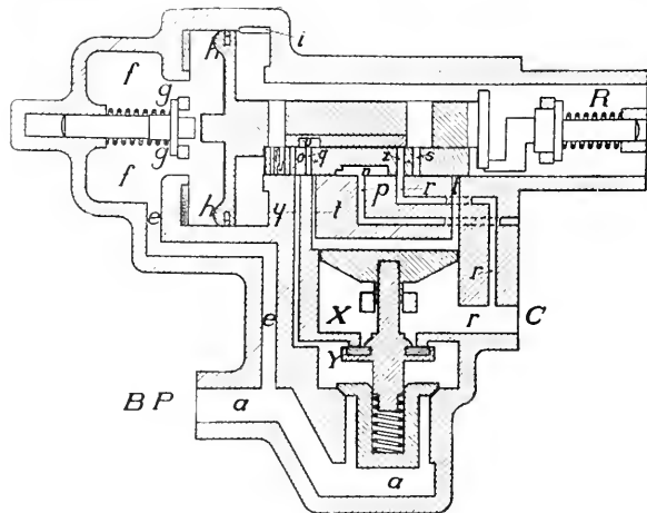
FIG. 4. SERVICE LAP POSITION.
