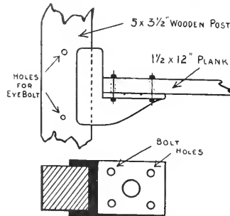
SLIDE AND BRACKET FOR SCAFFOLDING.
