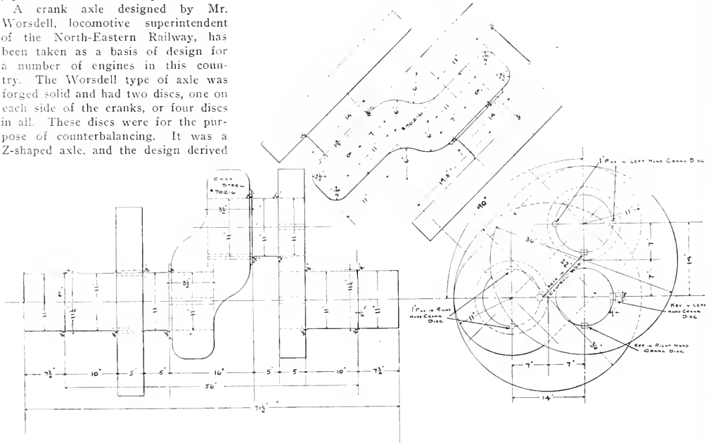
CRANK AXLE OF UNION PACIFIC 4-4-2 ENGINE. IT IS MADE IN SEVEN PIECES.
