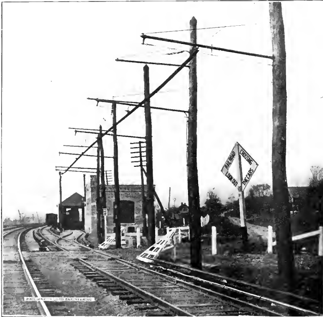
TEST TRACK FOR N. Y. C. ELECTRIC LOCOMOTIVES SHOWING THIRD RAIL ALONG THE LINE AND OVERHEAD CONTACT FOR HIGHWAY CROSSINGS
