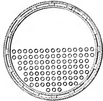
BOILER JACKET
