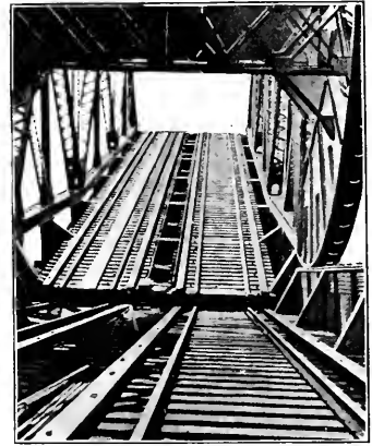
INTERIOR VIEW, BRIDGE PARTLY RAISED.
