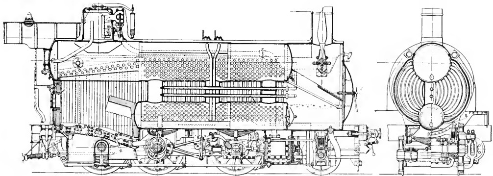
ROBERT WATER-TUBE BOILER FOR P. L. M. RAILWAY.
