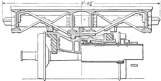
CROSS SECTION SHOWING BODY BOLSTER AND TRUCK CRADLE.
