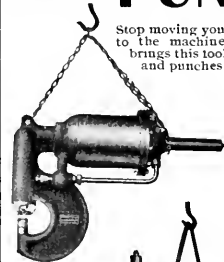
Punch Size 8
