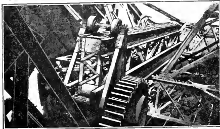
RACK FRAME FOR LIFTING ROLLER BRIDGE OVER NEWARK BAY—C. R. R. OF N. J.
