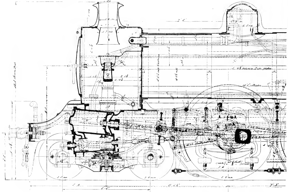
THREE CYLINDER COMPOUND ENGINE
