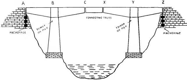
FIG. 1. SKELETON VIEW OF TYPICAL CANTILEVER BRIDGE.
