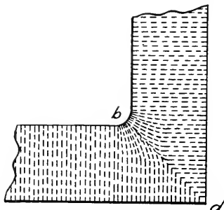
FIG. 2 ARRANGEMENT OF PARTICLES WHEN FILLET IS USED
