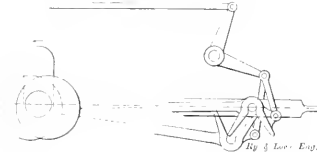
FIG. 10. FAWCELS' VALVE GEAR.
