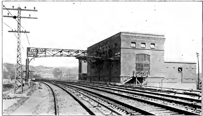
N. Y. C. SUB-STATION NO. 3, SHOWING POLE AND OVERHEAD CONSTRUCTION
