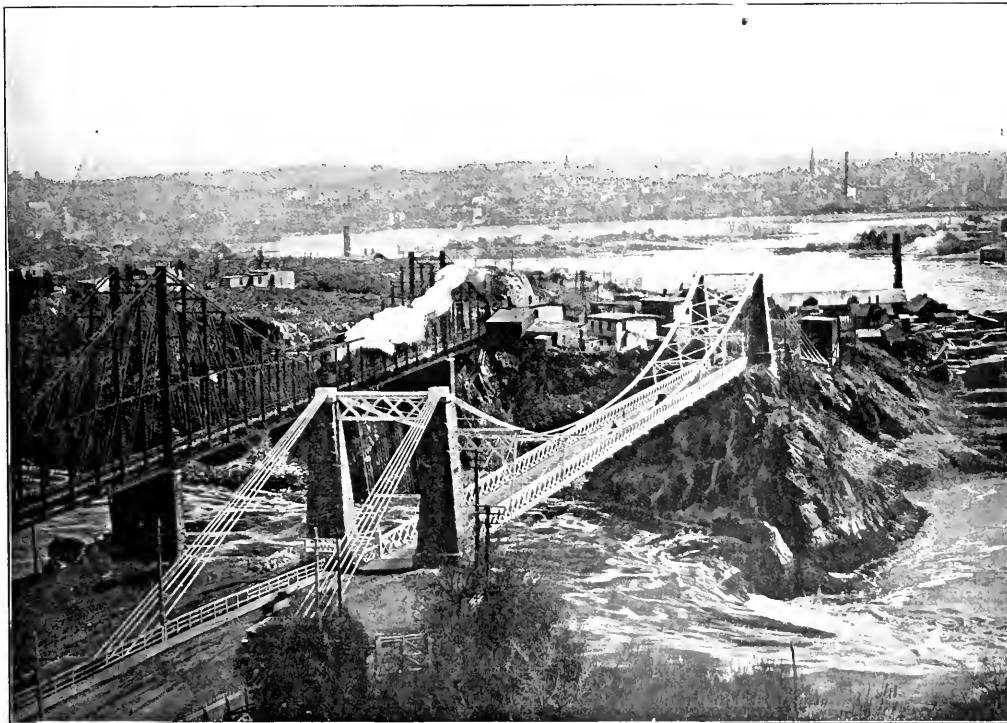
RAILWAY AND ROAD BRIDGES OVER THE ST. JOHN RIVER, NEW BRUNSWICK, CANADA.
