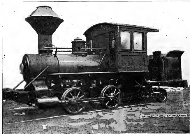
ENGINE WITH OSCILLATING CYLINDER AND NO VALVE GEAR
