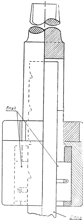
CHUCK FOR FLAT DRILLS
