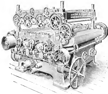
TRIPLE DRUM SANDER.
