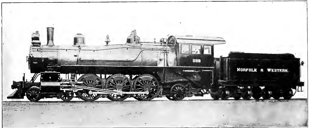
SINGLE EXPANSION 4-6-2, FOR THE NORFOLK & WESTERN.
