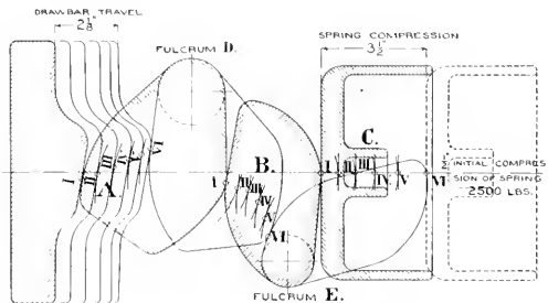
DIAGRAM SHOWING MOVEMENT OF CAMS.
