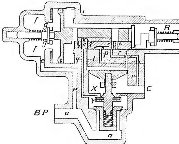
FIG. 3. SERVICE POSITION.
