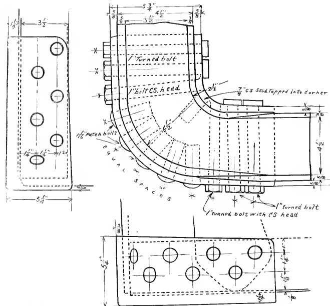
MUD RING PATCH, WINNIPEG SHOPS, CANADIAN PACIFIC RAILWAY.
