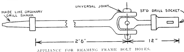
APPLIANCE FOR REAMING FRAME BOLT HOLES.
