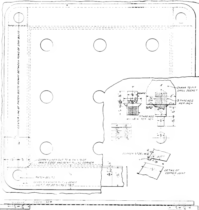
METHOD OF APPLYING PATCH TO LOCOMOTIVE FIRE BOX.
