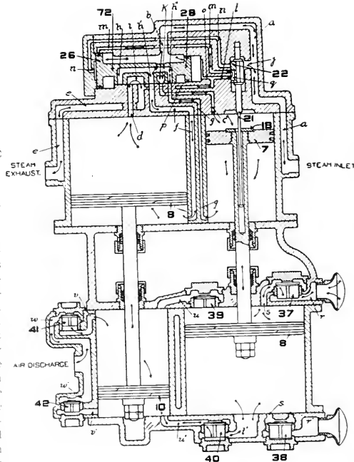
FIG. 3. DIAGRAM OF THE CROSS COMPOUND PUMP DOWN-STROKE HIGH-PRESSURE-STEAM SIDE.
