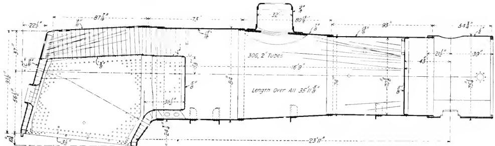
BOILER OF NORTHERN PACIFIC 4-6-2 ENGINE, SHOWING COMBUSTION CHAMBER
