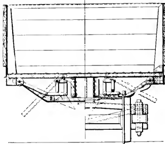
CAMPBELL DROP-BOTTOM GONDOLA.
