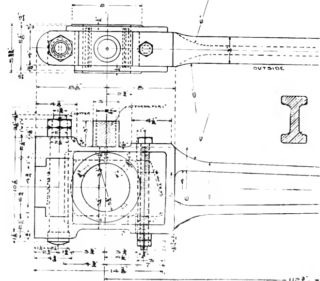
FORK END OF CONNECTING ROD. L. & N. E. RAILROAD.
