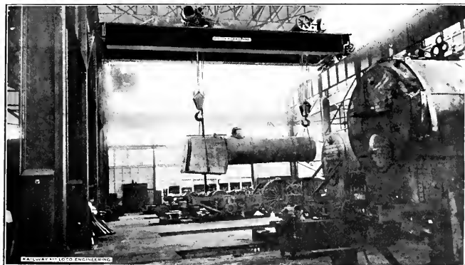
LIFTING A BOILER, TEXAS & PACIFIC SHOPS, MARSHALL, TEX.
