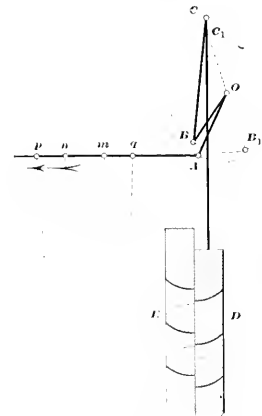
FIG. 36. STRONG VALVE GEAR.
