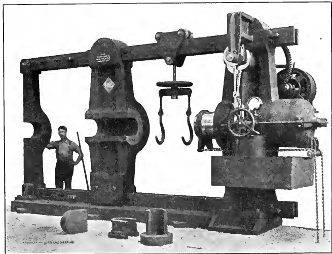
HYDRAULIC WHEEL PRESS, 600-TONS CAPACITY.
