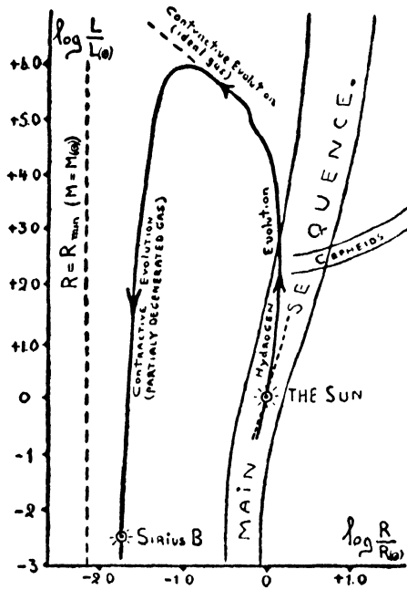
FIG. Evolutionary track of a light star.
