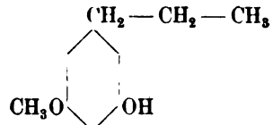
(1)Propyl-(5)methoxy-(3)phenol
