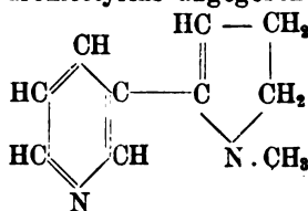
Dihydrornicotyrin.
