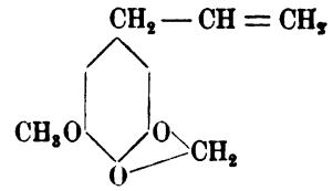
Myristicin
