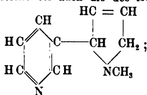
Nicotein
