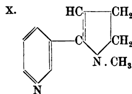
Dihydronicotyrin.
