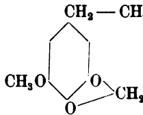
Dihydromyristicin
