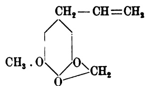
Myristicin.
