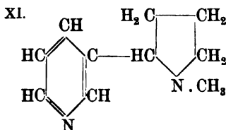
Tetrahydronicotyrin = i-Nicotin.
