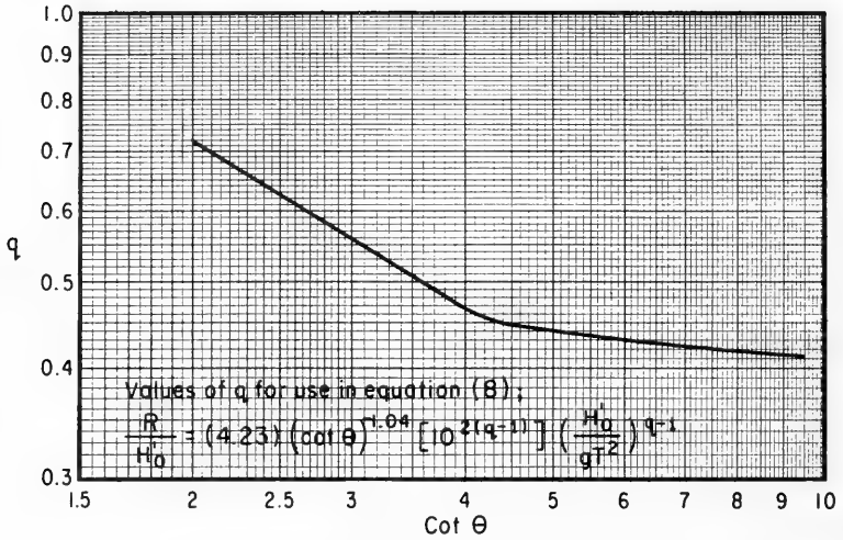
Figure 5. Values of q for equation (8).
