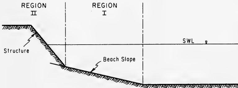
Figure 11. Regions of breaking waves for depth-related instabilities.
