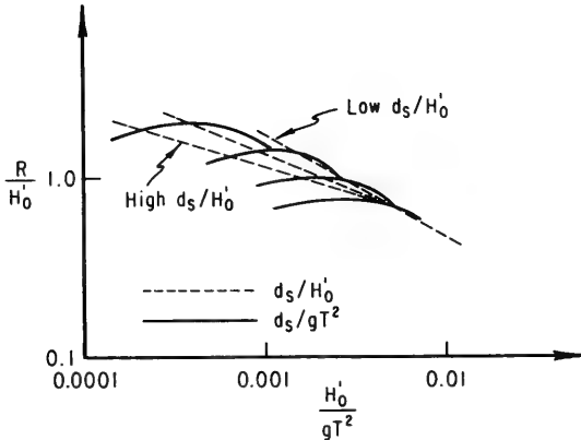
Figure 8. Sketch of lines of d_s/H_0' related to lines of d_s/gT^2 for a fixed slope.
