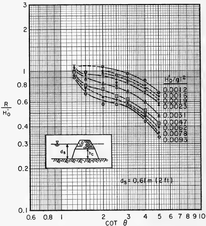
Figure 27. Quarystone rubble-mound runup; d_s/H_0' = 8.0 ; H_0'/k_r = 1.7 ; h_c/d_s \approx 0.75 (after Hudson, 1958).
