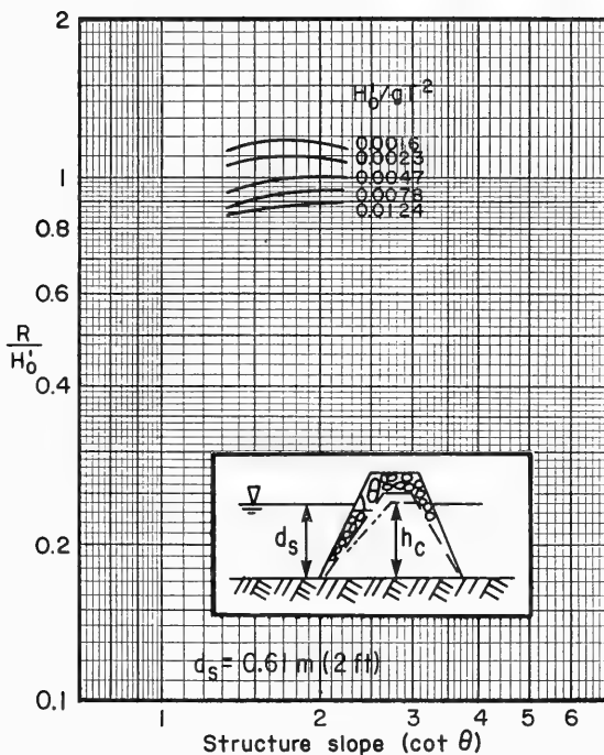
Figure 28. Quarrystone rubble-mound runup ("smooth" stones); random placement; d_s/H_0^1 = 5.0 ; H_0^1/k_T = 2.7 ; h_c/d_s \approx 1.10 (after Jackson, 1968a).
