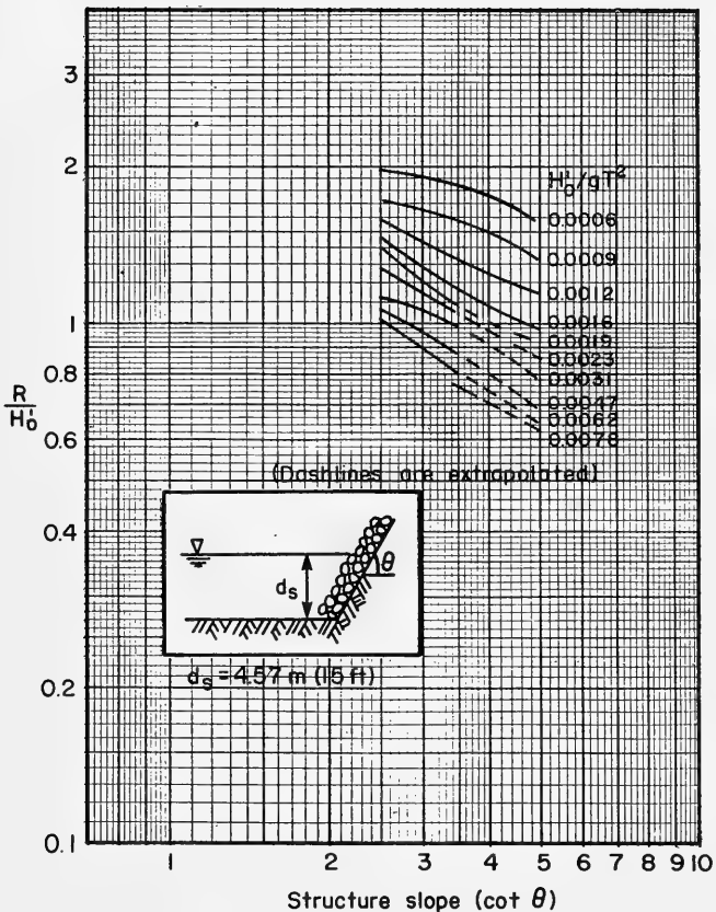
Figure 41. Relative runoff for riprap slopes; d_s/H_0' = 8.0 ; H_0'/k_p = 2.8 (after Ahrens, 1975a).
