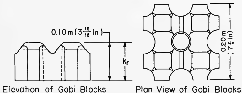
Figure 44. Gobi blocks (McCartney and Ahrens, 1975).
