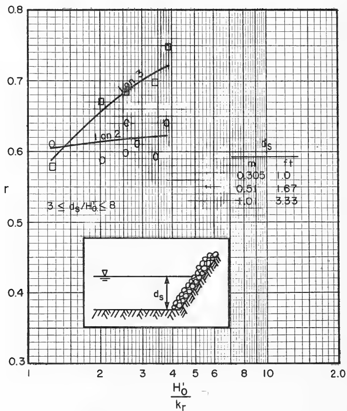
Figure 35. Values of r for slope and relative roughness ( H_0^1/k_r ) for riprap slopes; armor layer approximately two stones thick (after Hudson and Jackson, 1962).
