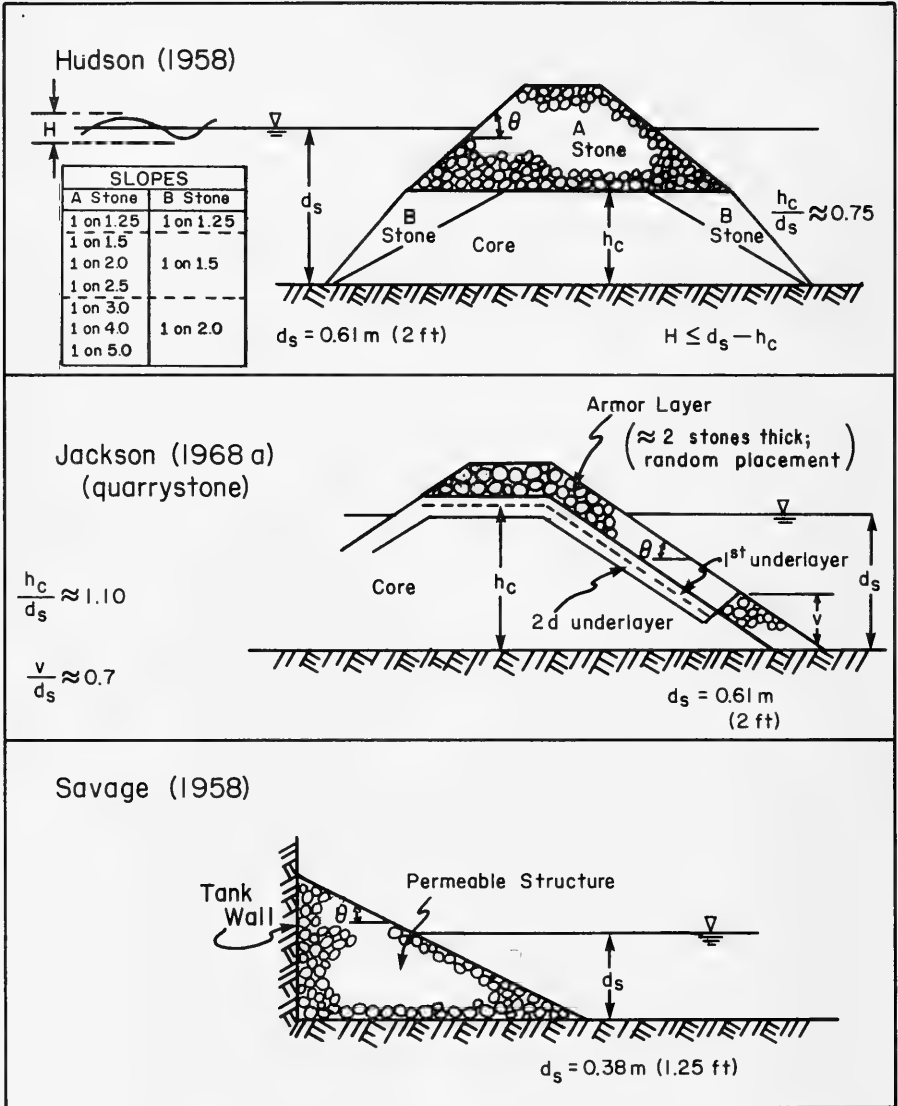
Figure 24. Permeable rubble-mound structures.
