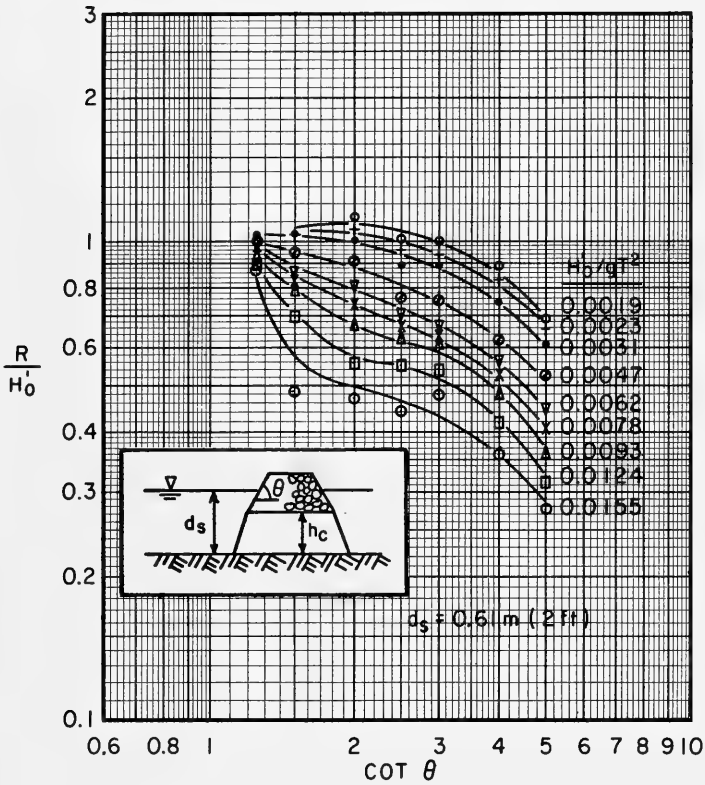
Figure 26. Quarystone rubble-mound runup; d_s/H_0' = 5.0 ; H_0'/k_T = 2.7 ; h_c/d_s \approx 0.75 (after Hudson, 1958).
