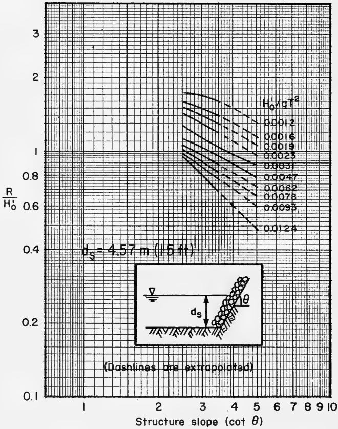
Figure 40. Relative runup for riprap slopes; d_s/H_0' = 5.0 ; H_0'/k_r \approx 3.15 (after Ahrens, 1975a).
