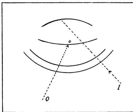
FIG. 35.—Vacuole in the anterior lens-cortex viewed by retroillumination.
