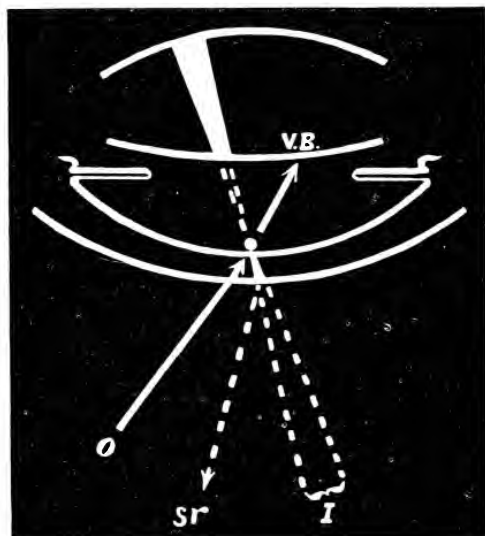
FIG. 15.—Illumination-beam traversing cornea and lens; observation of a spot of K.P. by direct illumination.
