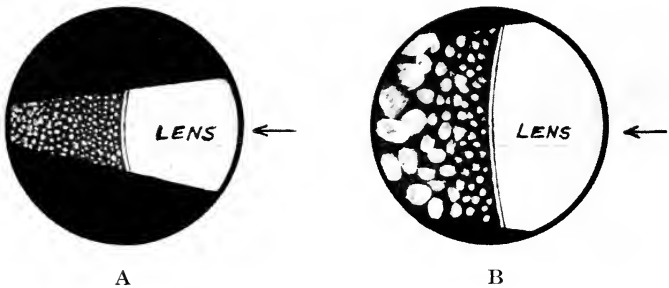
FIG. 51.—Pathological masses in the vitreous fluid seen by (A) low and (B) high magnification.
