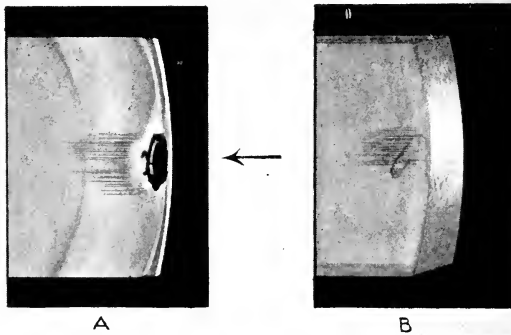
FIG. 49.—Wide slit-beam (B) and narrow slit-beam (A) through anterior region of the lens showing pathological dissolution of a small area of the cortex.
