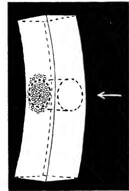
FIG. 25.—View of the endothelial face of the cornea by D.I.S.R.
