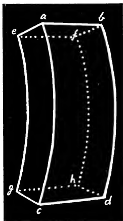
FIG. 17.—Edges and faces of the illuminated corneal block.
