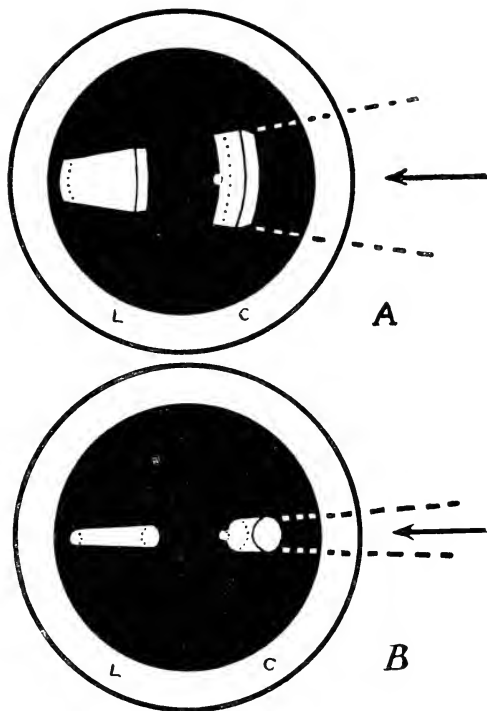
FIG. 16 —A: Wide slit-beam; B: Small circular beam, illuminating a spot of K.P. on the deep face of the cornea. Beam in cornea (c) and lens (l).
