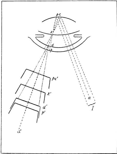
FIG. 22.—Observation along the axis of the specularly reflected beam from the posterior lens-capsule.
