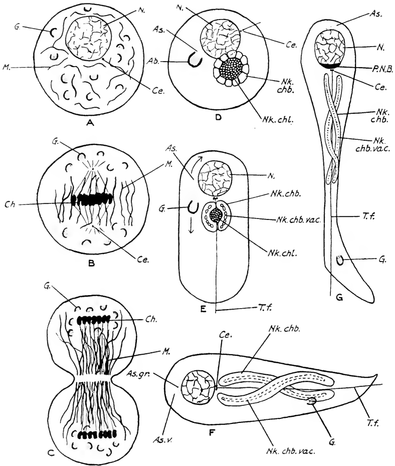
FIG. 64.—Diagram of spermatogenesis in the hemiptera (after Bowen (3, 6 and 7)). For details of lettering see Fig. 63. In addition: As.v. , acrosomal vesicle; As.gr. , acrosomal granule; Nk. , Nebenkern; Nk.chl. , central chromophilic mass of Nebenkern; Nk.chb. , cortical chromophobic mass of Nebenkern; Nk.chb.vac. , vacuoles in chromophobic cortex of Nebenkern.
