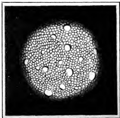
FIG. 38.—Intraepithelial vacuolation of the cornea by retroillumination.
