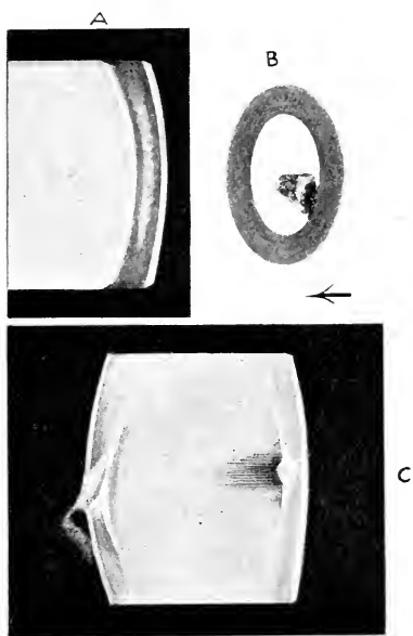
FIG. 50.—A, Slit-beam showing a plaque-like change in the anterior lens-cortex. B, The same viewed as an opacity by the ophthalmoscope. C, Pathological changes in the anterior and posterior lens-cortex.
