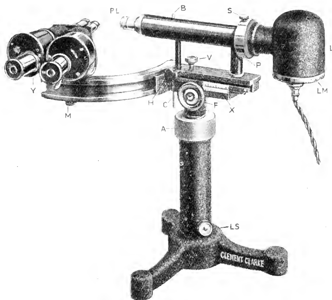
FIG. 14.—Fincham pattern of Gullstrand slit-lamp and Czapski binocular microscope, made by Messrs. Clement Clarke & Co., Ltd.
