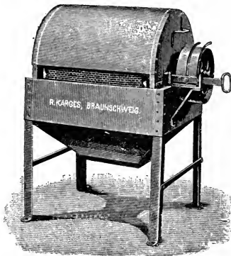
FIG. 14.—Carrot-cleaning machine.
