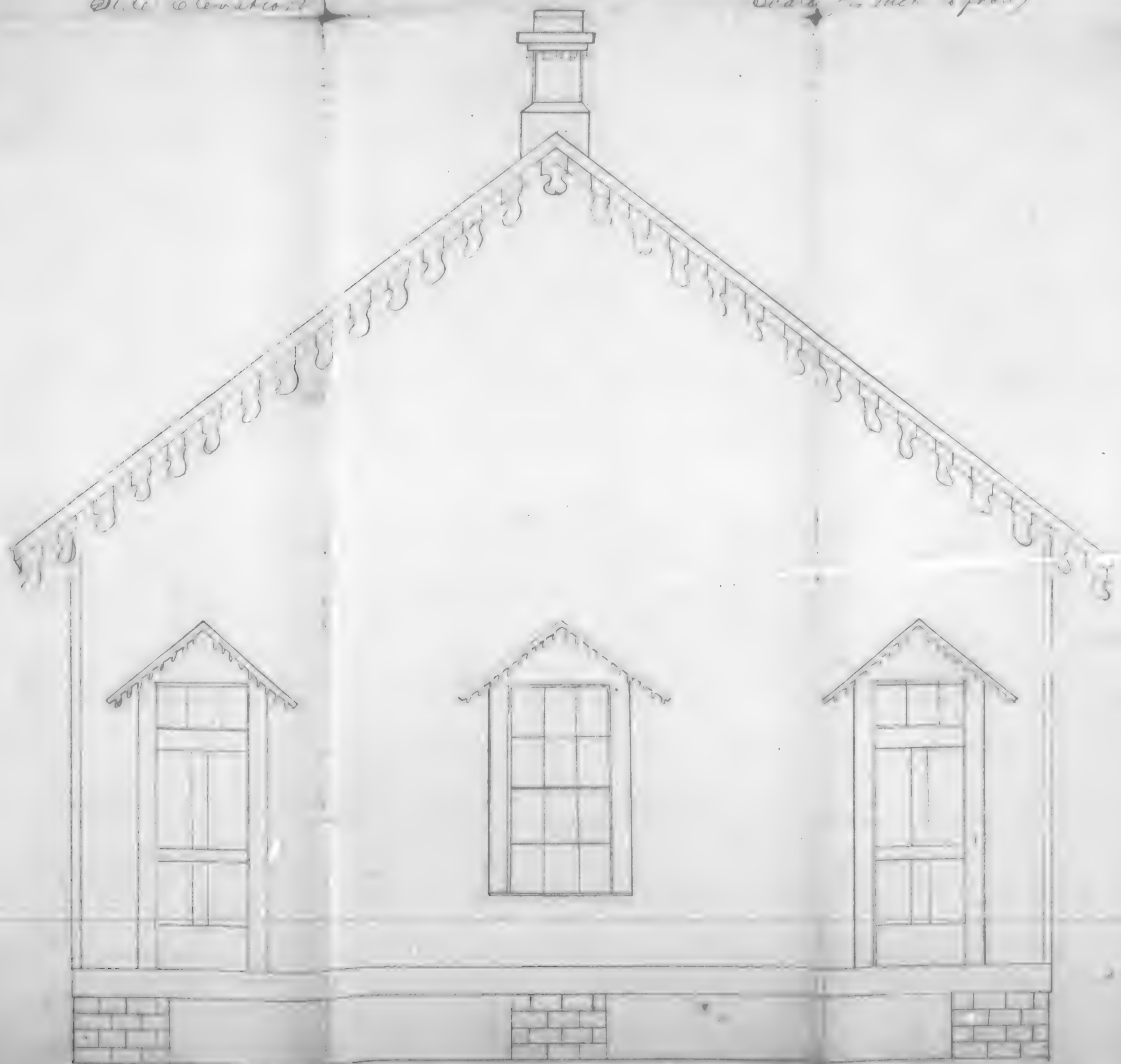
Front Elevation
