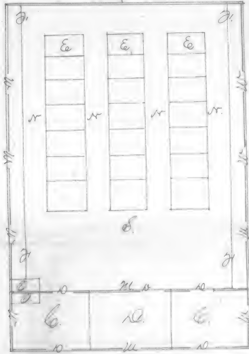
Plan of School House at ... 24' 36'
