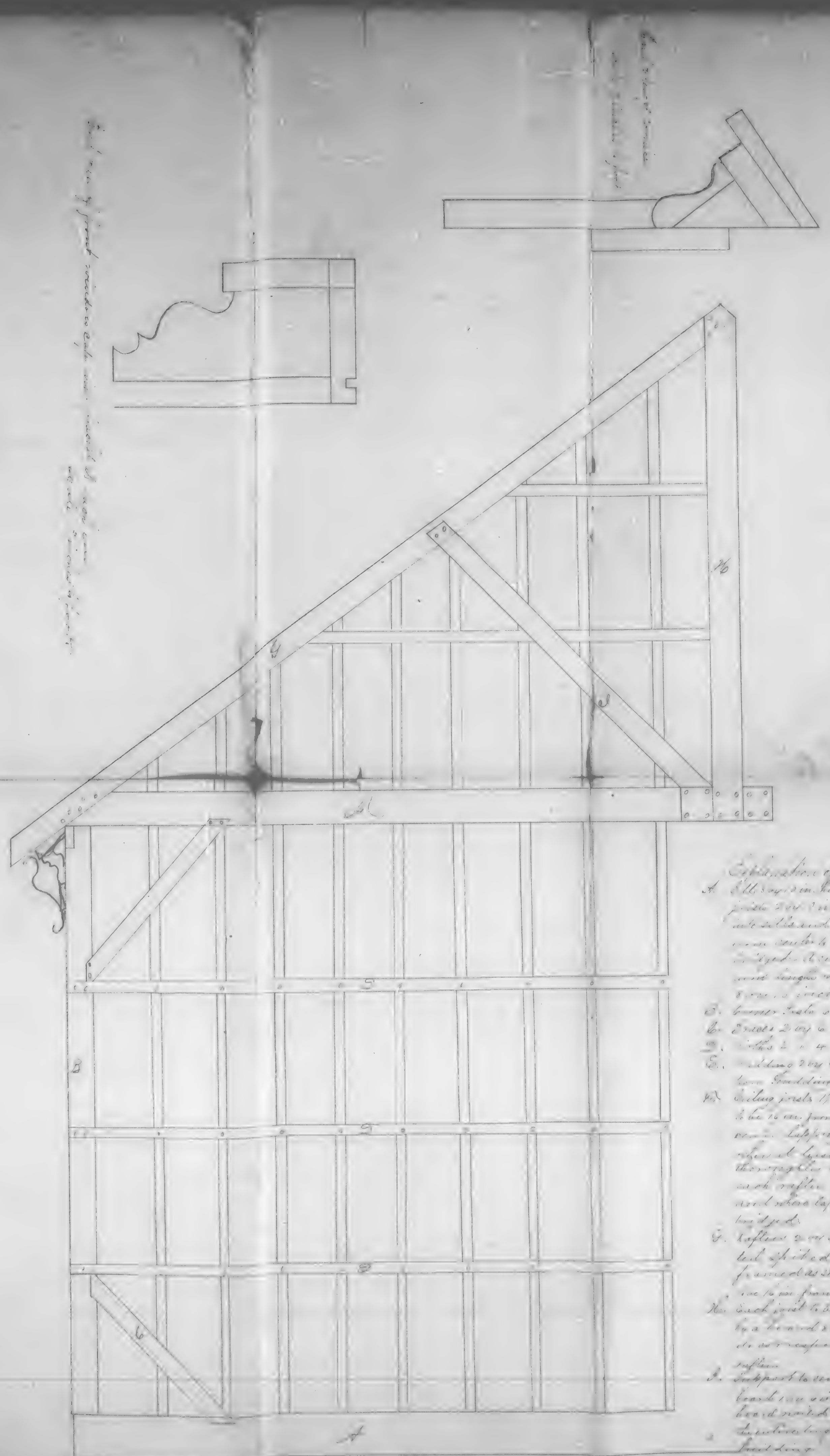
Sections of Rafters
