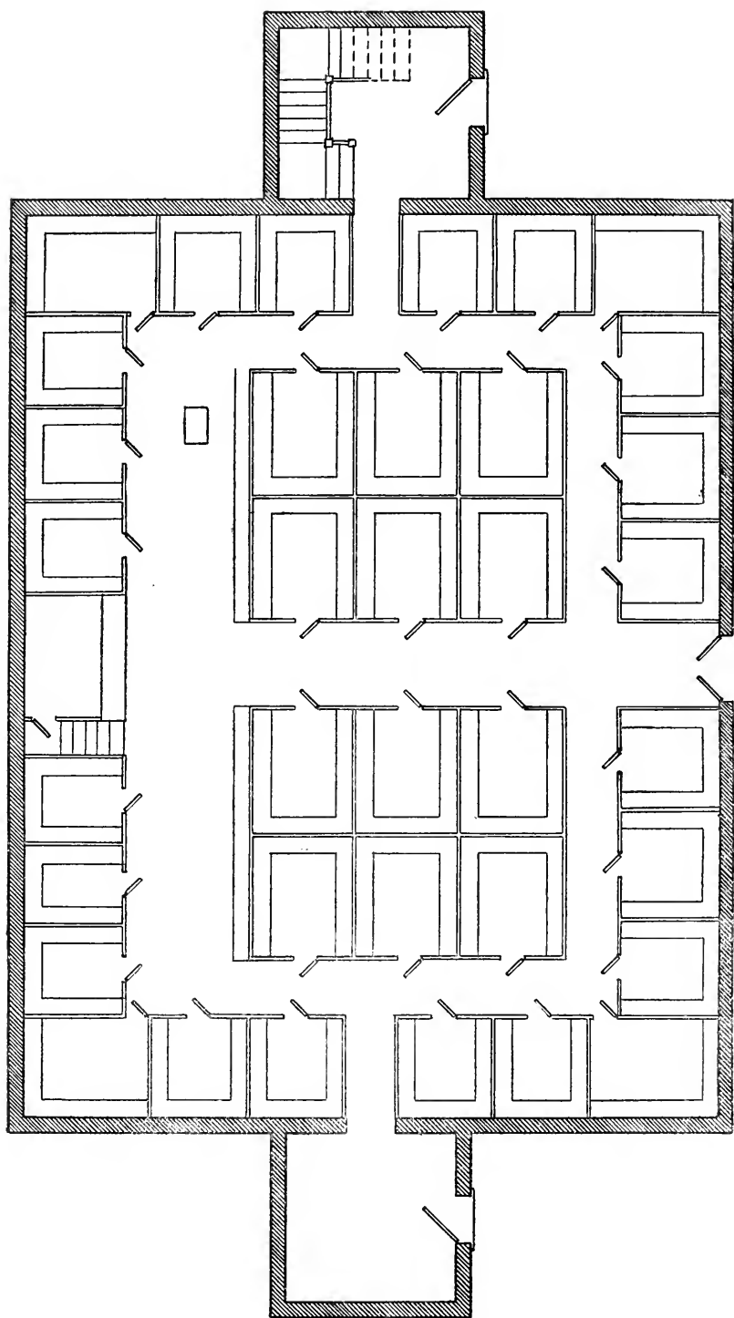
PLAN OF ROCKINGHAM MEETING HOUSE, (Scale 3/32 in. to 1 ft.)
