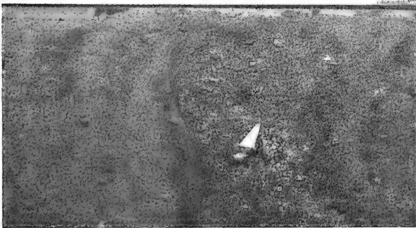
Figure 22. Photo of sand in core 93; scale in meters from top of core. Arrow points to top of core.
