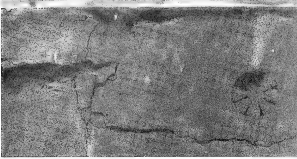
Figure 23. Photo of muddy sand in core 92; scale in meters from top of core. Arrow points to top of core.
