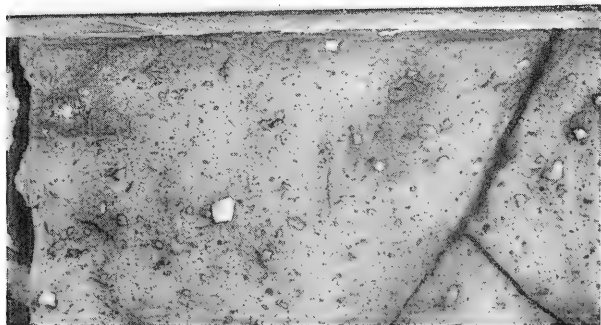
Figure 15. Photo of basal till in core 79; scale in meters from top of core. Arrow points to top of core.
