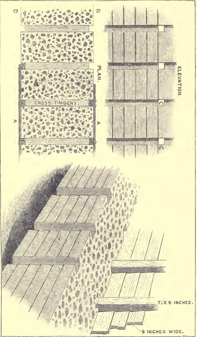
Fig. 3. Method used in Rome of casting concrete walls inside wooden boarding.
