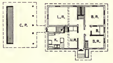
REVERSED FLOOR PLAN
