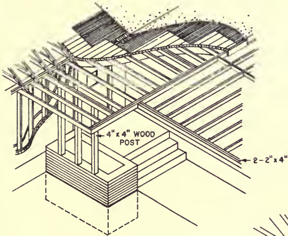
ROOF FRAMING
