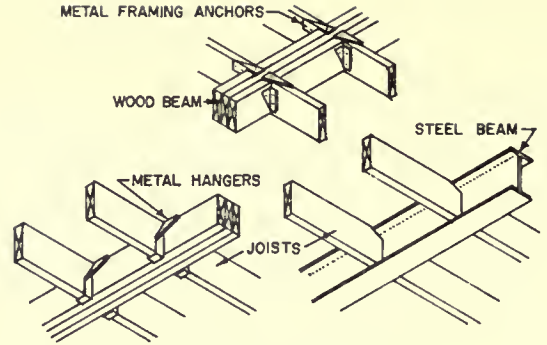
CONCEALED BEAMS
