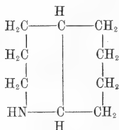
Decaidrohincholina o chinolanina
