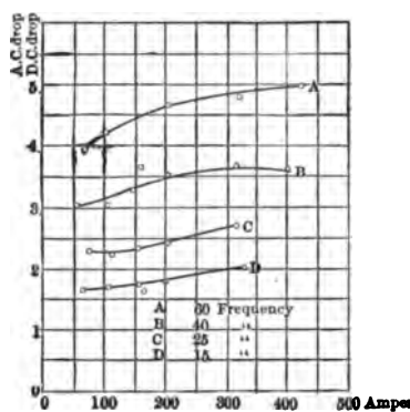
Fig. 156. — Variation of Ratio \frac{A.C. \text{ Drop}}{D.C. \text{ Drop}} Single Rail and Single Track.
