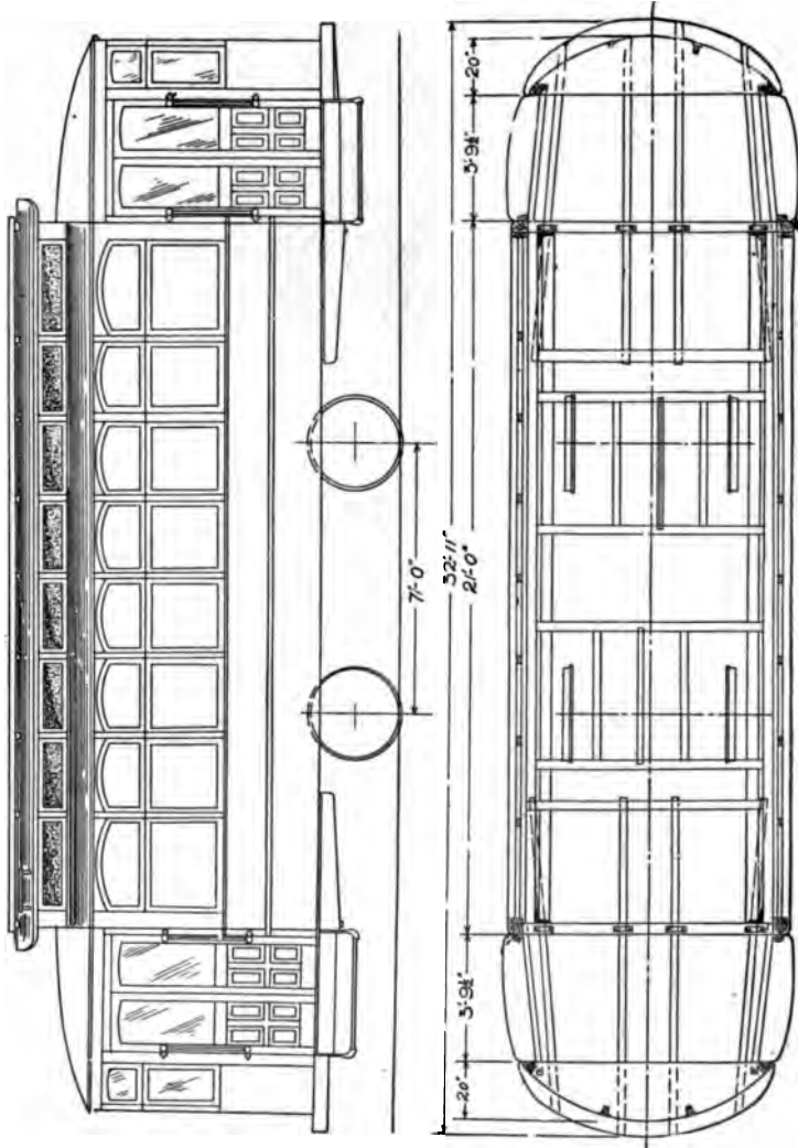
Fig. 4. — General Drawing of the Sing'e-Truck Car.
