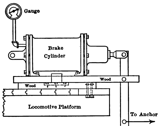
Fig. 105.—Oil Dynamometer. Industrial Locomotive.
