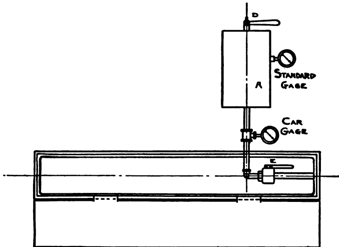
Fig. 80. — Connection for Calibrating Car Gages.
