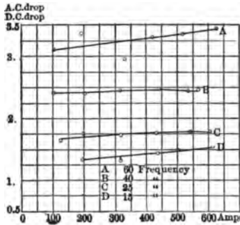
Fig. 140.—Variation of Rates A.C. Drop with D.C. Drop Total Amperes. Double Track and Trolley.
