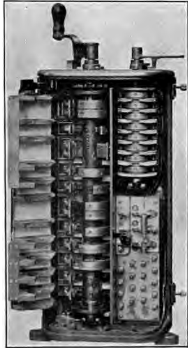
Fig. 16A. —General Electric Company, K. 28, Controller.
