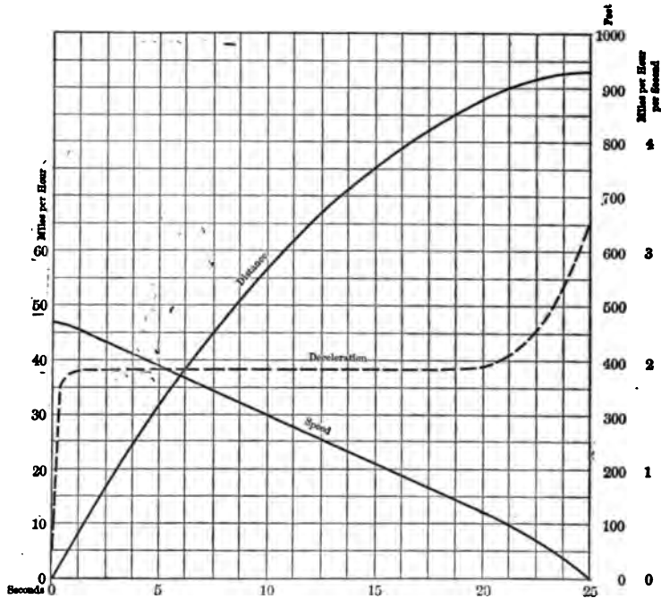
Fig. 91. — Speed and Distance Data. Test No. 31.
