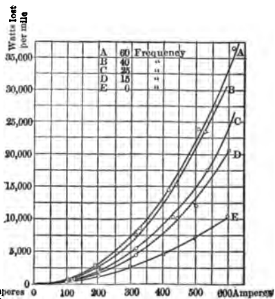
Fig. 143.—Variation of Watts Lost per Mile with Total Amperes. Double Track.
