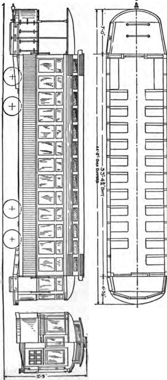
Fig. 12. — General Drawing of Double-Track City Car.
