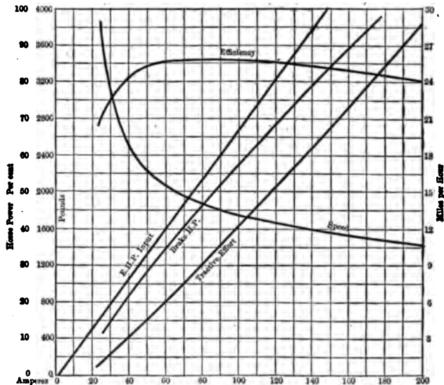
Fig. 26.—Curves Showing the General Performance of the Westinghouse, No. 58 Motor with Gear Ratio 18 to 64.
