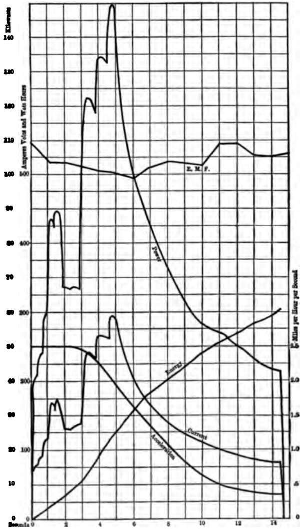
Fig. 57. — Electrical Data of Test No. 12.
