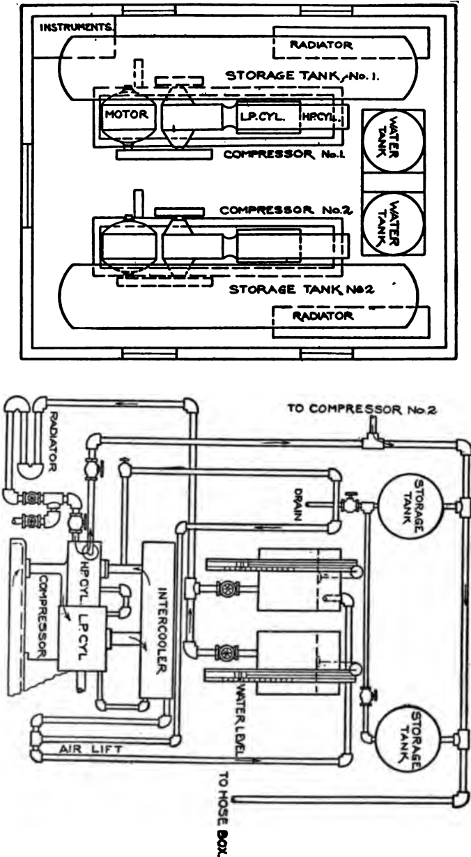
Fig. 75.—Tower Grove Park Station of the St. Louis Transit Company.
