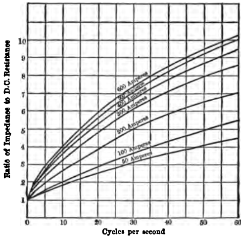
Fig. 124. — Frequency Ratio Curves, 56 lb. Rail, A. C. Rail Tests.
