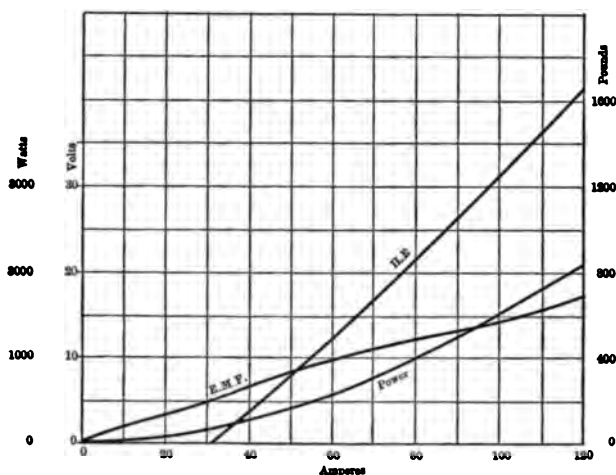
Fig. 110.—General Data, Industrial Locomotive Tests. Run No. 5.
