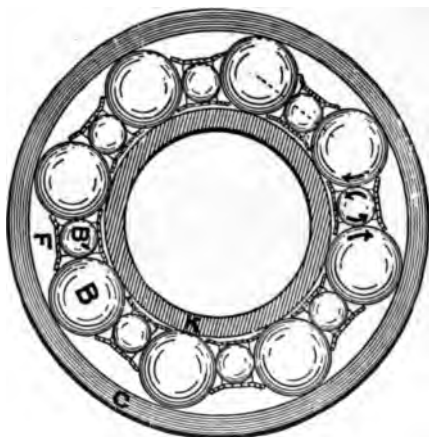
Fig. 185.—Pressed Steel Duct-Ring of Chapman Double-Ball Bearing.
