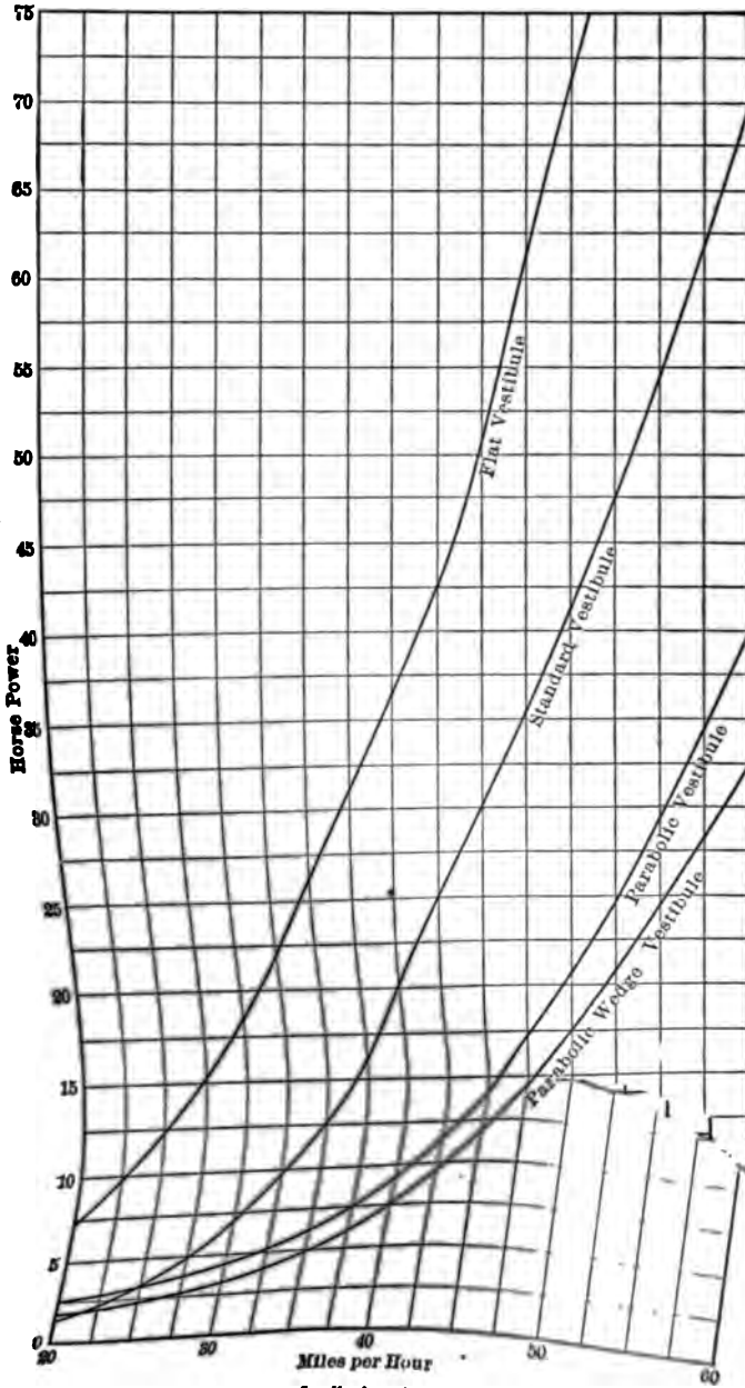
Fig. 298. — Pressure Power Curves for Various Vestibules — Air Resistance Tests.
