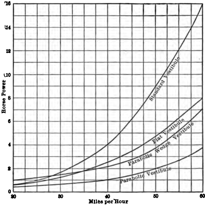
Fig. 204.—Suctions—Power Curves for Various Vestibules—Air Resistance Tests.
