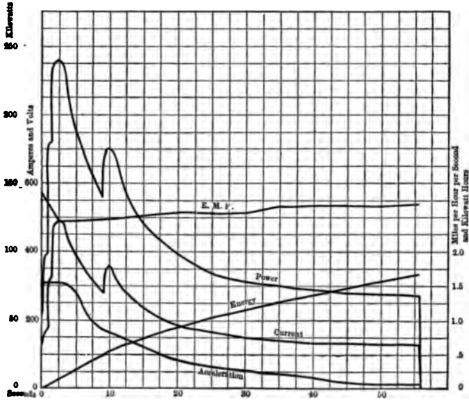
Fig. 71.—Electrical Data of Test No. 18.
