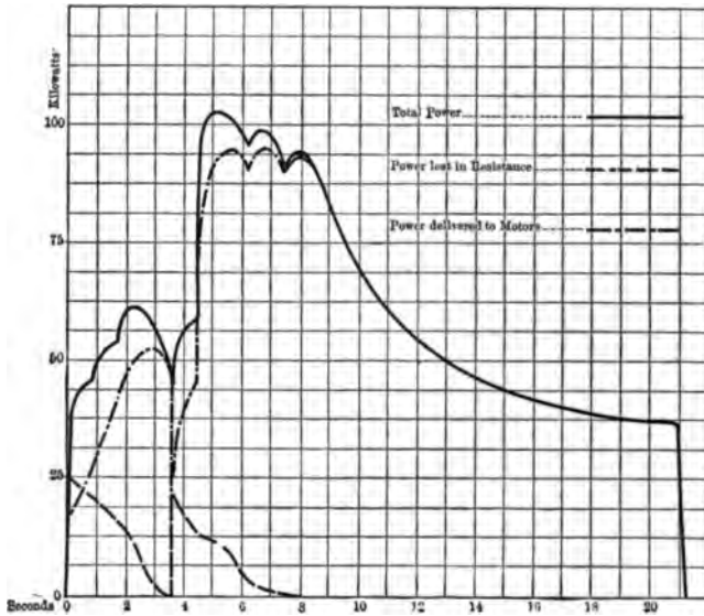
Fig. 32. — Division of Power, Test No. 2, Sept. 24, 1904.
