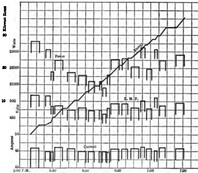
Fig. 82. — General Electrical Data of Test No. 21.
