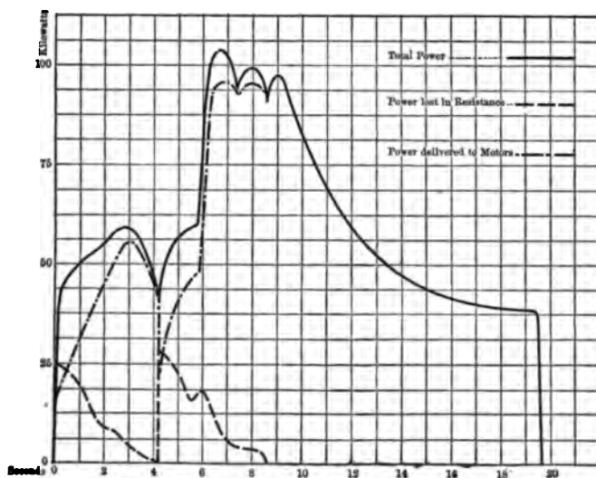
Fig. 41. — Division of Power in Test No. 5, Oct. 7, 1904.
