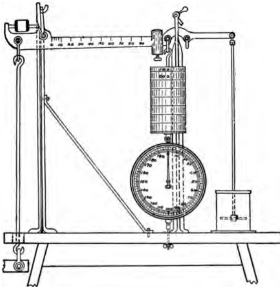
Fig. 101. — General Sketch of Scale Mechanism Used with Dynamometers.
