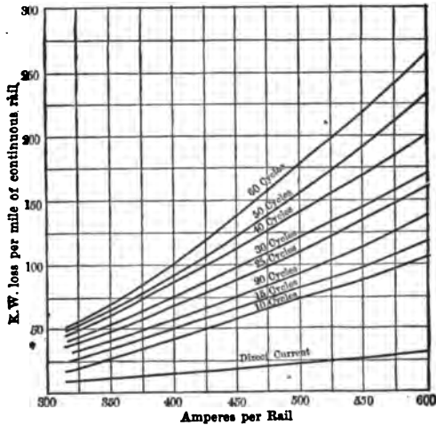
Fig. 127.— Current Power Curves, 56 lb. Rails, A. C. Rail Tests.
