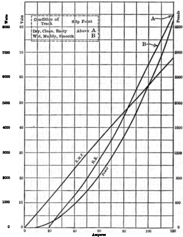
Fig. 109.—General Data, Industrial Locomotive Tests. Run No. 4.
