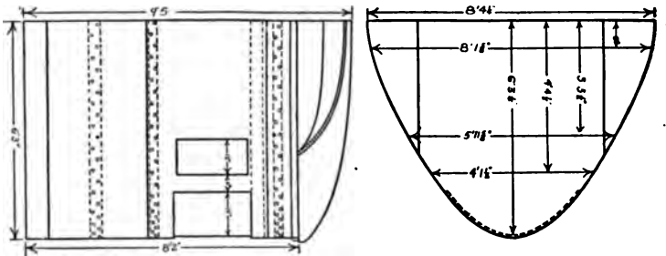
Fig. 173. — Sketch of "Parabolic" Movable Vestibule.
