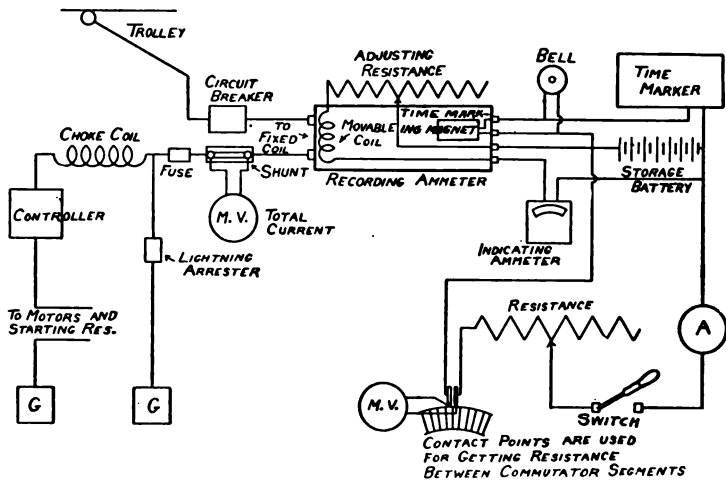
Fig. 44. — Diagram of Connections, Service Tests of Double-Track City Car.
