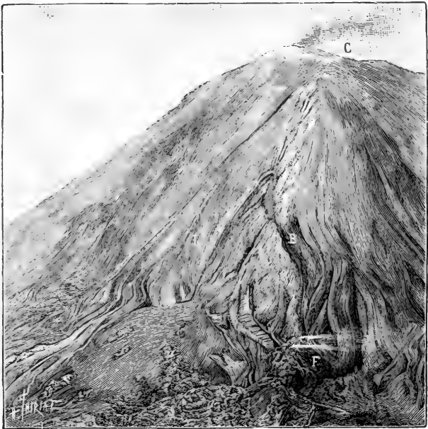
C , crater plain and cone of eruption; B , rift, marked half-way down by an irregular crateriform pit produced by the explosion at 5.30 P.M.; L , tongues of lava that issued from last-mentioned pit; F , main outpour of lava with fumaroles.
