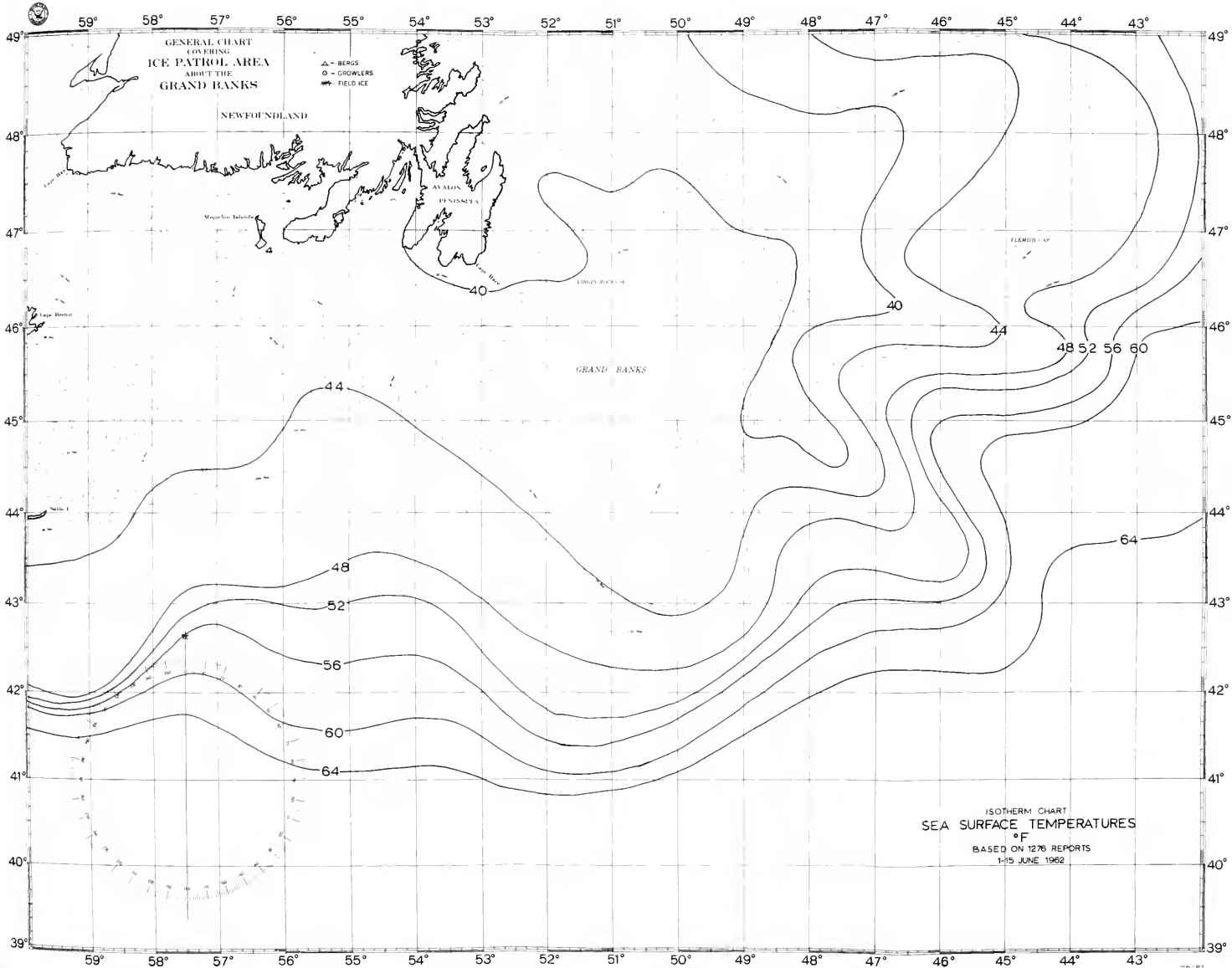
FIGURE 7.—Surface isotherms for the period 1-15 June 1962.
