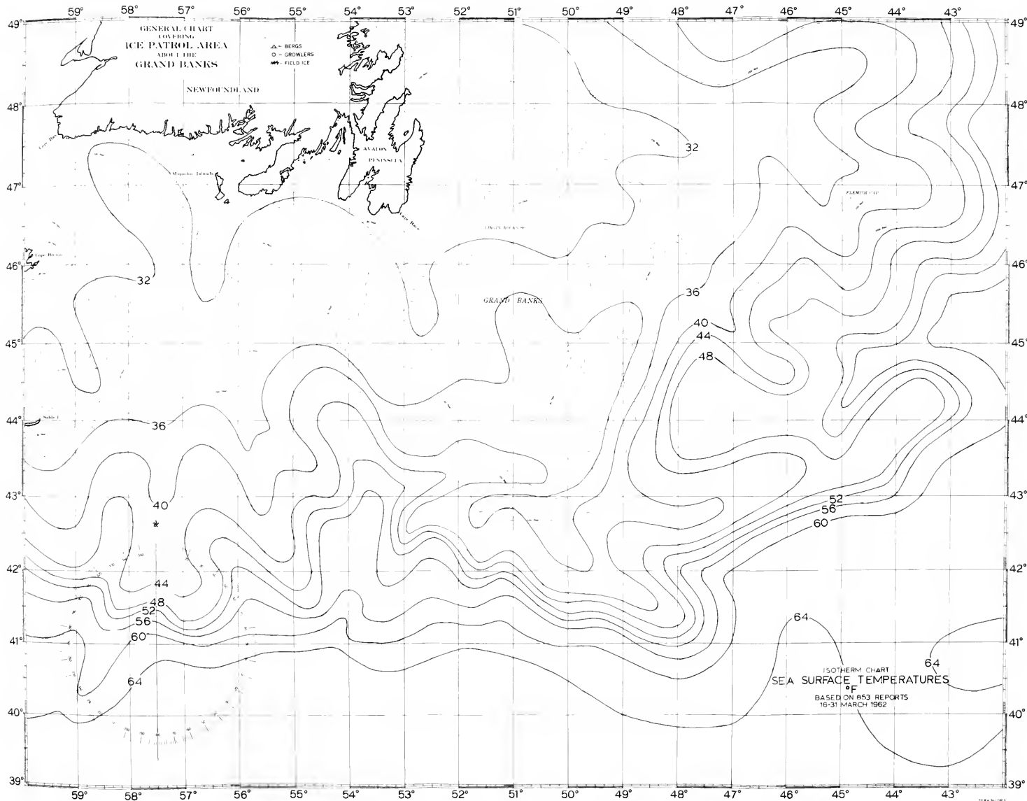
FIGURE 2.—Surface isotherms for the period 16-31 March 1962.
