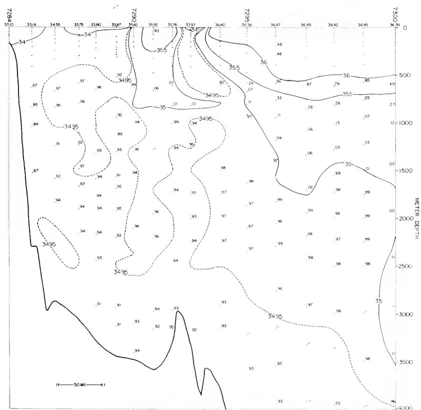
FIGURE 34.—Temperature distribution along meridional section at 50^{\circ}15' W., from data collected 7-10 April 1960.
