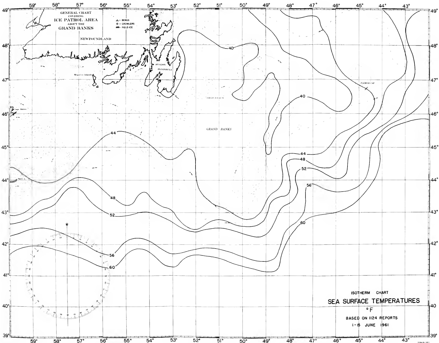
FIGURE 8.—Surface isotherms for the period 1-15 June 1961.
