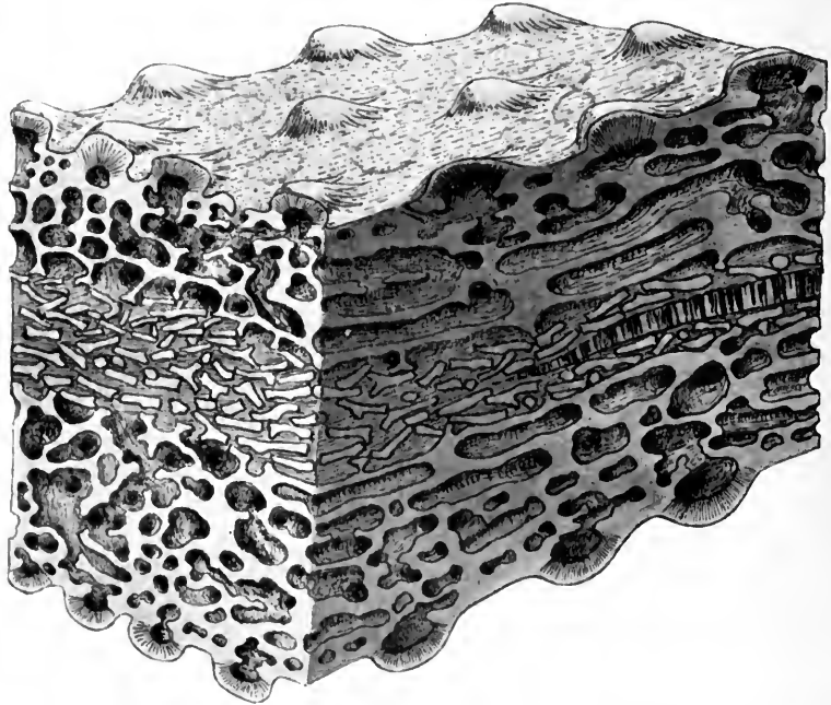
Fig. 6. Sketch showing the structure of the dermal skeleton in Drepanaspis Gemündenensis , SCHLËTER. The section is made through one of the upper and one of the lower body plates. The latter are so greatly compressed that the inmost layer of the skeleton is crushed. At the extreme top and bottom we see the denticles with their wide pulp cavities and fine dentine tubules; below them is the vascular canal system.
