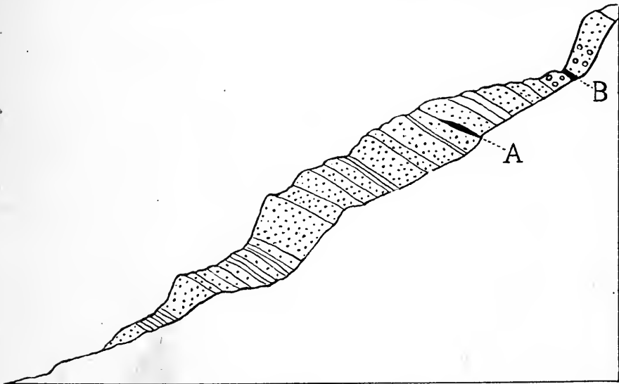
Fig. 4. Section at Bregnekløften after PER SCHEI. The strata mainly consist of quartz sandstone and sandy schists. At A, plant fossils. At B, anthracitic coal, about 2—3 cms. in thickness. Conglomerate at the top. The strata are somewhat over 100 m. in thickness.
