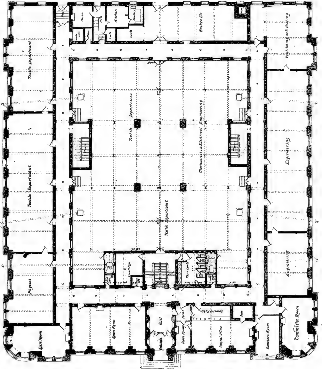
GROUND PLAN
