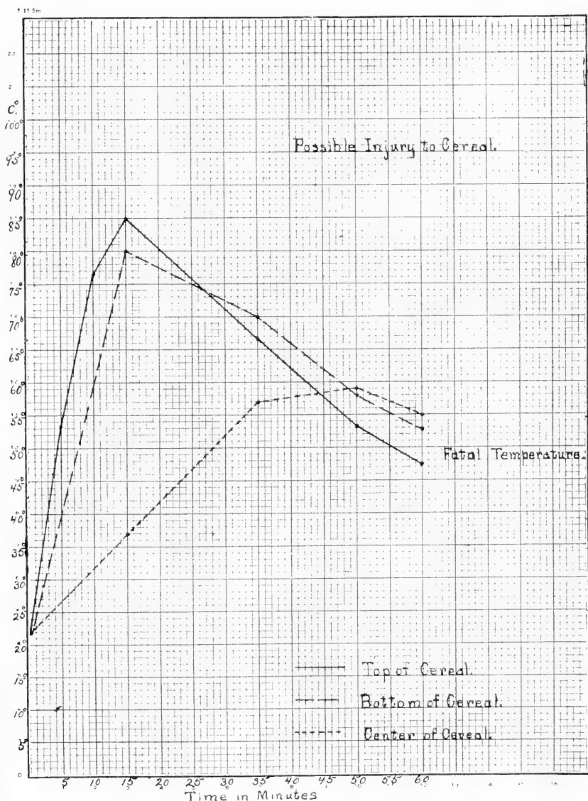
Fig. 15. Curves showing the rise of temperature in the top, center, and bottom of a pan of cereal heated in a gas oven. The oven was cold at the start, the cereal was two inches deep in the pan, and the fire was as low as it would burn for fifteen minutes.
