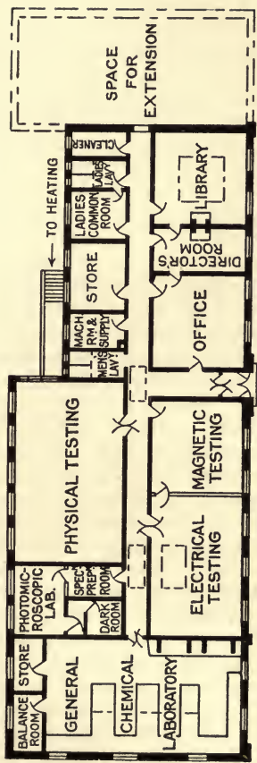
PLAN. Scale of Feet. 10 5 0 10 20 30 40 50
