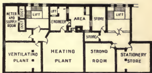
BASEMENT PLAN
