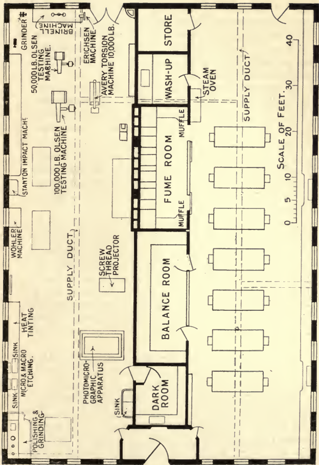
FIG. 14. RESEARCH BUILDINGS, METROPOLITAN-VICKERS ELECTRICAL CO., LTD., MANCHESTER Chemical and Mechanical Testing Laboratories
