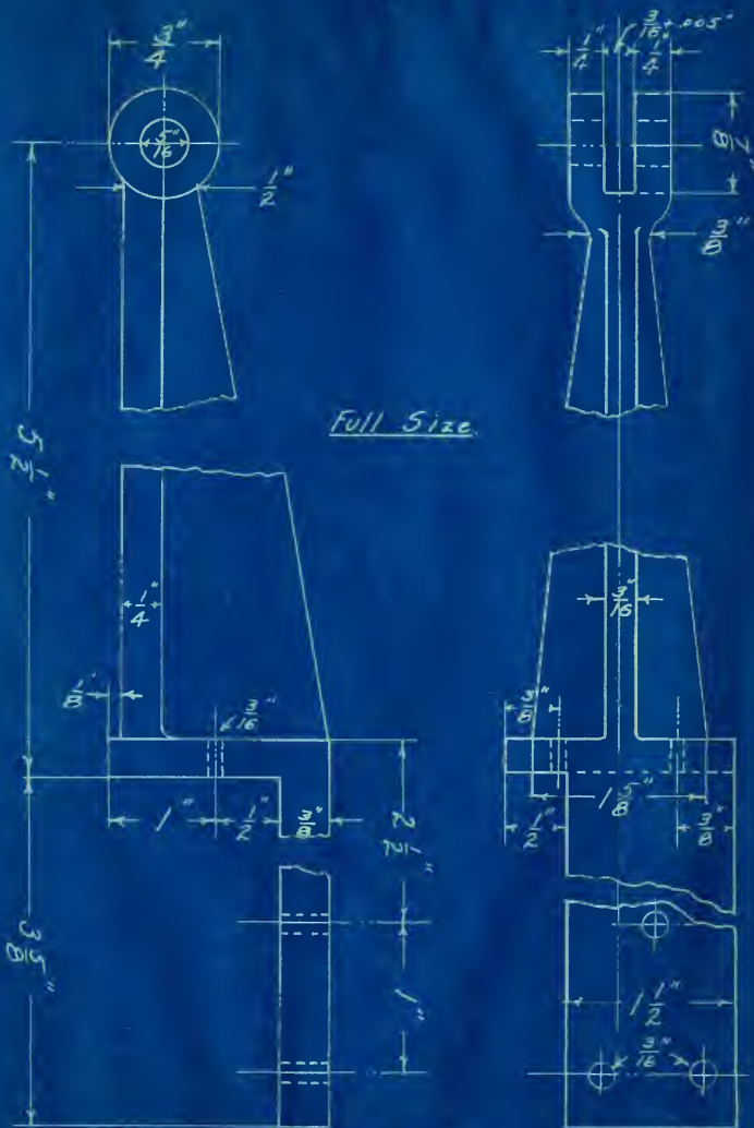
FULCRUM FOR RECORDING DEVICE.
