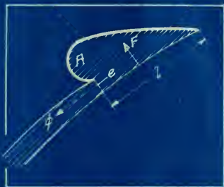
Fig. 6- Showing Forces Acting at Bead of Tire.
