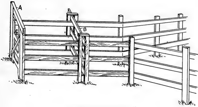
Fig. 263. Cattle "Chute."
