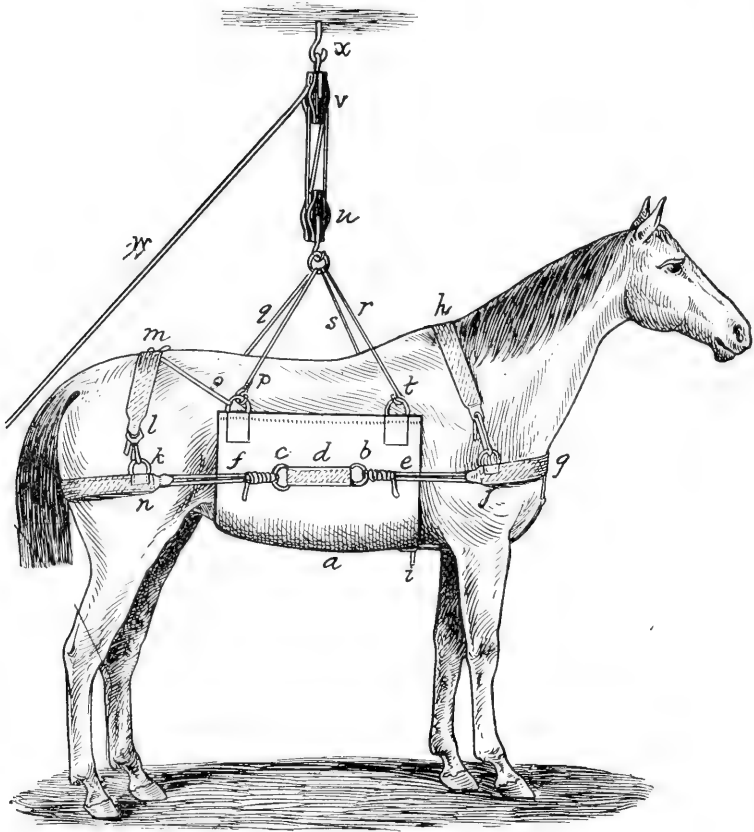
Fig. 77. French Sling.
