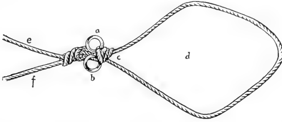
Fig. 152. Collar Loop of Hayes' Improvised Casting Ropes.
