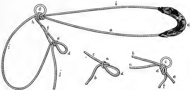
Fig. 175. Magner's Rope Casting Rig.
