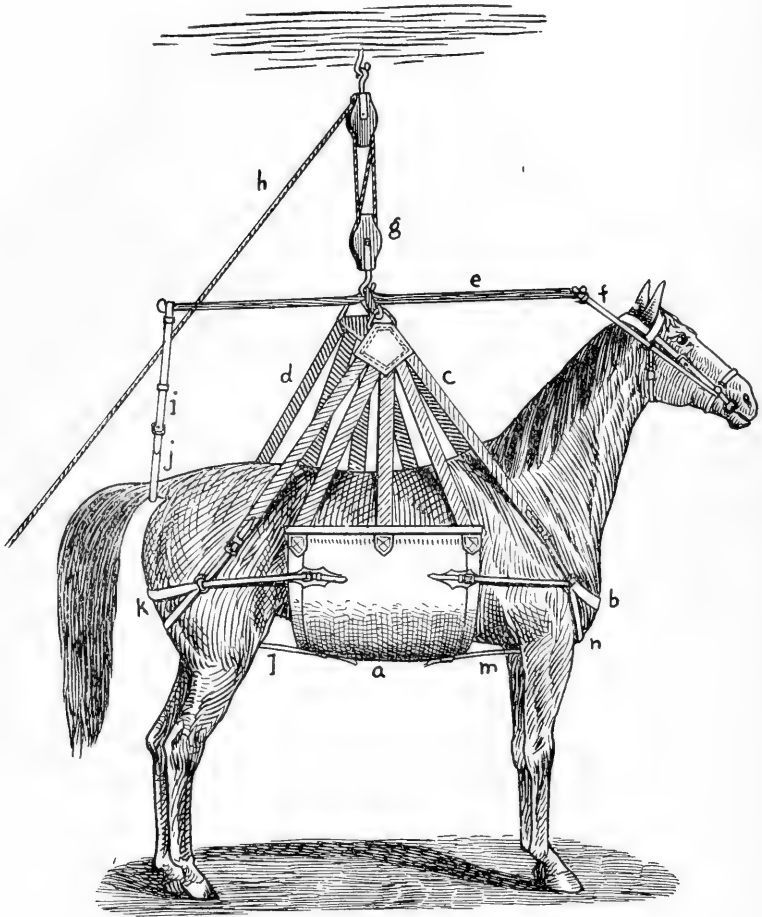
Fig. 75. German Sling.
