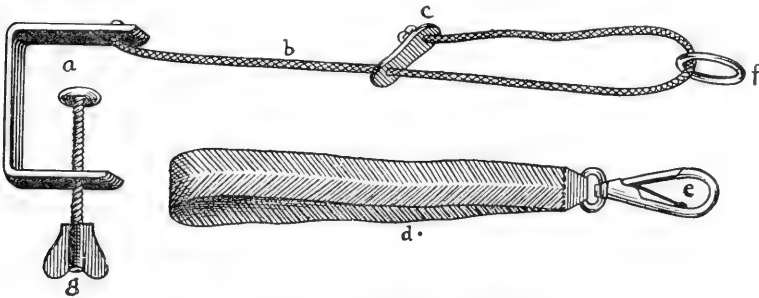
Fig. 279. Hobday's Hobbles.
