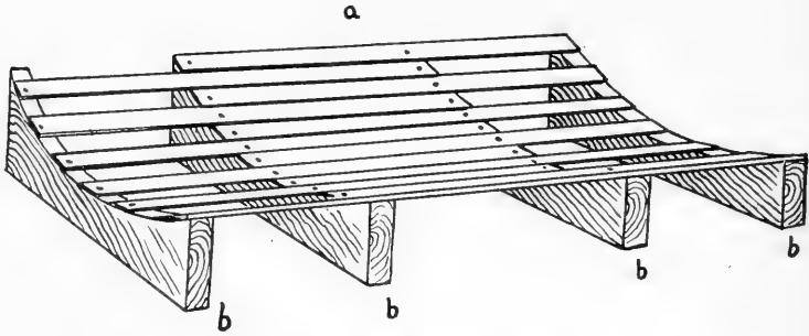
Fig. 285. Extension Grate.
