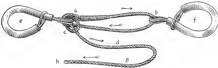
Fig. 82. James' Cross Hobbles.
