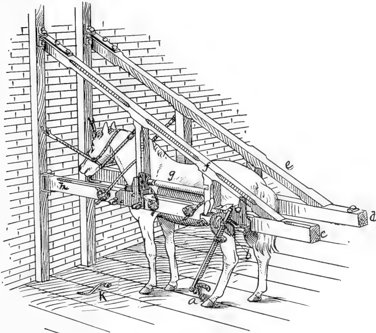
Fig. 61. Barcus Stocks.
