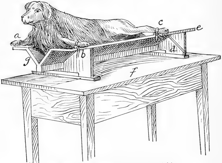
Fig. 287. MacQueen's Operating Table.
