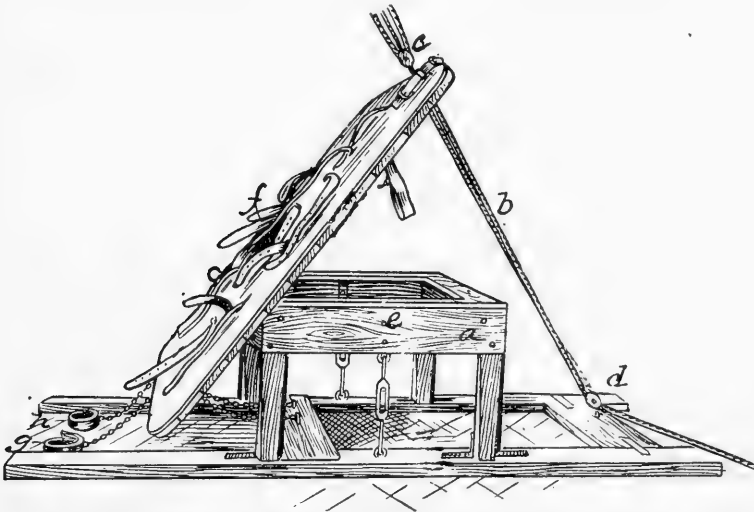
Fig. 193. Hodgson & Magee's Table, Oblique Position, Side View.
