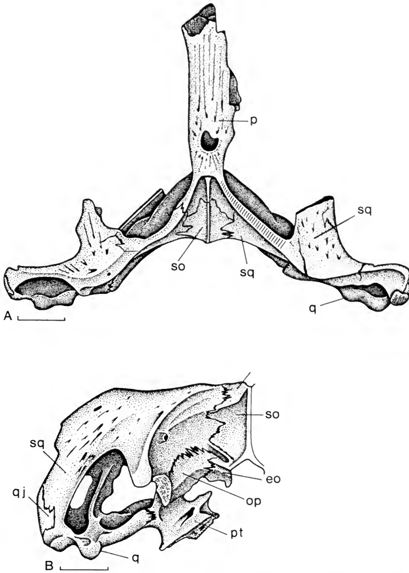
FIG. 46. Nothosaurus sp. (MB R. 1775); lower Muschelkalk, Freyburg/Unstrut. Skull fragment. A , Dorsal view; B , occipital view. Scale bar = 20 mm. Abbreviations: eo, exoccipital; op, opisthotic; p, parietal; pt, pterygoid; q, quadrate; qj, quadratojugal; so, supraoccipital; sq, squamosal.
