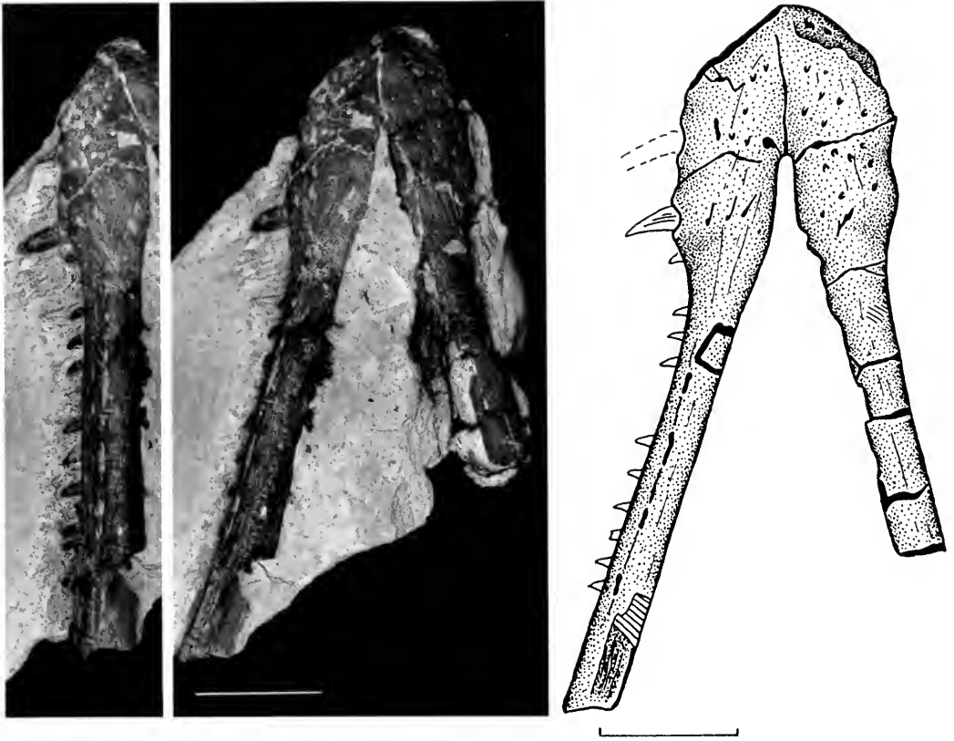
FIG. 29. Nothosaurus (Oligolyck) hecki v.Frisch (holotype; Ha 12/41); lower Muschelkalk, Halle/Saale. Scale bar = 10 mm.
