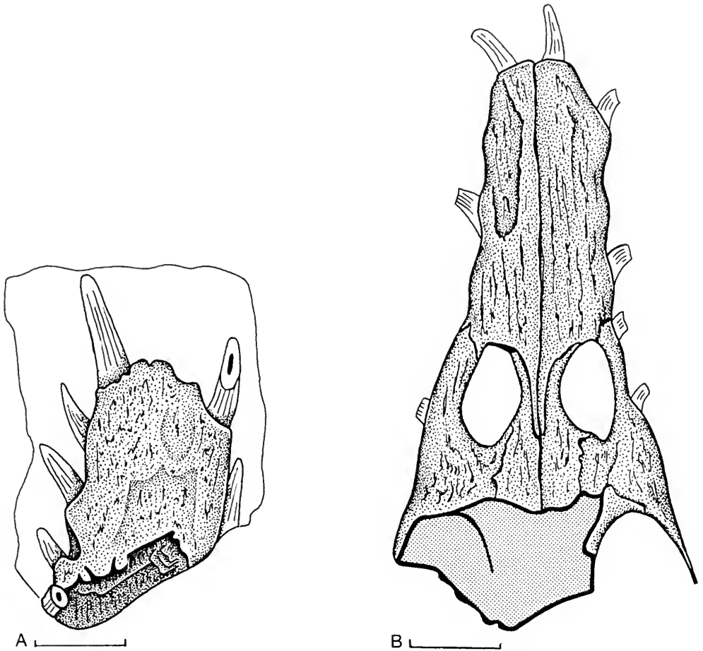
FIG. 51. Nothosaurus cuvieri Quenstedt; lower Keuper, Hoheneck near Ludwigsburg. Partial skulls. A, SMNS, uncatalogued (original of Fraas [1896: 12], and Schmidt [1928, Fig. 1114]); B, SMNS 17291 (undescribed specimen). Scale bar = 20 mm.
