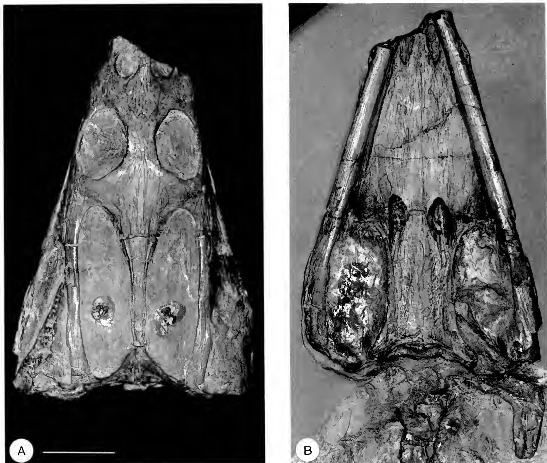
FIG. 31. Nothosaurus raabi Schröder (holotype; MB I. 007.18); lower middle Muschelkalk, Rüdersdorf. A, The skull in dorsal view; B, the skull in ventral view. Scale bar = 20 mm.
