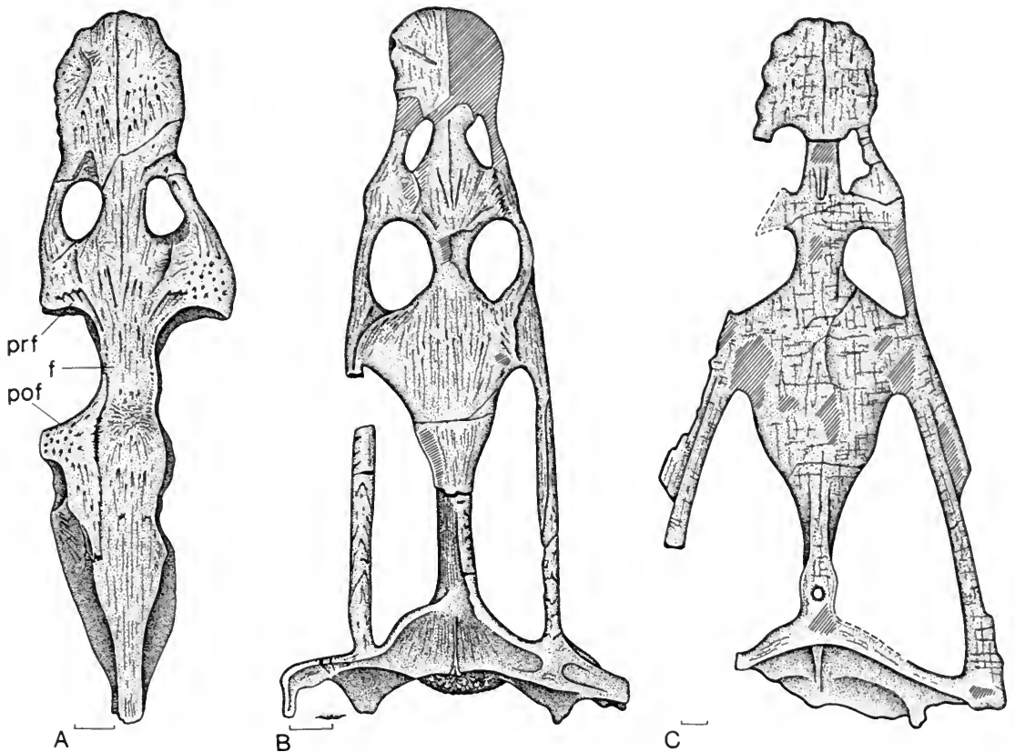
FIG. 3. A , Metal cast of the skull of Nothosaurus andriani Meyer (SMNS 7860b; original of Fraas, 1896 ["Allmendinger" specimen]); upper Muschelkalk, Crailsheim. B , Nothosaurus angustifrons Meyer and Plieninger (holotype; SMNS 51972); upper Muschelkalk (mo 2 ), Crailsheim. C , Nothosaurus chelydrops Fraas (holotype; SMNS 7162); lower Keuper, Hoheneck near Ludwigsburg. Scale bar = 20 mm. Abbreviations: f, frontal; pof, postfrontal; prf, prefrontal.
