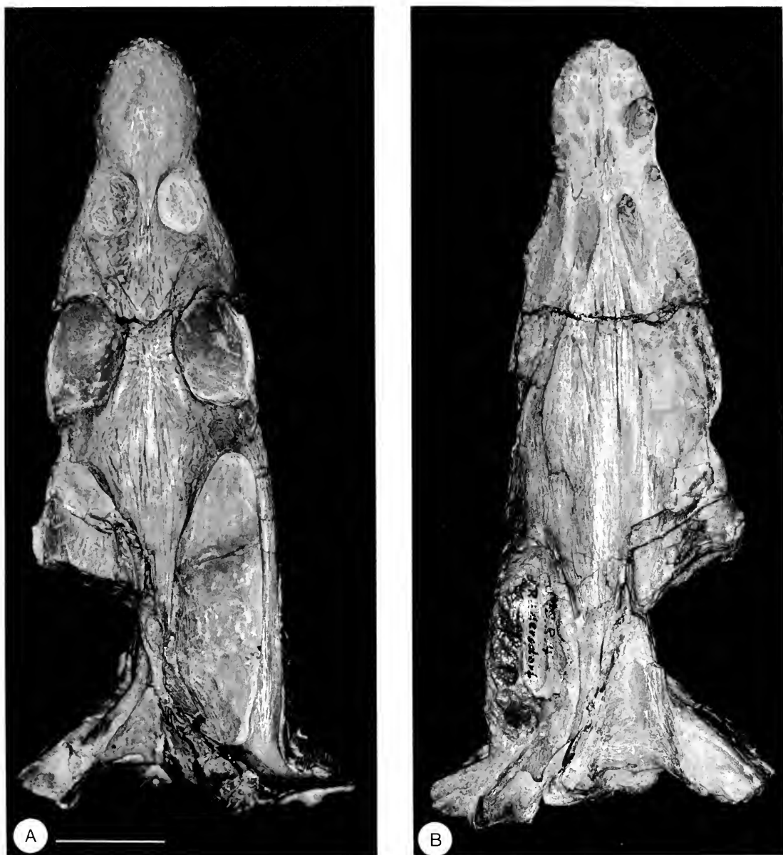
FIG. 33. Nothosaurus procerus Schröder (holotype; MB R. 4); lower middle Muschelkalk, Rüdersdorf. A , The skull in dorsal view; B , the skull in ventral view. Scale bar = 20 mm.
