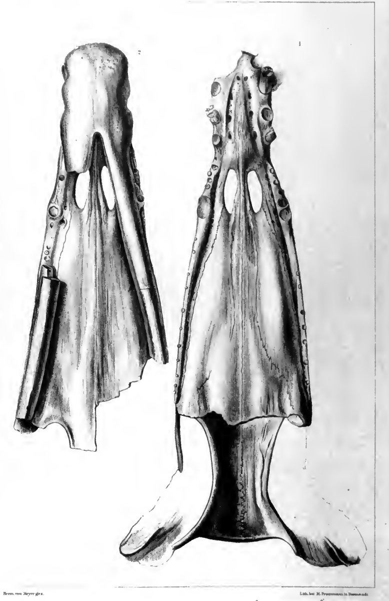
FIG. 48. Nothosaurus mirabilis Münster, paratype. Upper Muschelkalk, Bayreuth. Plate 3 of Meyer, 1847–1855 (SMNS negative no. 9172).
