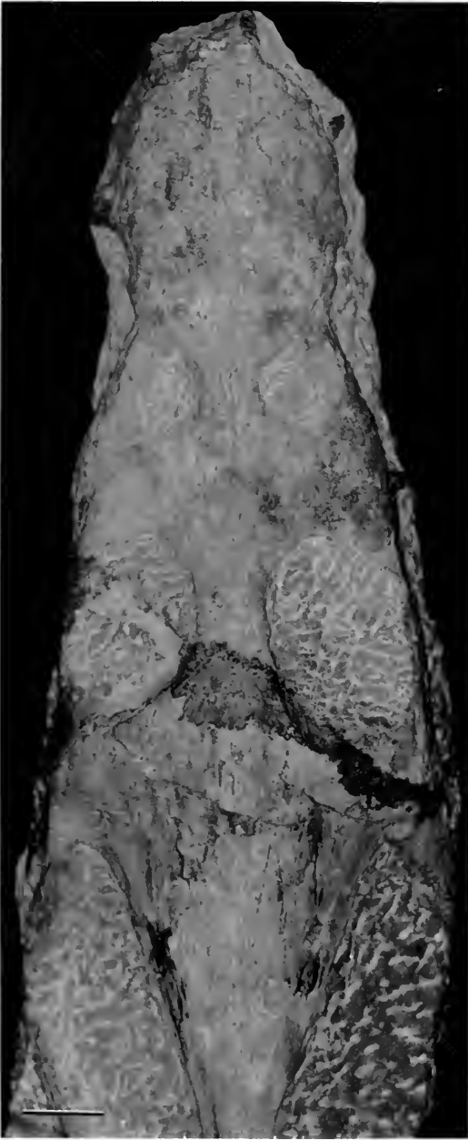
FIG. 5. Nothosaurus angustifrons Meyer and Plieninger (SMNS 8872; original of Fraas, 1896 [“Blezinger” specimen]); upper Muschelkalk, Crailsheim. Anterior part of skull in dorsal view. Scale bar = 20 mm.
