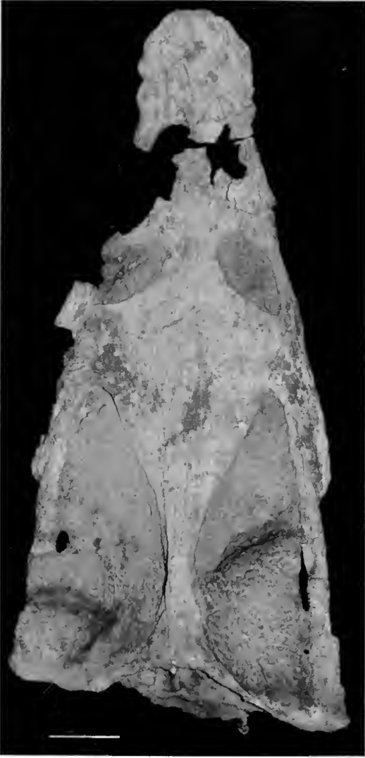
FIG. 7. Nothosaurus chelydrops Fraas (holotype; SMNS 7162); lower Keuper, Hoheneck near Ludwigsburg. The skull in dorsal view. Scale bar = 50 mm.
