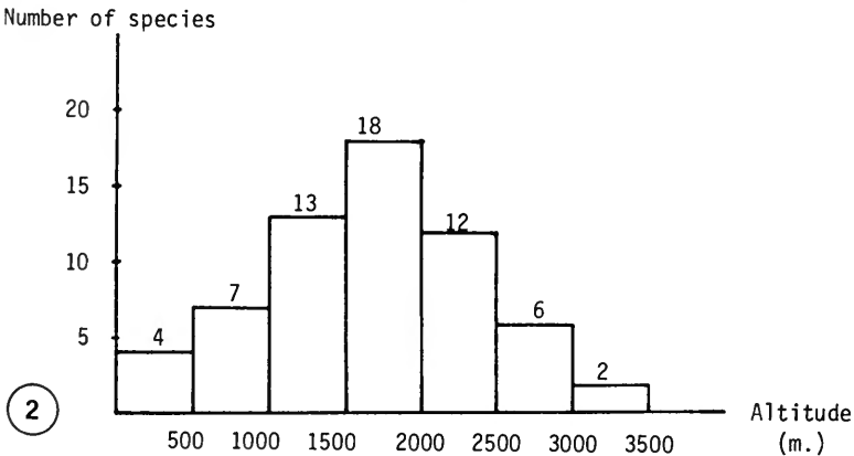
FIG. 2. Altitudinal distribution of Mexican and Central American Saurauia . (69.3 per cent of the species are found at altitudes of 1,000-2,500 m.)
