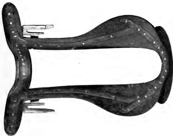
Fig. 124. View of under surface of Saddle Tree, with Bar Plates.
