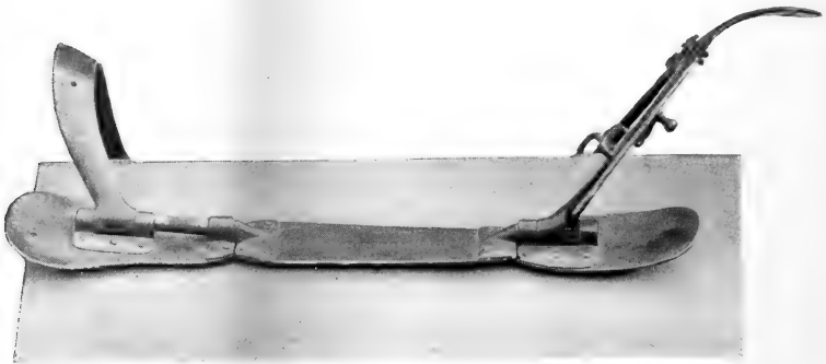
Fig. 133. Side View of Austrian Officer's Jointed Saddle Tree.
