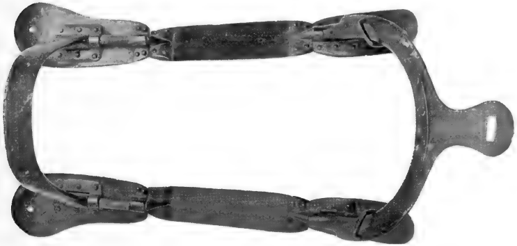
Fig. 134. Plan of Austrian Officer's Jointed Saddle Tree on a Broad-backed Horse.
