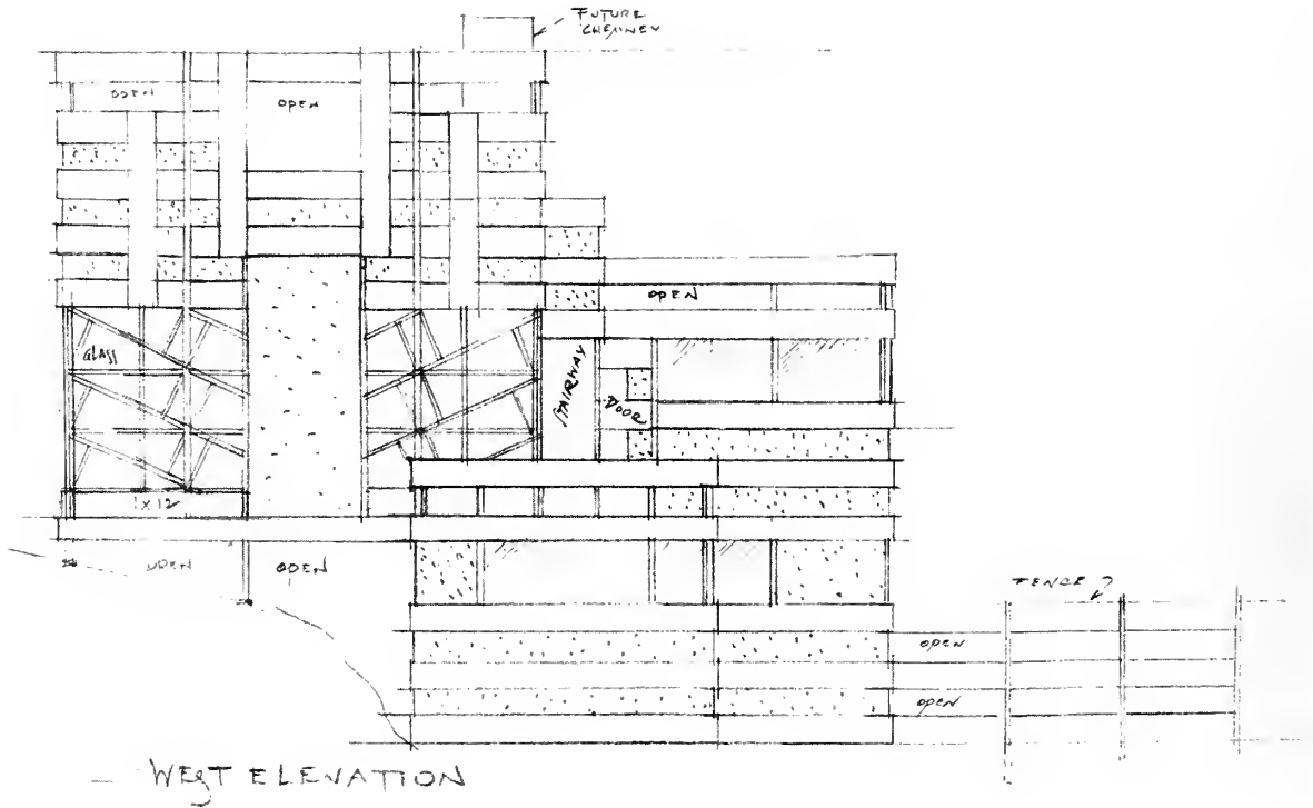
Proj.: Physical Education Club Lodge for Topanga Ranch Topanga Canyon, Los Angeles Co., 1923
