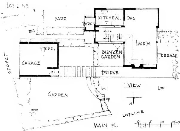
Proj.: First scheme for W. E. Oliver house, Los Angeles, 1931 floor plans
