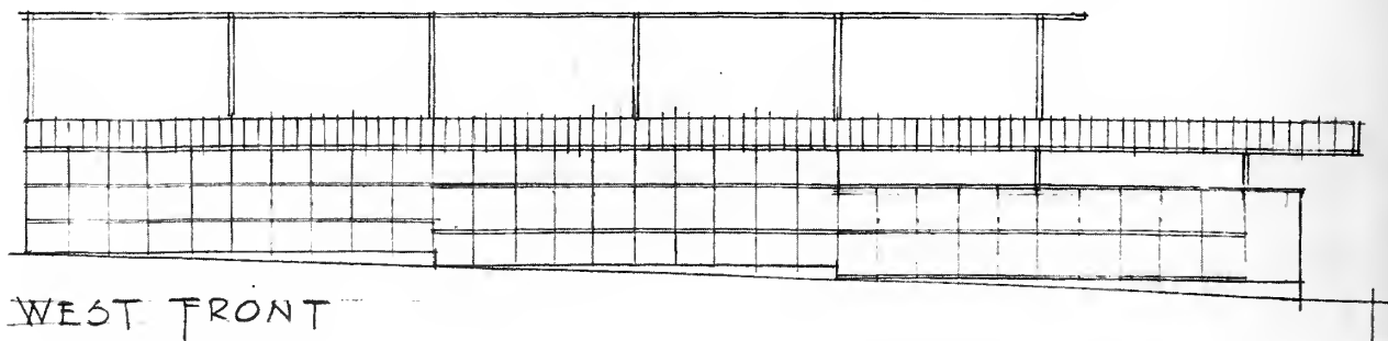
Proj.: Gasoline station for Mrs. Nerenbaum (no location given), 1934
