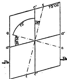
FIG. 8.—Cross section of hornblende crystal parallel to clinopinacoid (parallel to axes a and c in fig. 5), showing positions of crystallographic and elastic axes.
