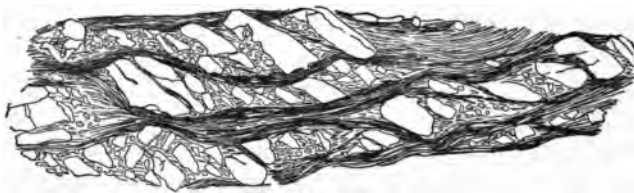
FIG. 17.—“Sliced” feldspars in micaeous and chloritic schist from southern Appalachians.
