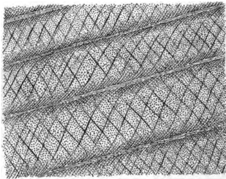
FIG. 37.—Fracture cleavage after fissility in bedded rocks, showing application of principles illustrated in figs. 35 and 36.
