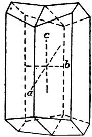
FIG. 12.—Twinned albite crystal with macropinacoidal development.
