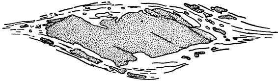
FIG. 9.—Slicing of quartz grain in schistose conglomerate (Metropolitan, Mich., large slide No. 1).
