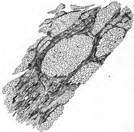
FIG. 27.—Pebbles of quartzite with constituent quartz grains elongated by recrystallization in the plane of elongation of the pebbles and of the rock as a whole. Schistose conglomerate from Metropolitan, Mich. Large slide.
