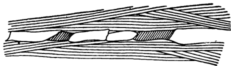
FIG. 4.—Biotite and quartz in a band with parallel muscovite plates adjacent. (Sp. 14901, sl. 7651, Black Hills, South Dakota.)
