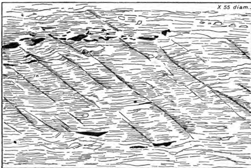
FIG. 40.—Fracture cleavage crossing flow cleavage. After Dale.
