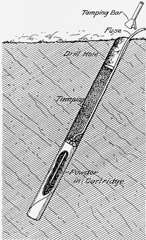
Fig. 48. Method of Charging Drill Hole.
