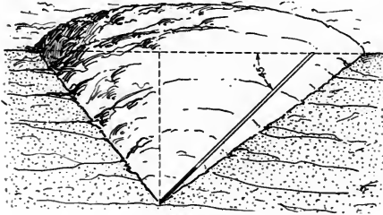
Fig. 2. Inclination of Drill Hole for "Grip" Shot.
