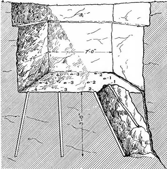
Fig. 15. Drill Holes Near Fissures or Faults.
