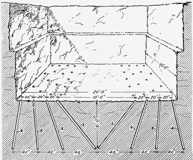
Fig. 10. Arrangement of Drill Holes in Shaft Sinking.
