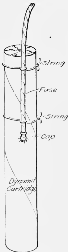
Fig. 59. Fuse Attached to side of Cartridge.
