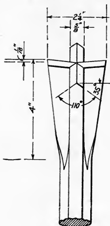
Fig. 23. Drill Steel for Soft Rock.
