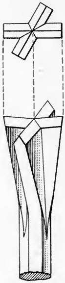
Fig. 26. X Bit Drill Steel
