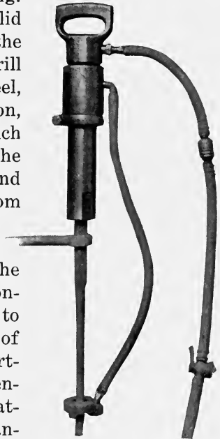
Fig. 35. Hammer Drill.
