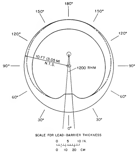
Fig. 5—Schematic diagram showing lead shielding required to attenuate primary, scattered, and leakage radiation to 1 mr/hr at 10 ft. ———, total lead-barrier thickness if leakage radiation from source housing is 0.1 per cent of the primary beam. - - - - -, total lead-barrier thickness if leakage radiation from source housing is 2 mr/hr at 1 meter.
