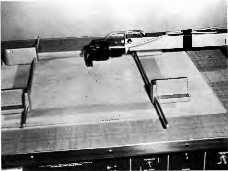
Fig. 21—Automatic isodose plotting device used for scanning X-ray film.
