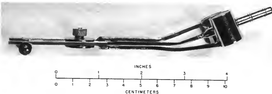
Fig. 2c—Photograph of rigid applicator assembled in lateral projection.
