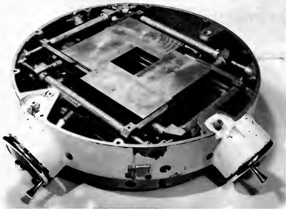
Fig. 8—Cobaltron II diaphragm (model A).
