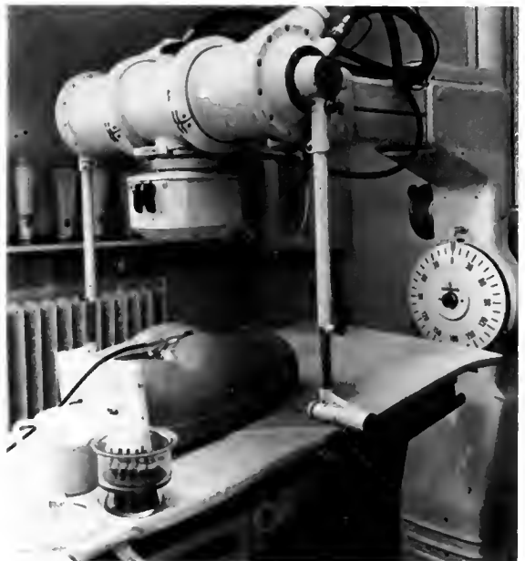
Fig. 2—Heterogeneous phantom containing plasticized skeleton and Lincolnshire bolus.
