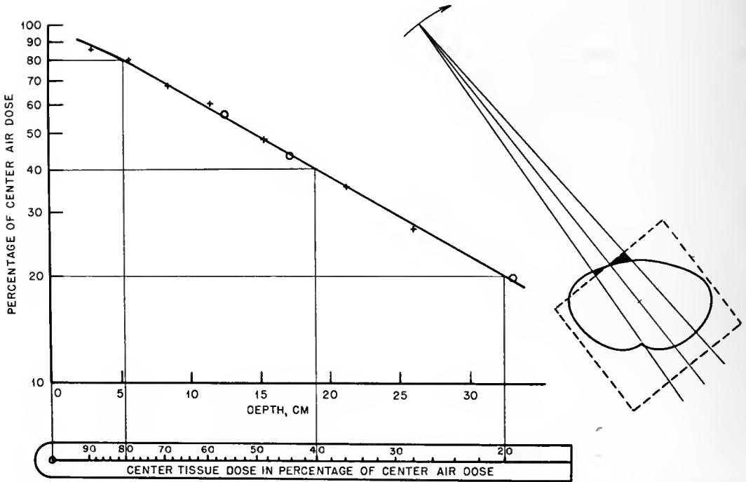
Fig. 2—Relation between center dose and tissue thickness. +, 30- by 30-cm phantom. O, contour phantom. The same absorption is obtained with both phantoms owing to compensating effect of shaded areas. The field was 10 by 10 cm at 75 cm.
