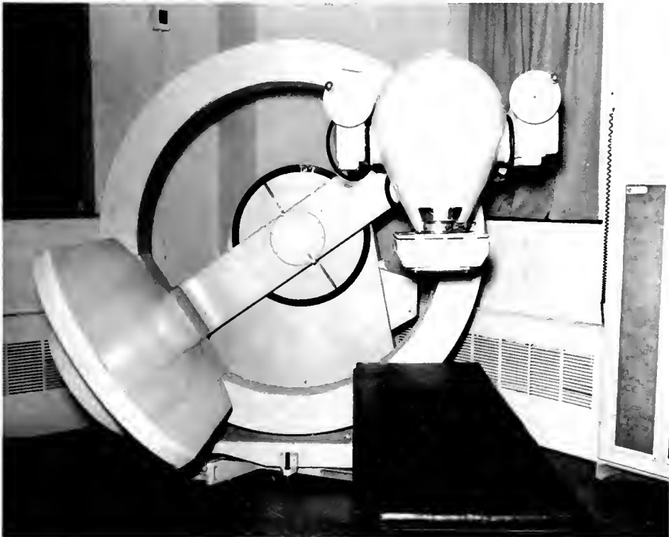
Fig. 9 — The Rotaray showing yoke rotation.
