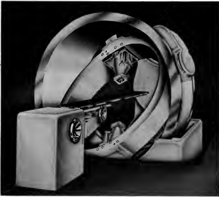
Fig. 4—The Spheray with two source shields.
