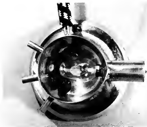
Fig. 1—Vacuum threading device as it appears from the underside. The light source illuminates the threading holes for alignment of the sources before threading. Note the glass elbows in each vacuum line, which allow light transmission.
