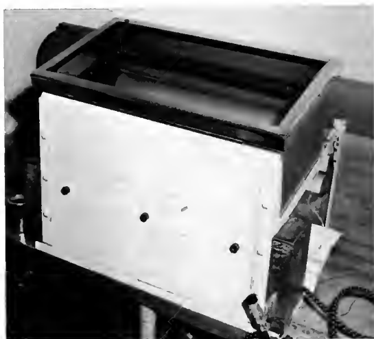
Fig. 6—Zinc bromide viewing tank and associated shielding. Note vacuum control lever in lower right-hand corner.
