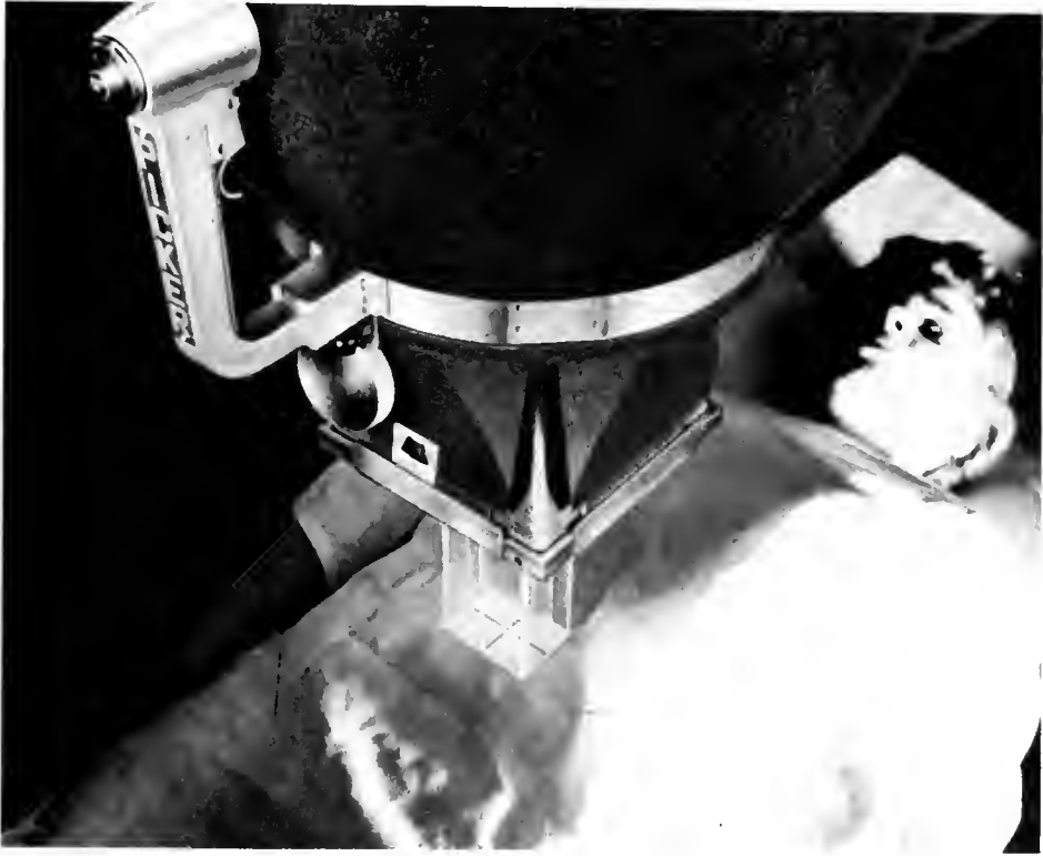
Fig. 6—Collimator with treatment cone of the C-1000 unit.
