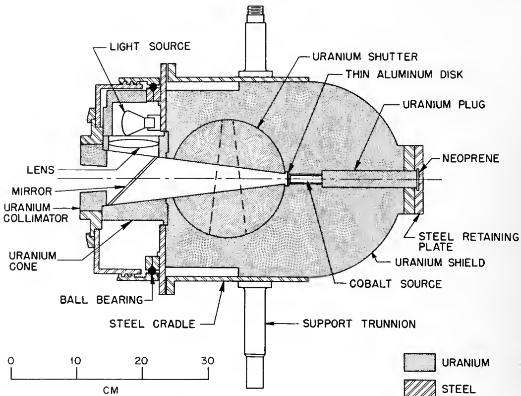
Fig. 1—Kilocurie revolving \text{Co}^{60} unit for radiation therapy, showing some construction details of the uranium housing with a fixed collimator in place. Broken lines show the closed position of the shutter.
