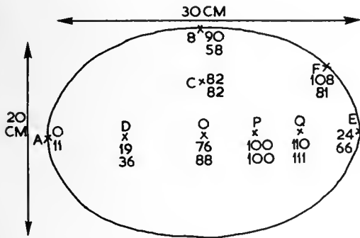
Fig. 6—Diagram showing dosage distribution at certain points in a body section using 250-kv radiation.
