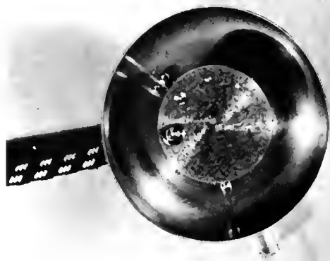
Fig. 2—Vacuum threader as it appears from the top. The circular catch tray prevents spillage of the sources in the course of threading. Note the light illuminating the threading hole.
