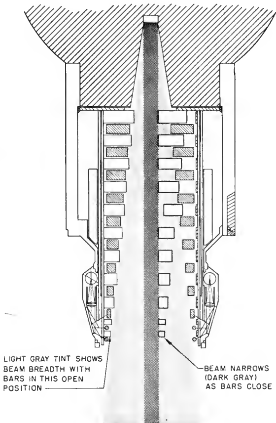
Fig. 3—The Johns-MacKay collimator.
