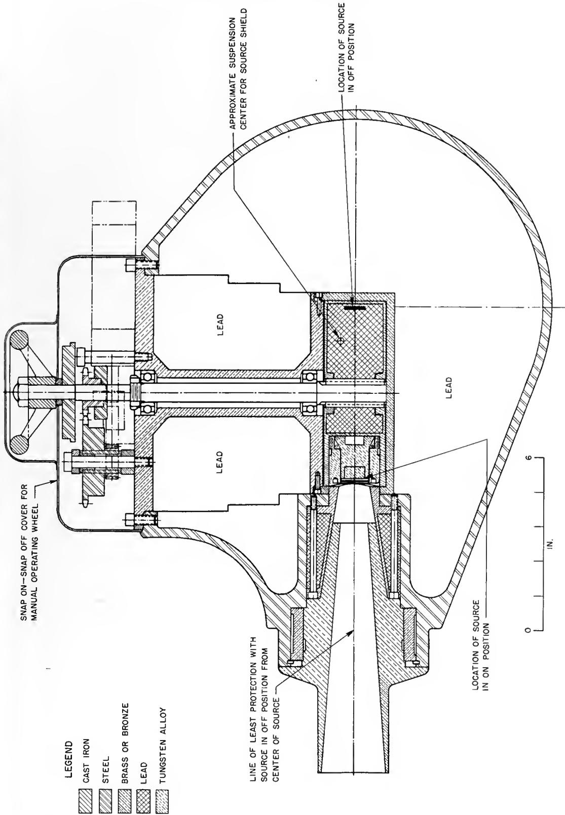
Fig. 3—Cross-sectional diagram of the unit.
