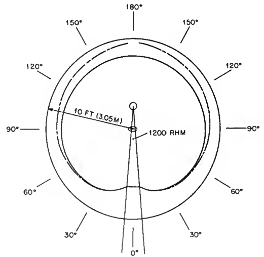
Fig. 4—Schematic diagram showing concrete shielding required to attenuate primary, scattered, and leakage radiation to 1 mr/hr at 10 ft. ———, total concrete-barrier thickness if leakage radiation from source housing is 0.1 per cent of the primary beam. - - - - -, total concrete-barrier thickness if leakage radiation from source housing is 2 mr/hr at 1 meter.
