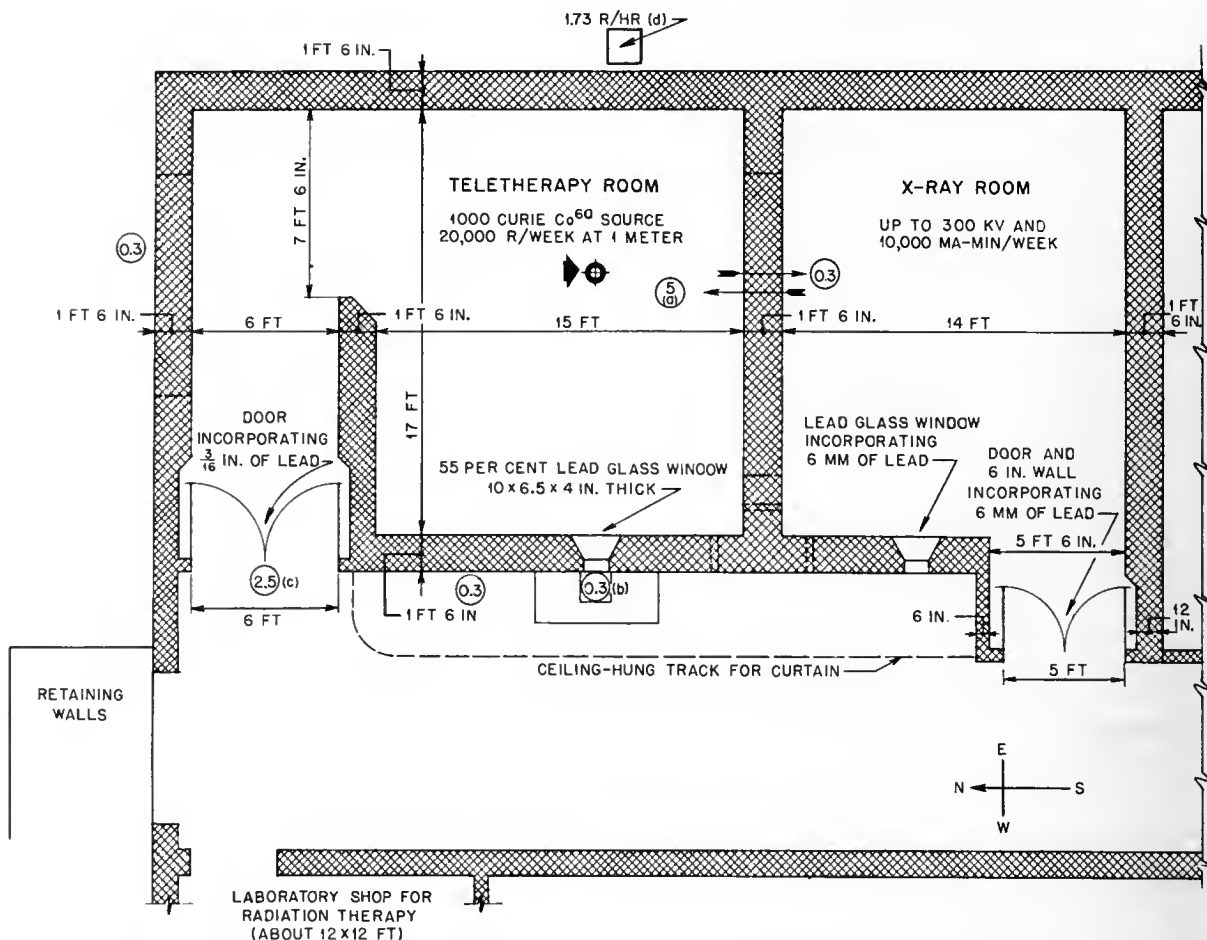
Fig. 2—Tentative plan for radiotherapy rooms at the Syracuse Memorial Hospital. The assumed density of concrete for all walls and roof is 2.35 \text{ g/cm}^3 (147 lb/cu ft). The roof will be 18 in. thick and will be reinforced to support 70 lb/sq ft in addition to the maximum load otherwise considered. There are to be special conduits and provisions for conjoint use of the teletherapy and the X-ray rooms. The ceiling height will be 11 ft.
