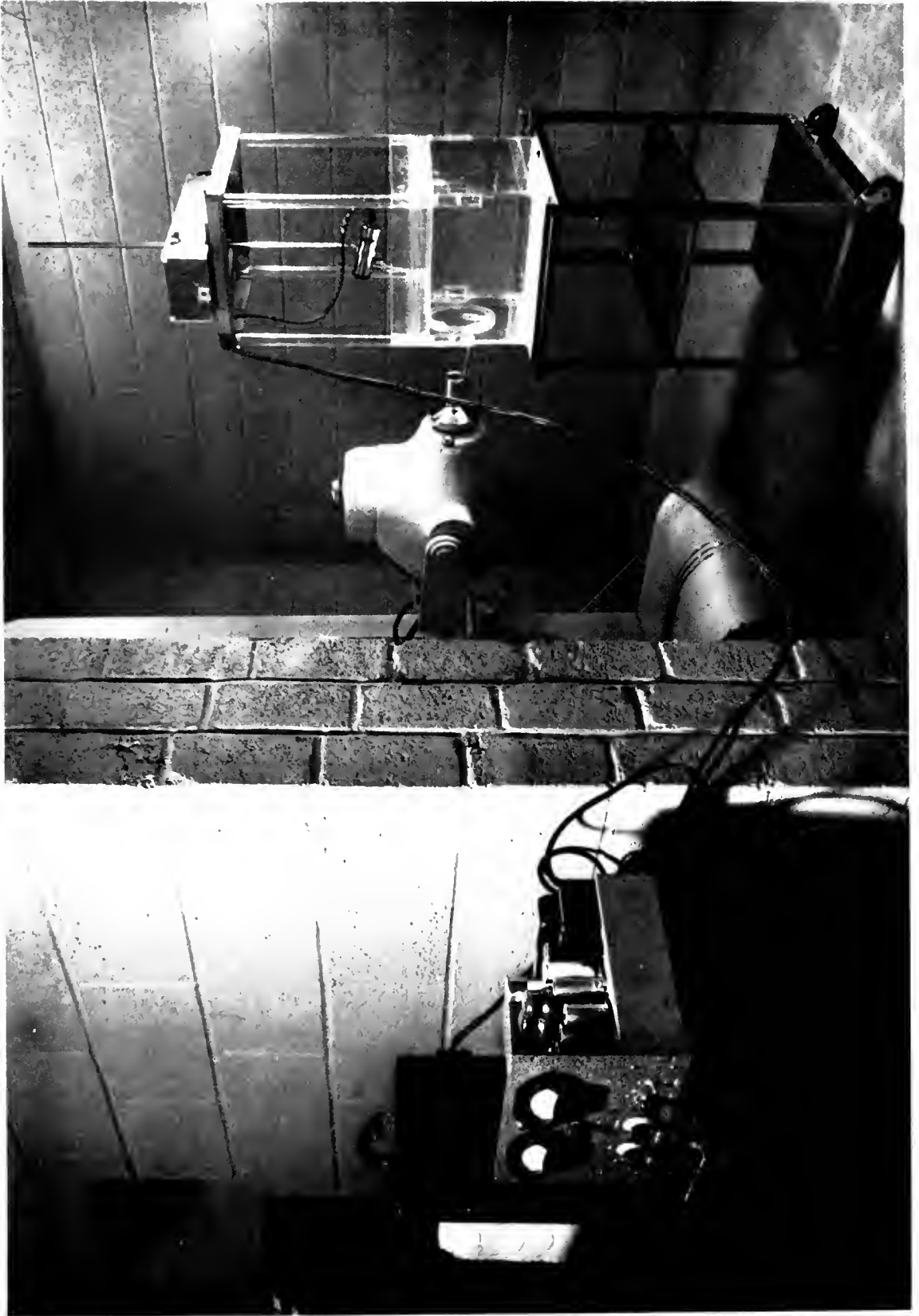
Fig. 2 — Automatic isodose plotter and amplifier with the teletherapy unit.
