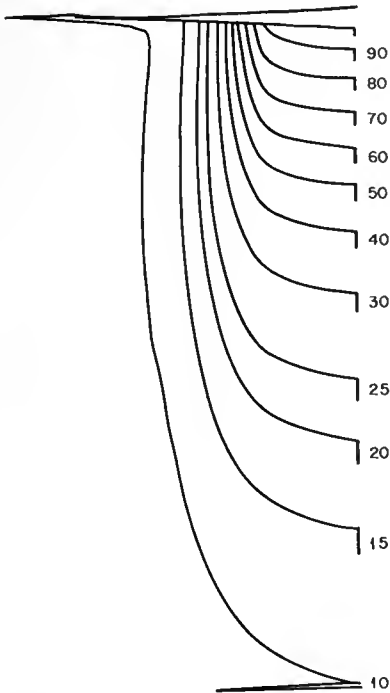
Fig. 4—Source-to-skin distance, 60 cm; source-to-collimator distance, 31.3 cm; collimator-to-skin distance, 28.7 cm; field, 10 cm diameter at 70 cm; aperture, 6.2 cm.
