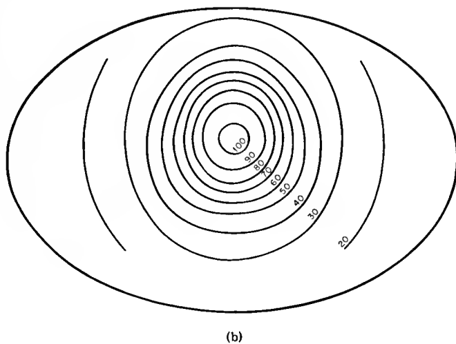
Fig. 7—Calculation of off-axis doses by the method of Braestrup and Mooney. (a) Determination of off-center dose rate, showing the contribution of the radial beam to the dose at points off center. (b) Typical isodose pattern used in the treatment of cancer of the cervix. \text{Co}^{60} therapy; 360-deg rotation.
