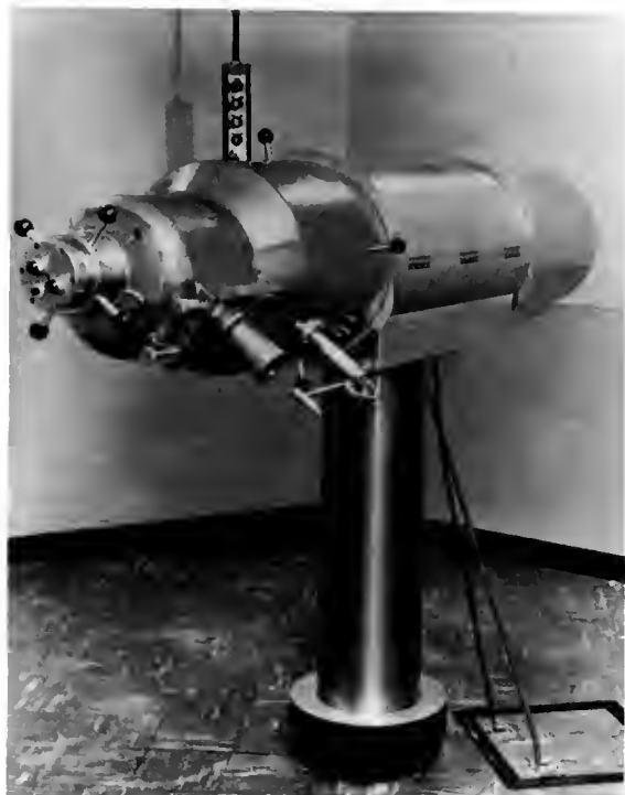
Fig. 2—The City of Hope teletherapy machine mounted on a central pedestal, showing the hydraulic lift mounted in the floor.
