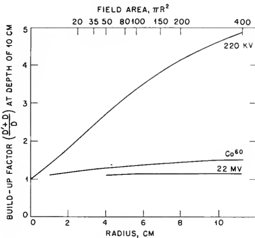
Fig. 4—Rapid increase of build-up factor at low energies and a slower increase at high energies. D', dose due to scattered radiations, D, dose due to primary radiations. For 220 kv, the half-value layer (HVL) is 2 mm of copper, and the FSD is 60 cm. For Co 60 , the FSD is 60 cm. For the 22-Mv betatron, the FSD is 100 cm.
