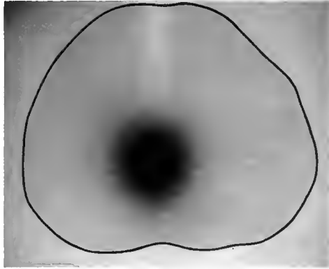
Fig. 17d — Radiograph made with 2-Mv X rays. The film was placed in a phantom reduplicating the patient and rotated 360 deg. The density is proportional to the dose. The lighter streak at the top is the shadow cast by the supporting column on the rotating platform.
