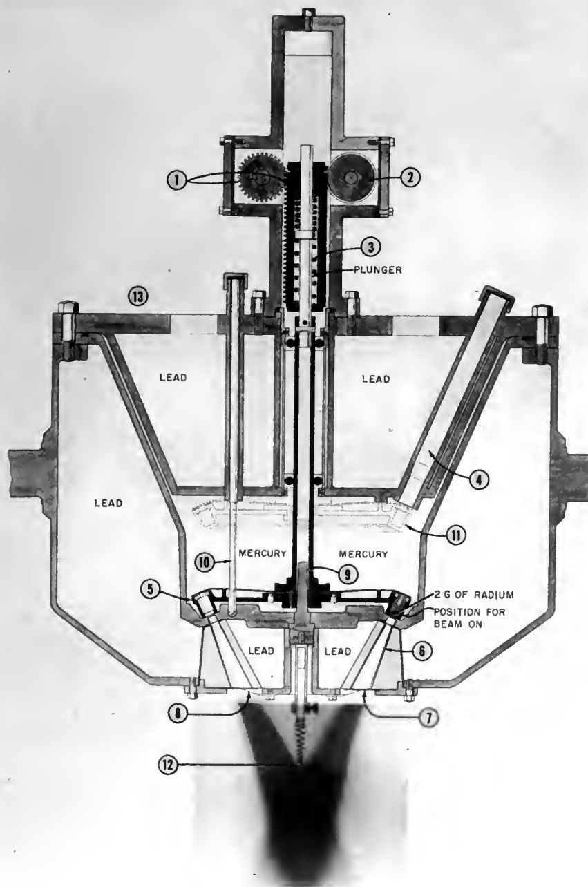
Fig. 4—Diagram of a cross section of the radium-beam head. (1) Rack and pinion for controlling motion of radium-carrying ring up and down; (2) guiding roller; (3) spring compressed to force out mercury at bottom of pool when radium is in treating position; (4) filling hole through which radium was inserted in Belgium; (5) treating position of radium-carrying ring, showing position and angulation of radium capsule; (6) conical collimating channel through lead; (7) brass beta-ray filter covering bottom of beam head; (8) removable graded brass filter to reduce central high point of radiation; (9) cone for centering radium-carrying ring; (10) guide rod to prevent rotation of ring; (11) off or safe position of ring at top of mercury pool; (12) central pointer along which radium-to-skin distance is measured; (13) location of machinery on top of beam head, concealed by cover.
