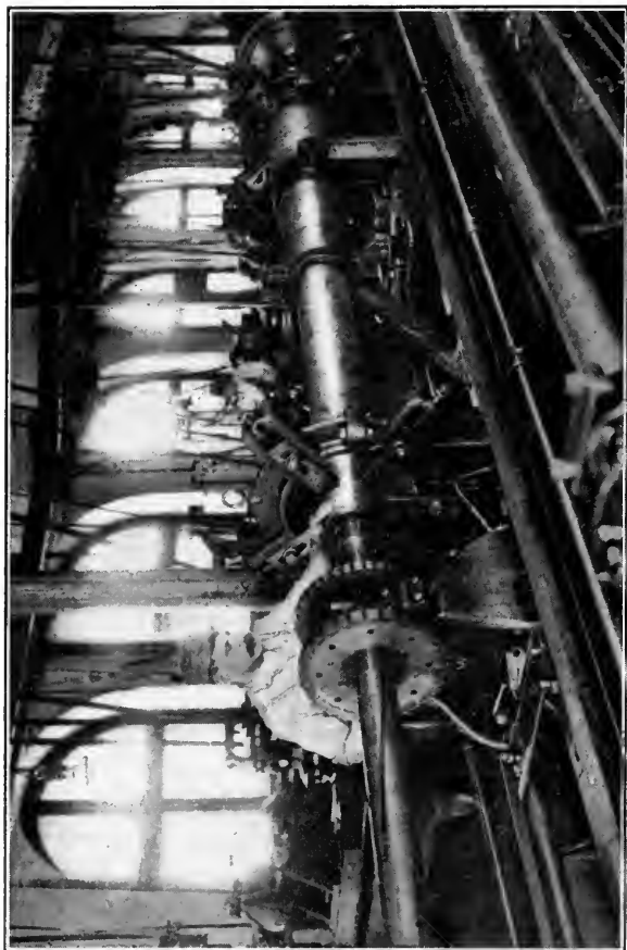
Rifling a Gun.
