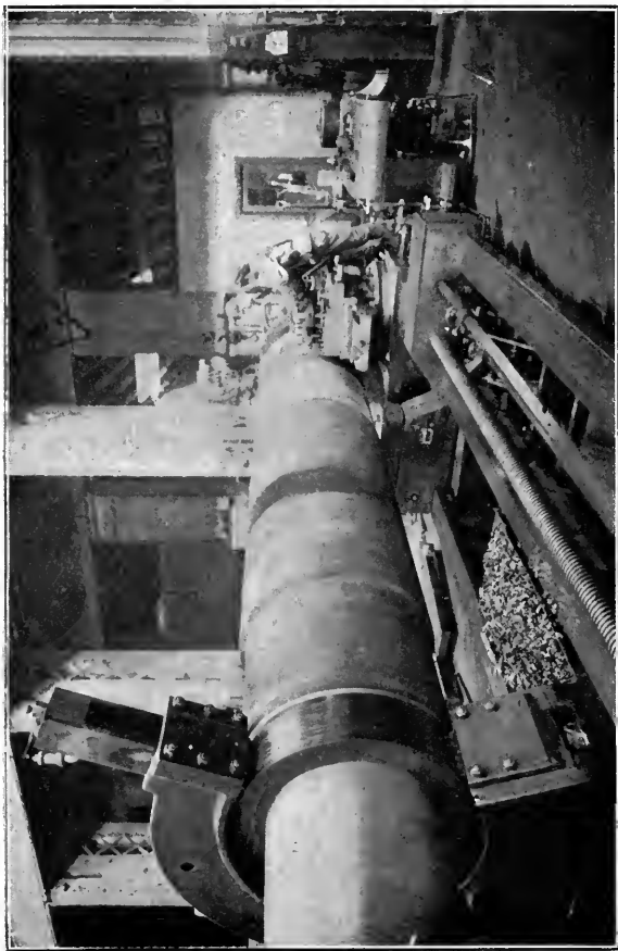
Cutting down a Jacketed Gun.
