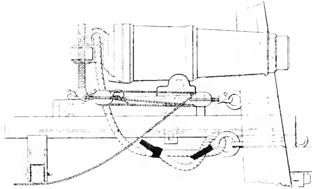
A 24-PR. CARRONADE, ca. 1820.
