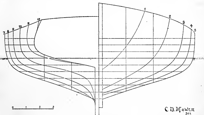
Body-plan of the Spray .
