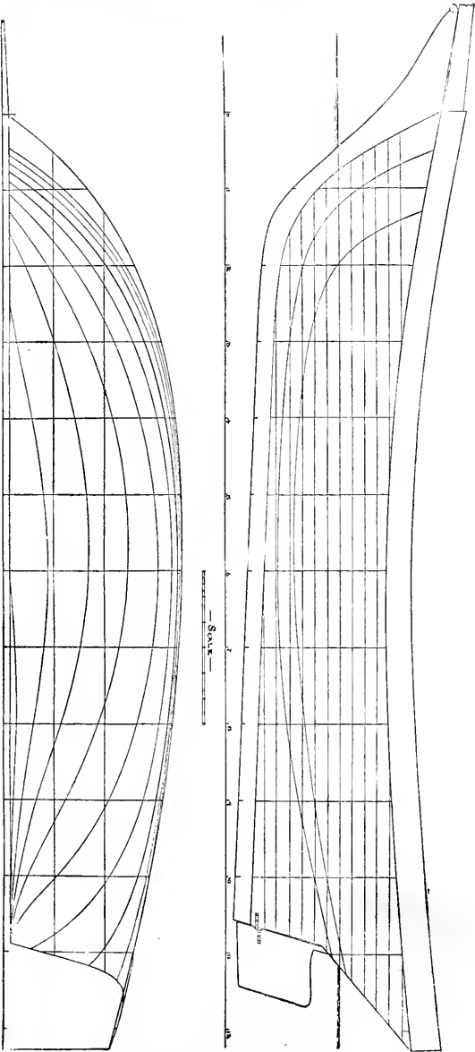
Lines of the Spray.
