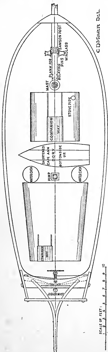
Deck-plan of the Spray .
