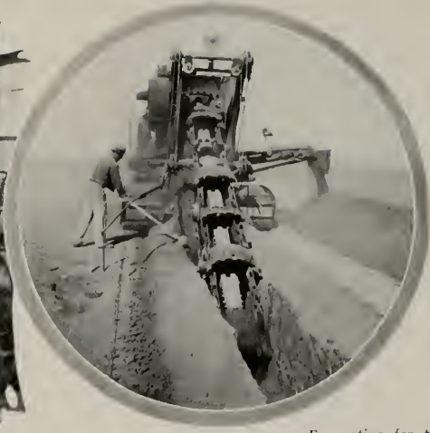
Excavating for pipe line
