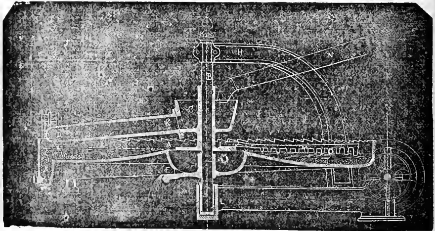
Sectional View of Hendy's Patent Ore Concentrator.
