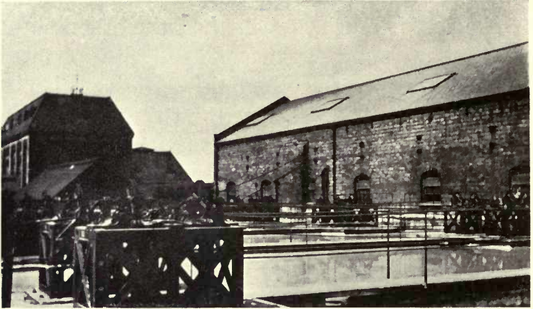
CROSSNESS, LONDON, ENGLAND Chemical precipitation sewage treatment plant
