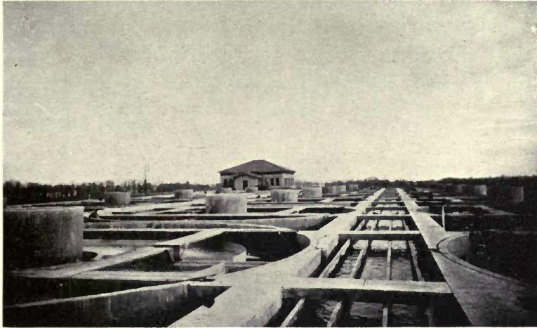
BALTIMORE, MARYLAND Imhoff tank sewage treatment plant
