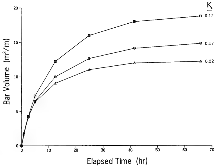
Figure 64. Effect of \kappa on bar volume
