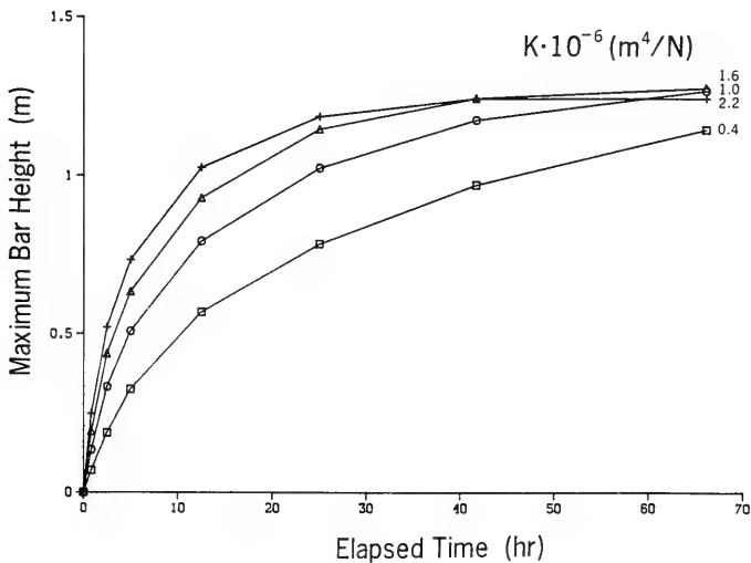
Figure 62. Effect of K on maximum bar height
