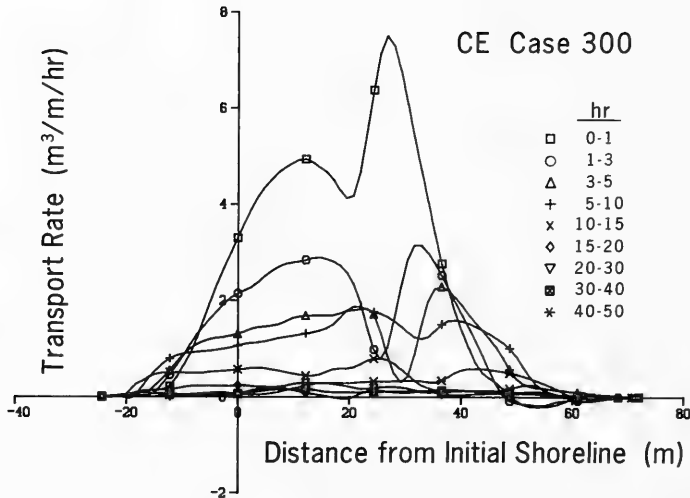
Figure 33. Calculated distributions of the net cross-shore sand transport rate for an erosional case (Case 300)
