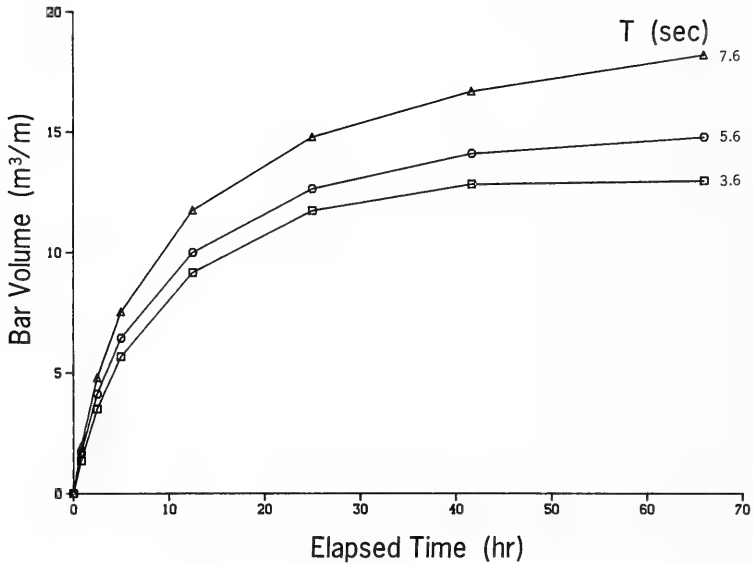
Figure 68. Effect of T on bar volume
