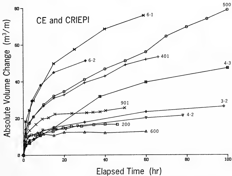
Figure 5. Absolute sum of profile change for selected cases
