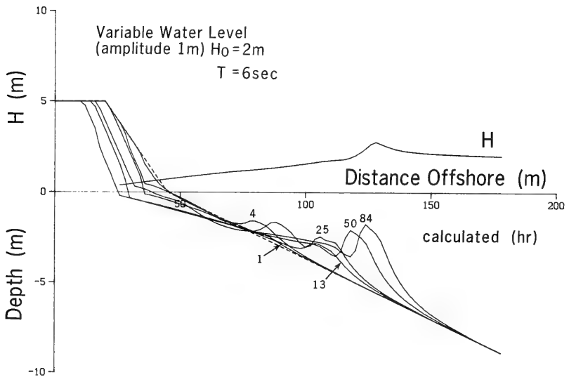
Figure 72. Simulation with varying water level
