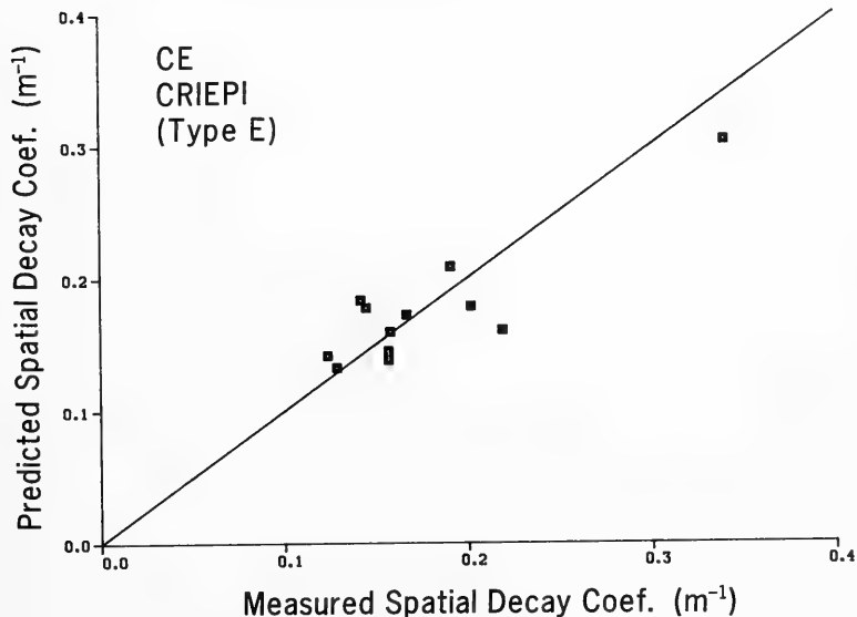
Figure 46. Comparison of spatial decay rate coefficients and an empirical predictive expression
