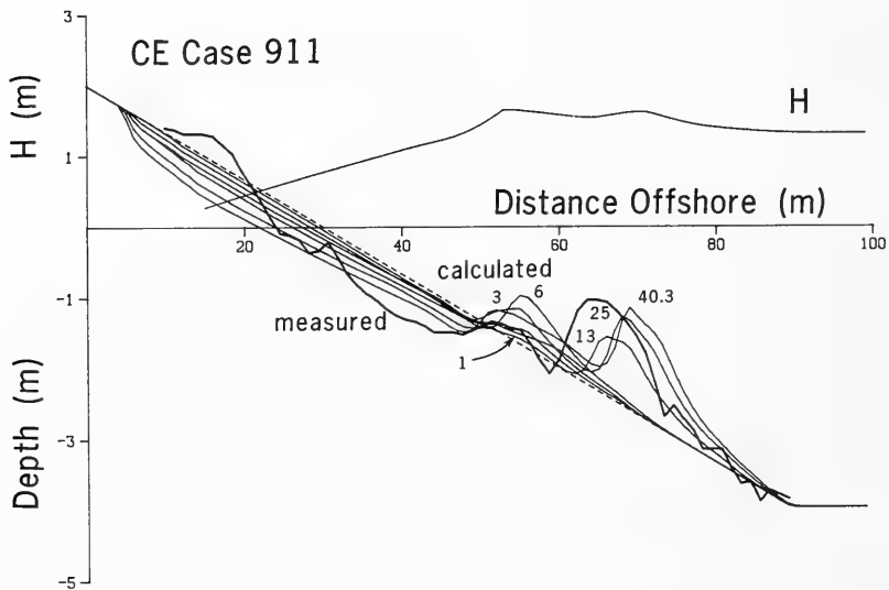
Figure 70. Verification for case of varying water level
