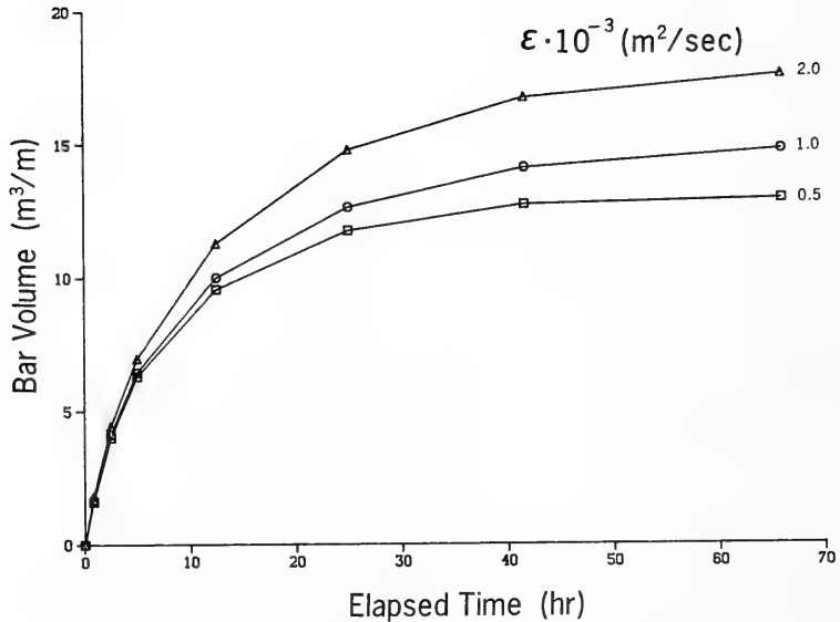
Figure 63. Effect of \epsilon on bar volume
