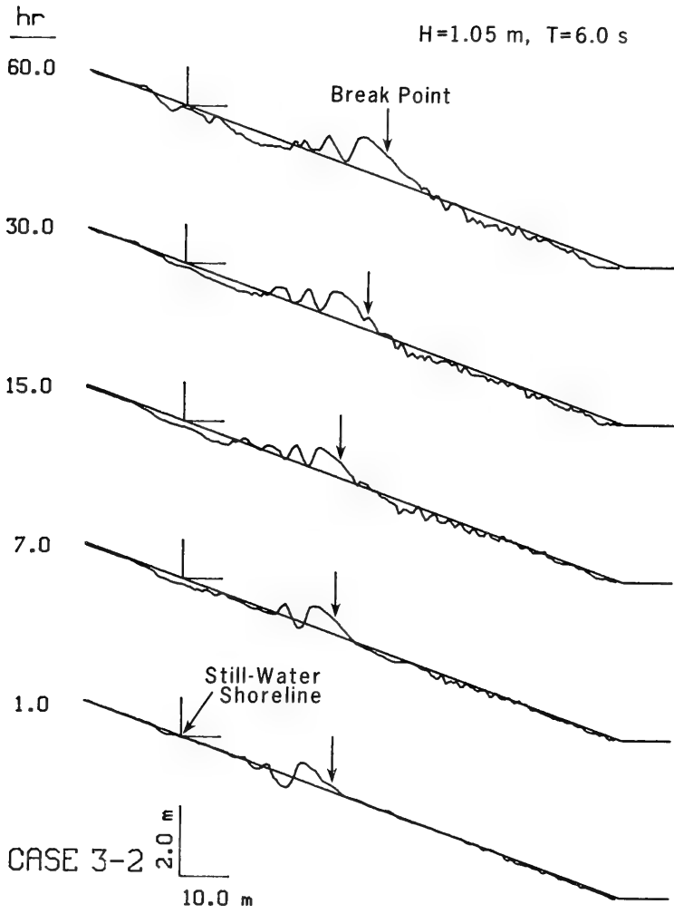
Figure 37. Evolution of beach profile under constant incident wave conditions for a mixed accretionary and erosional case (Case 3-2)
