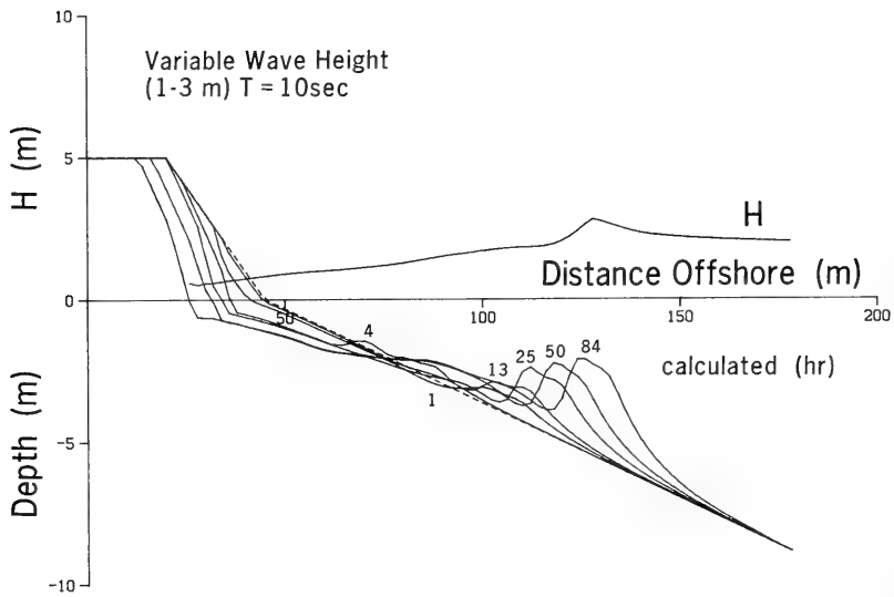
Figure 73. Effect of varying wave height
