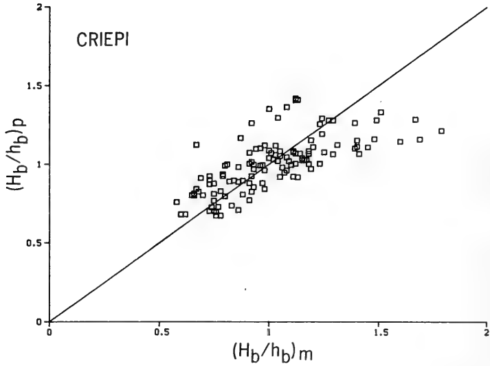
Figure 53. Comparison between measured and predicted breaker ratio
