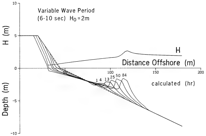
Figure 71. Simulation with varying wave period
