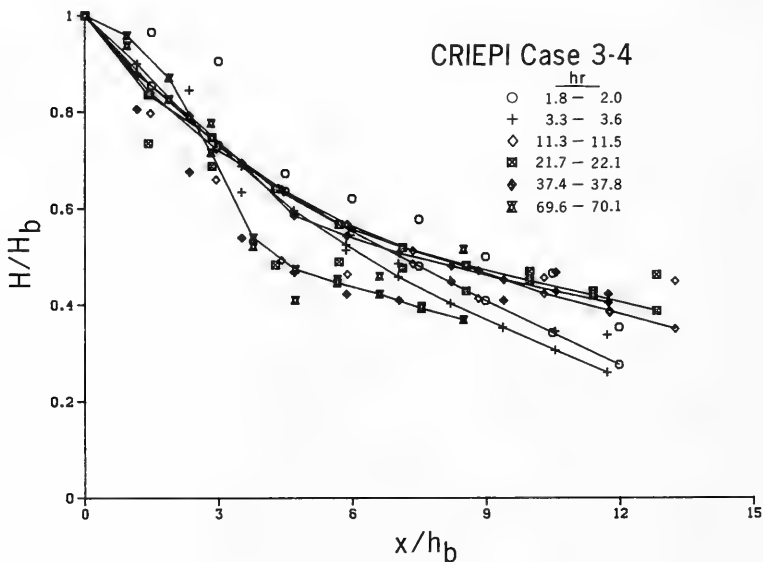
Figure 55. Measured and calculated wave heights
