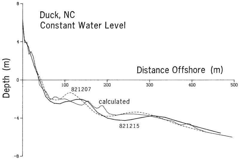
Figure 80. Field verification omitting water level variation
