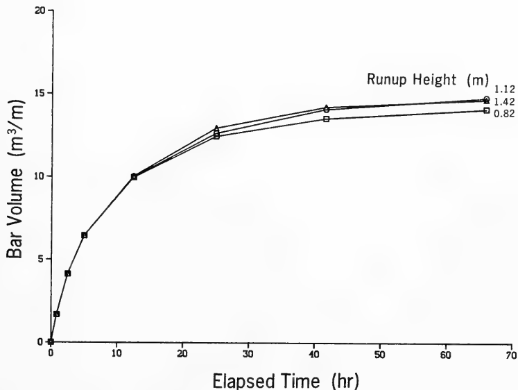
Figure 69. Effect of runup height on bar volume
