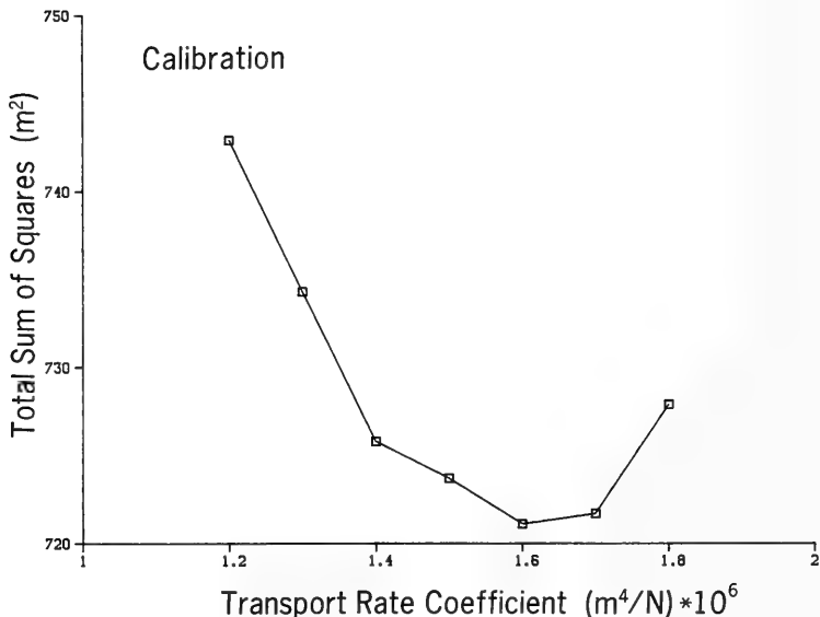
Figure 59. Optimization for model calibration
