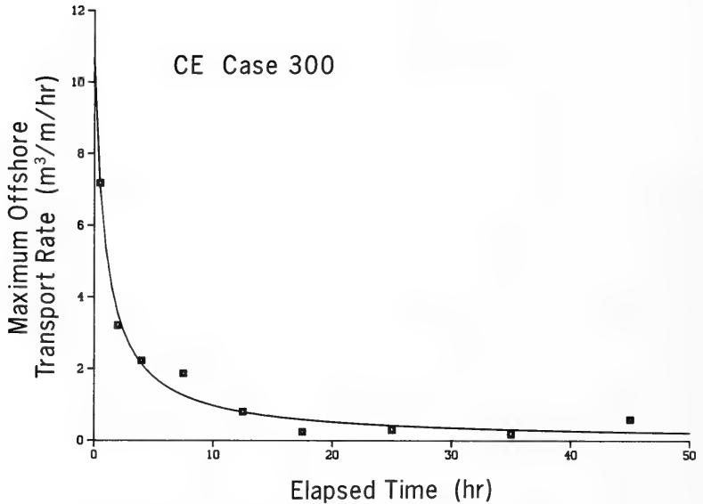
Figure 40. Decay of peak offshore sand transport rate and a best-fit empirical predictive expression
