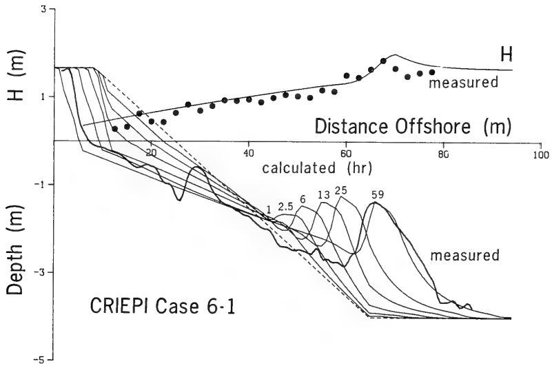
Figure 57. Calibration of numerical model
