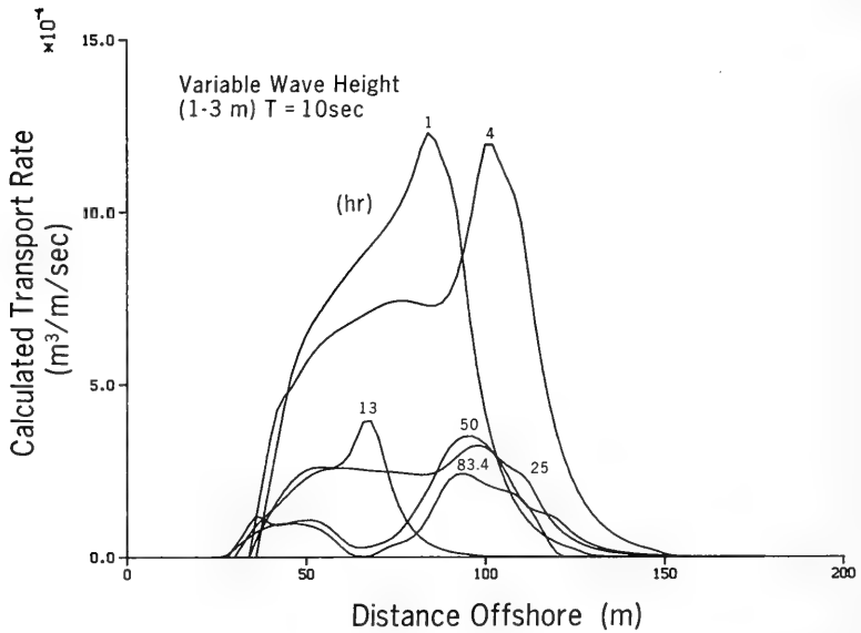
Figure 74. Transport rate distributions for varying wave height
