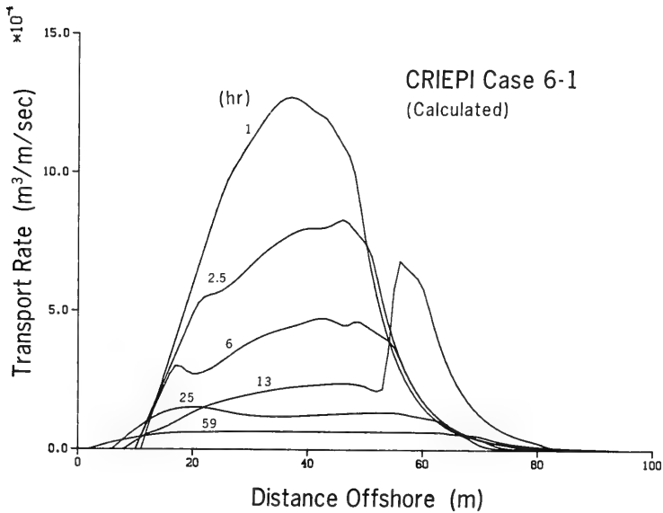
Figure 58. Net cross-shore transport rates at selected times
