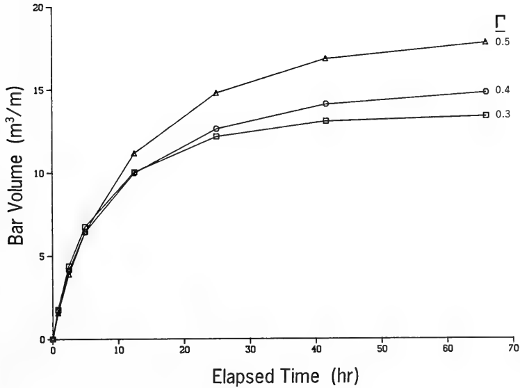
Figure 65. Effect of \Gamma on bar volume
