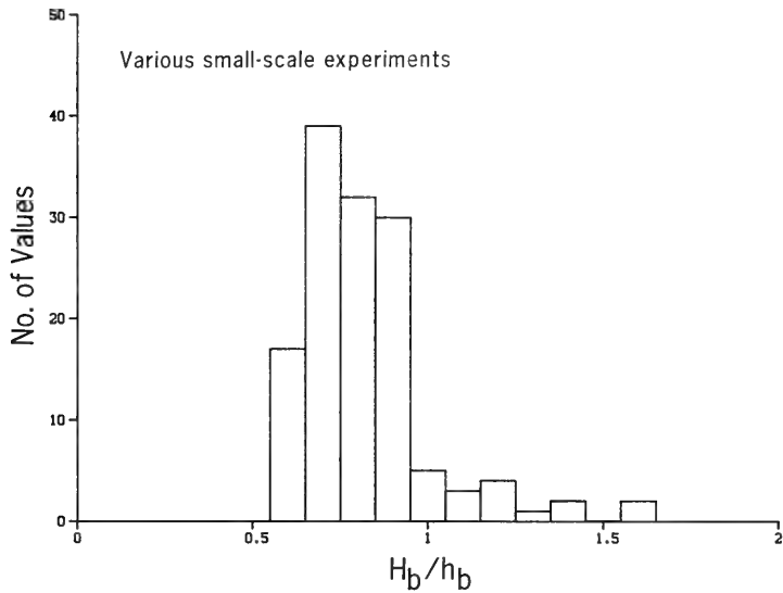
Figure 52. Distribution of breaker ratio for small-scale laboratory data
