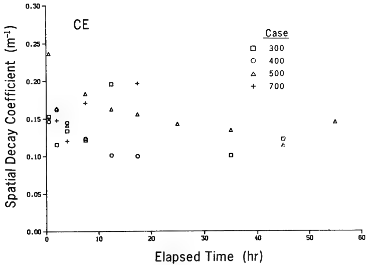
Figure 44. Spatial decay rate coefficient seaward of the break point
