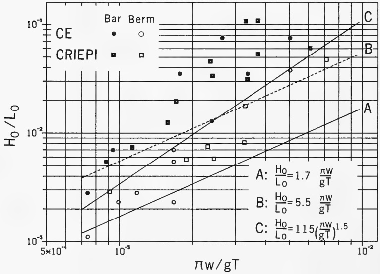
Figure 8. Criterion for distinguishing profile type by use of wave steepness and Dean parameter
