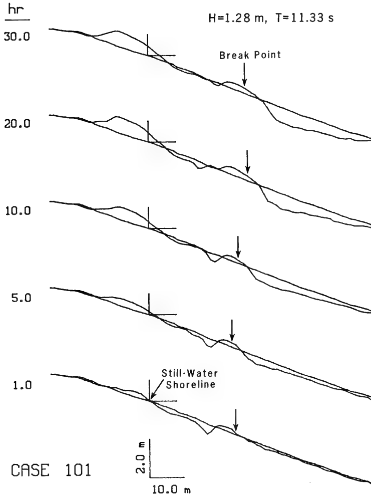
Figure 34. Evolution of beach profile under constant incident waves for an accretory case (Case 101)
