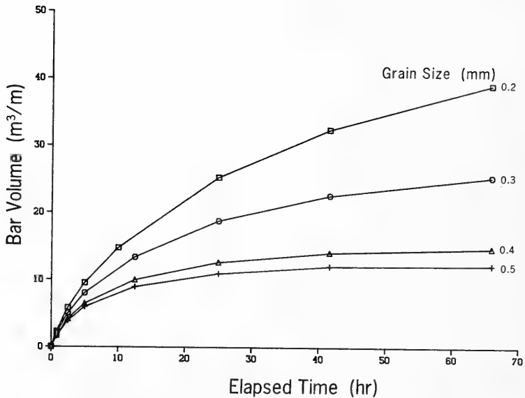
Figure 66. Effect of D on bar volume
