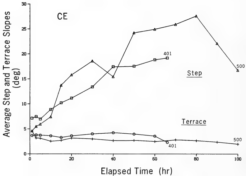
Figure 27. Evolution of representative step and terrace slopes
