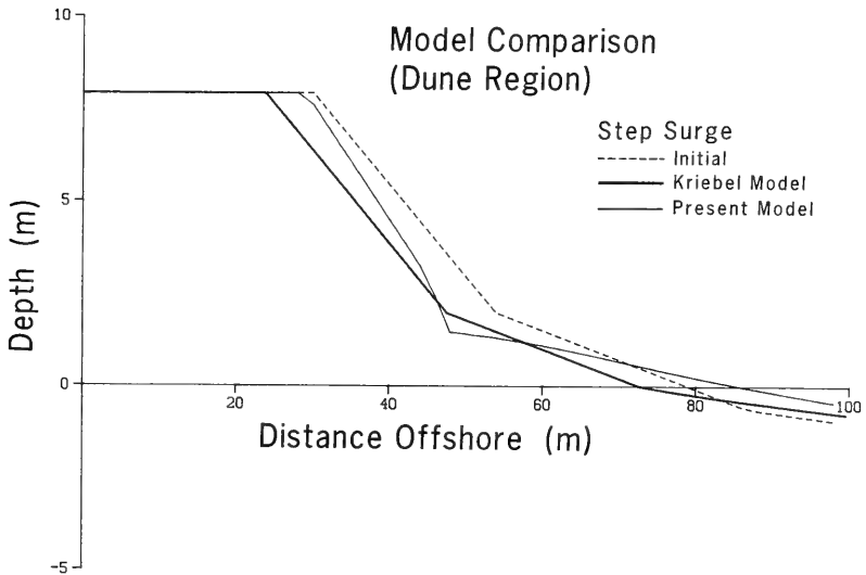
b. Details of dune region
