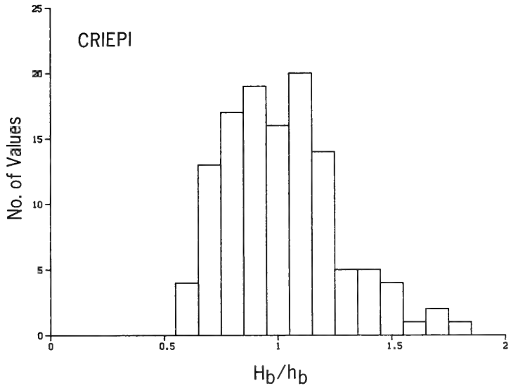
Figure 51. Distribution of breaker ratio for the CRIEPI data
