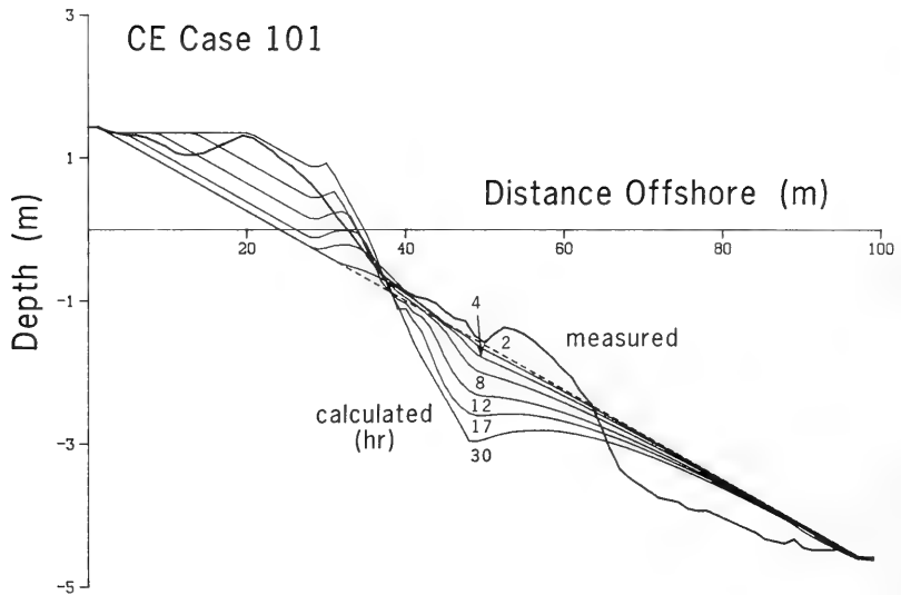
Figure 84. Simulation of berm formation and growth
