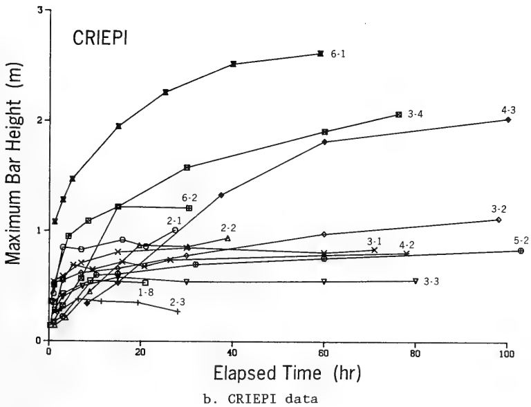
Figure 20. Evolution of maximum bar height
