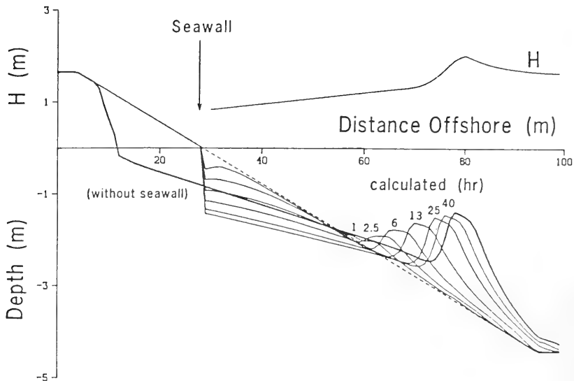
Figure 85. Simulation with and without seawall
