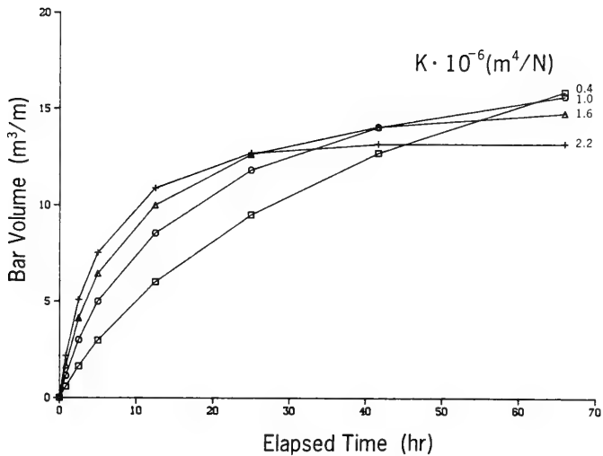
Figure 61. Effect of K on bar volume
