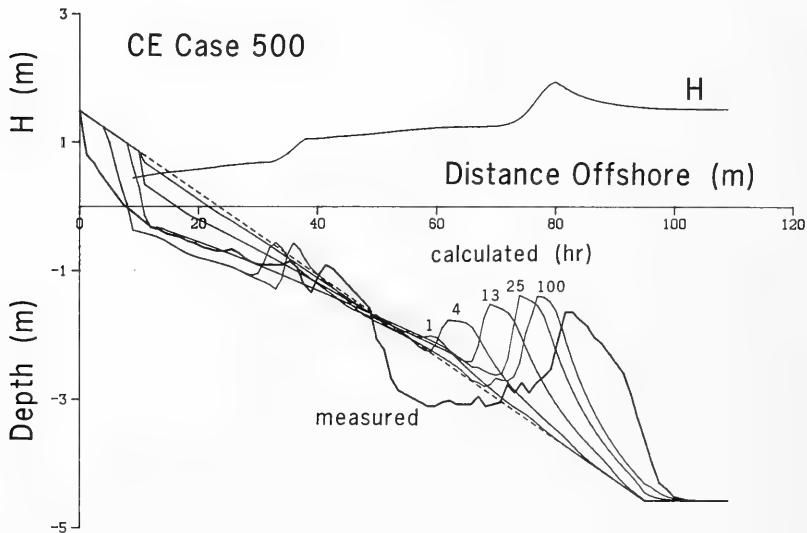
Figure 76. Reproduction of the second breakpoint bar
