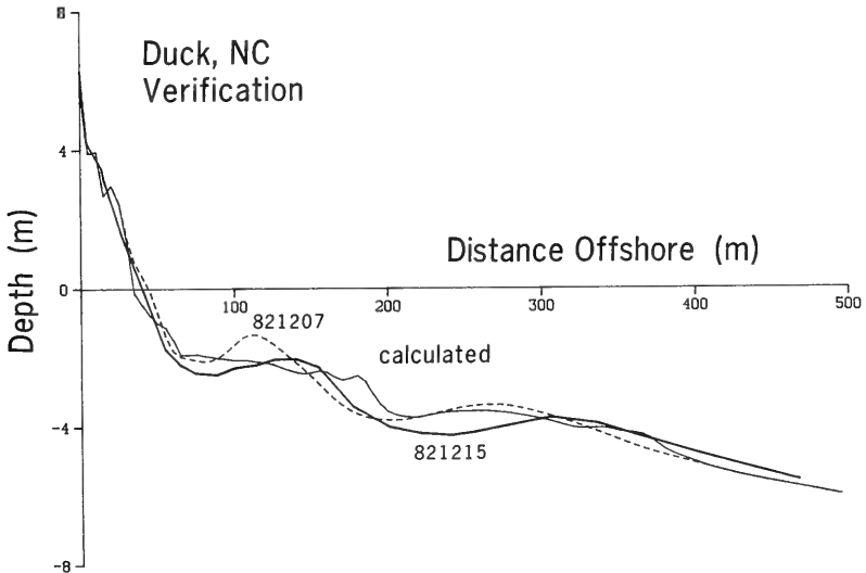
b. Result of simulation
