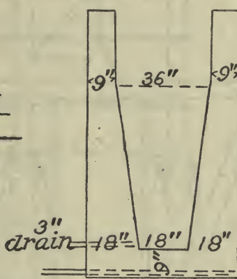
FIG. 10.—Showing a transverse section of swimming vat built of concrete or brick and cement.
