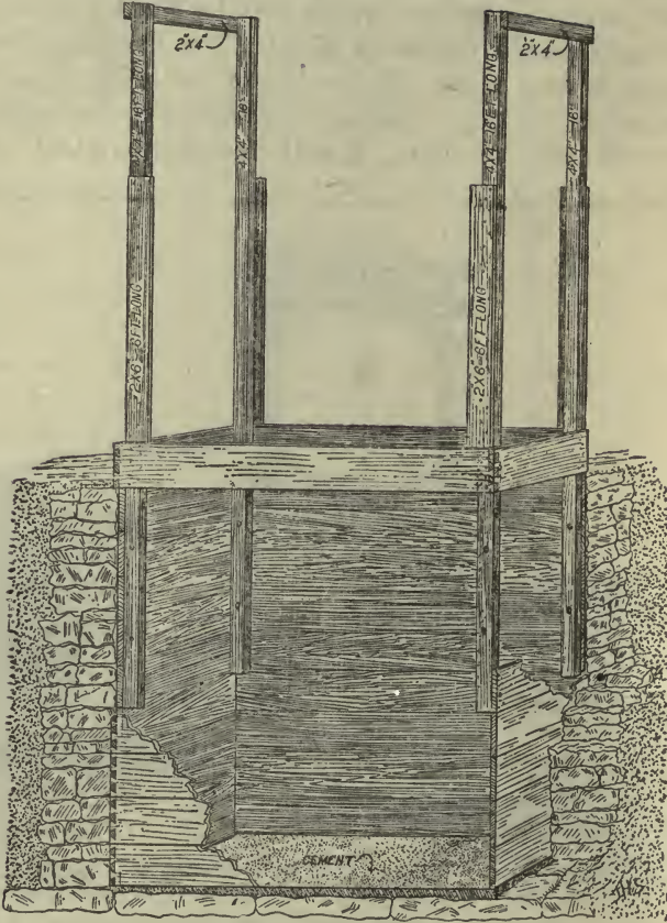
FIG. 2. —Vat. Tank 10 ft. deep, 4 ft. wide, 9 ft. in ground. Should contain from 5½ to 6 ft. of dip. Standards 4 by 4 in. by 16 ft. long, bolted to tank inside, to extend 6 ft. inside of tank, to act as guides to cage; 2 by 6 in. plank 6 ft. long nailed to outside of standards; 2 by 4 or 2 by 6 in. braces across top of standards. The tank should be built of 2-in. plank and joined with a tongue, the ends of the tank mortised in, the joints coated with lead. The braces are 4 by 4 in. The tank, being placed in the ground and packed solid, does not require much bracing. The tank should be laid in cement bottom, with stone and mortar about sides.
